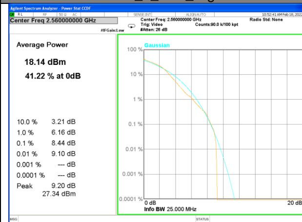
Band 7_1_Q16_High
