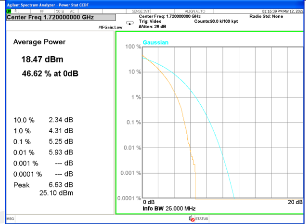
Band 66_100_Q16_Low
