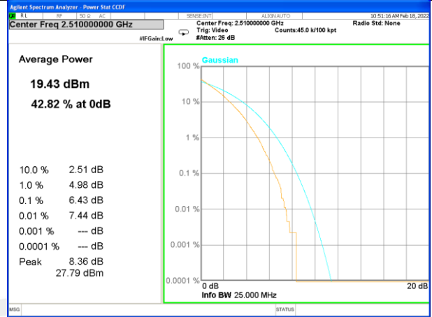
Band 7_100_Q16_Low
