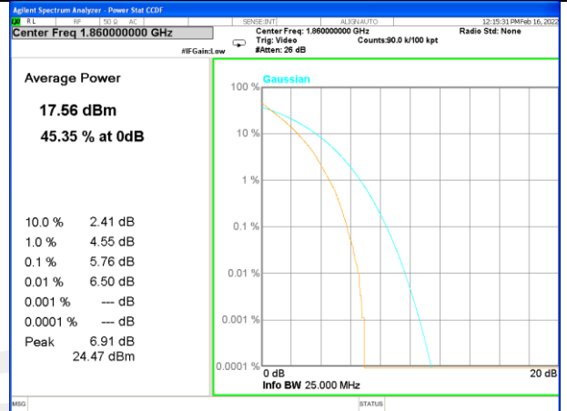
Band 2_100_Q16_Low
