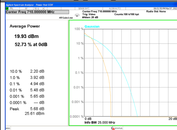
Band 17_1_QPSK_Middle
