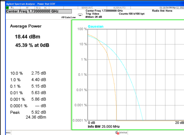
Band 66_1_QPSK_Middle
