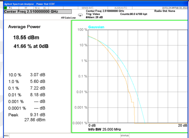
Band 7_100_QPSK_Middle
