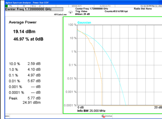
Band 66_1_Q16_Low
