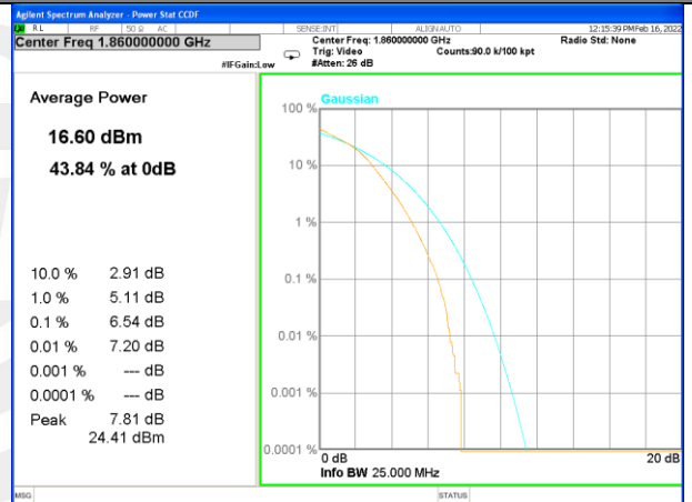
Band 2_100_QPSK_Middle
