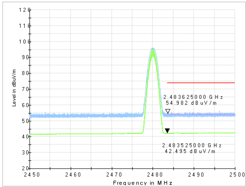
Fig.4. Frequency Band Edges: GFSK, 2480 MHz, Hopping Off , 2.45 GHz - 2.50GHz
