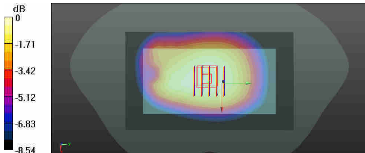
0 dB = 0.483 W/kg
