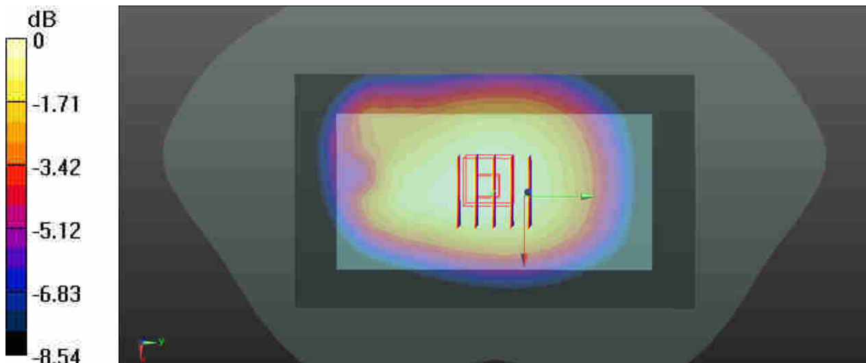
0 dB = 0.483 W/kg
