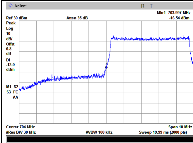
LTE Band XVII - Low Channel QPSK-5
