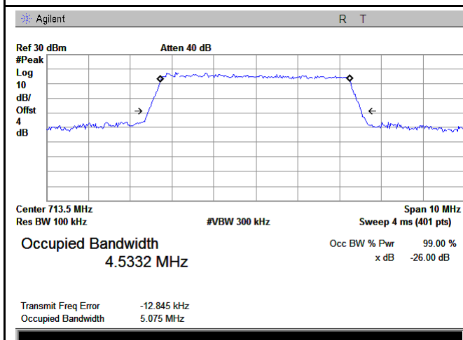
LTE Band XVII - High CH QPSK-5
