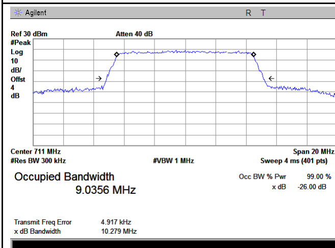
LTE Band XII - High CH QPSK-10
