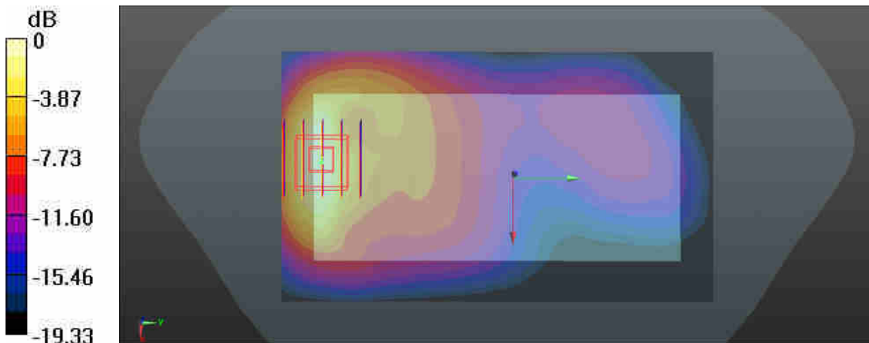
0 dB = 0.719 W/kg
