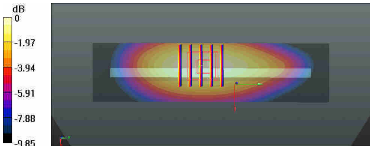
0 dB = 0.296 W/kg
