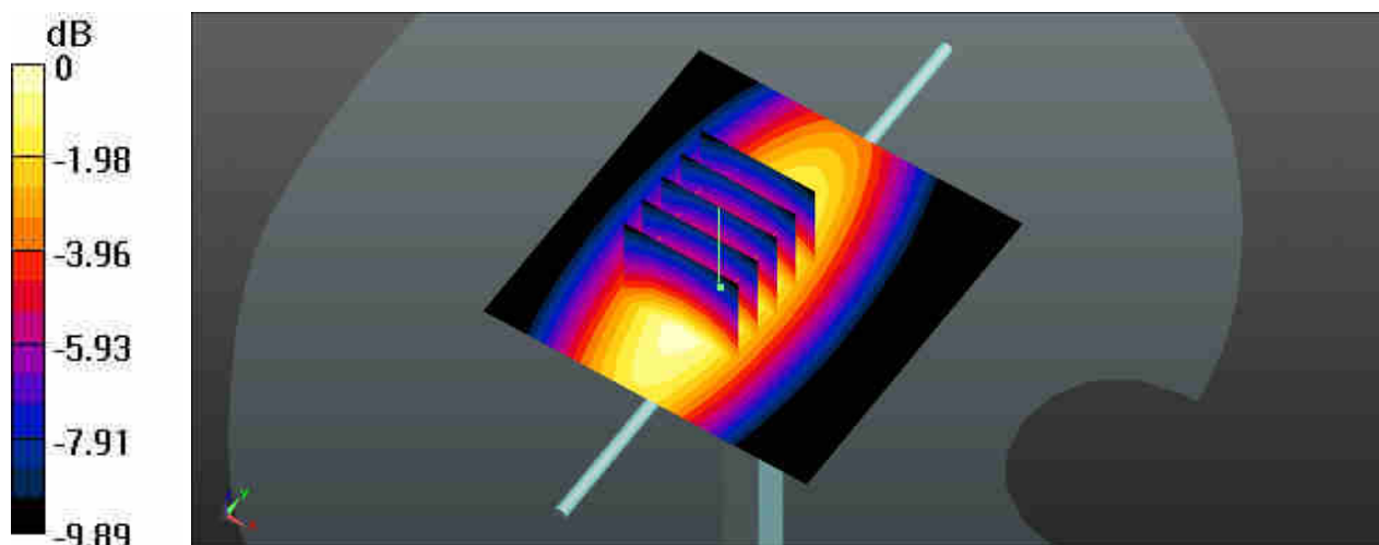
0 dB = 2.61 W/kg
