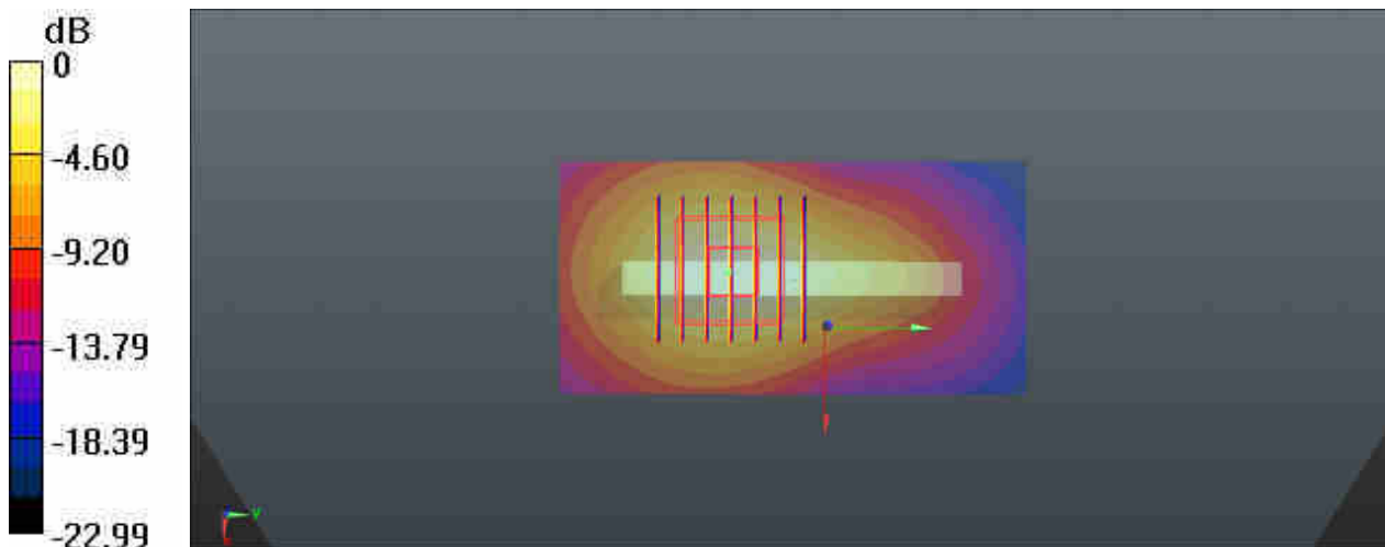
0 dB = 0.344 W/kg
