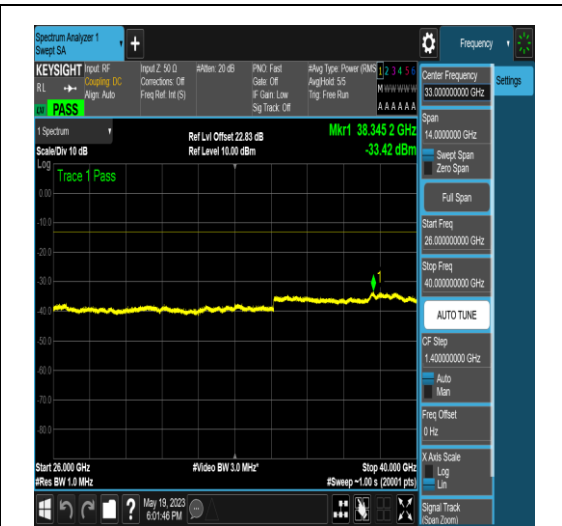
NTNV_N77-3700-3980_PC2_30_60_M_TID18_N S_01_26000_40000_#1
