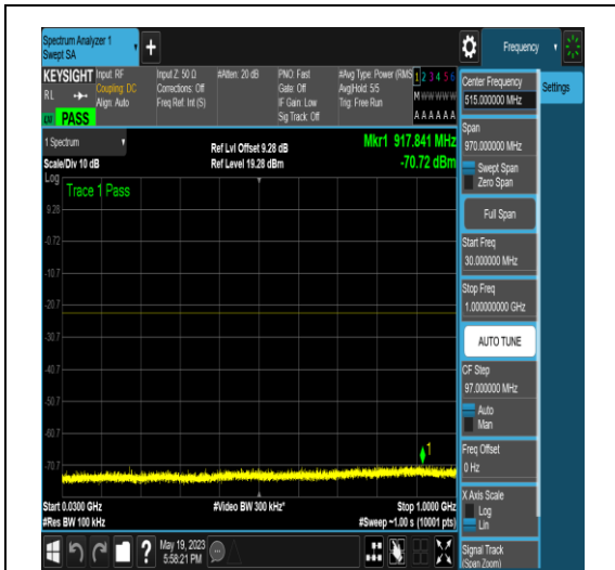
NTNV_N77-3700-3980_PC2_30_60_M_TID5_NS _01_30_1000_#1
