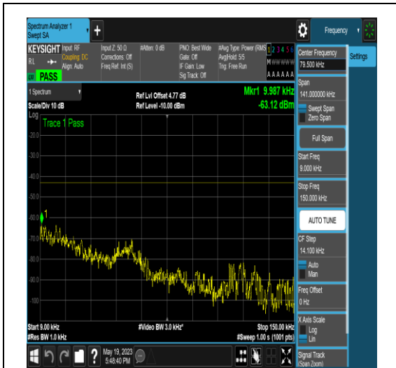
NTNV_N77-3700-3980_PC2_30_60_L_TID16_NS _01_0.009_0.15_#1
