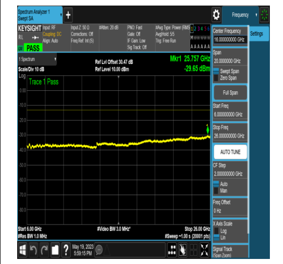
NTNV_N77-3700-3980_PC2_30_60_M_TID5_NS _01_6000_26000_#1
