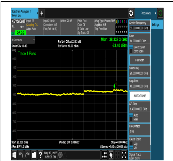
NTNV_N77-3700-3980_PC2_30_60_M_TID6_NS_01_26000_40000_#1
