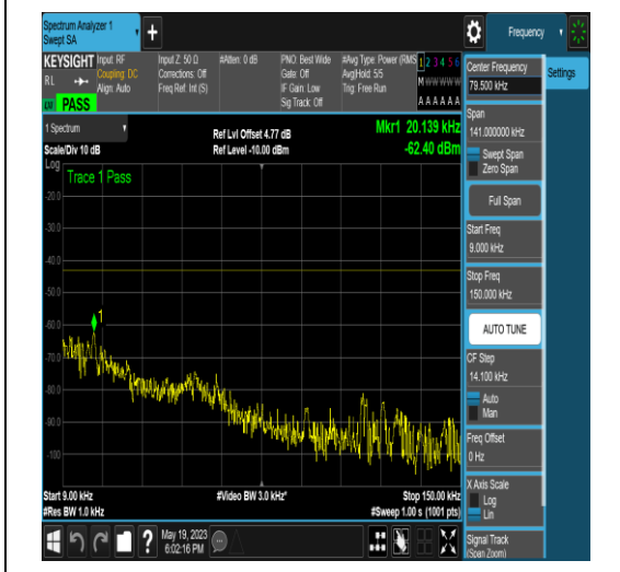
NTNV_N77-3700-3980_PC2_30_60_M_TID16_N S_01_0.009_0.15_#1
