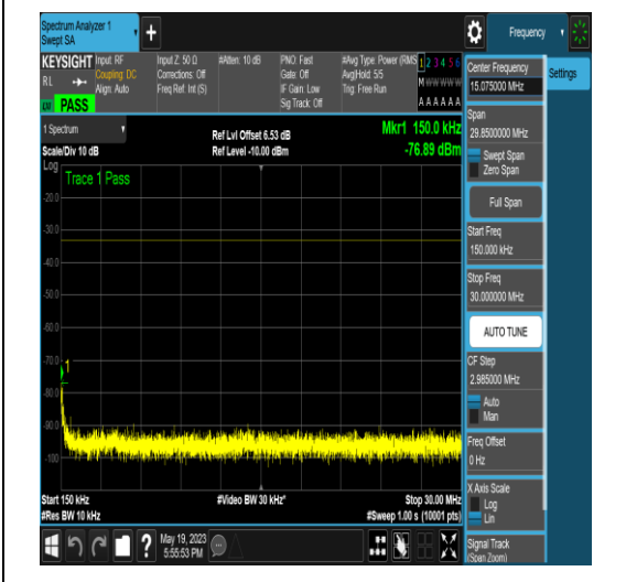
NTNV_N77-3700-3980_PC2_30_60_M_TID4_NS_01_0.15_30_#1
