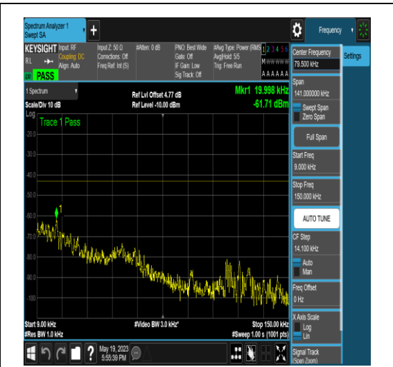
NTNV_N77-3700-3980_PC2_30_60_M_TID4_NS_01_0.009_0.15_#1
