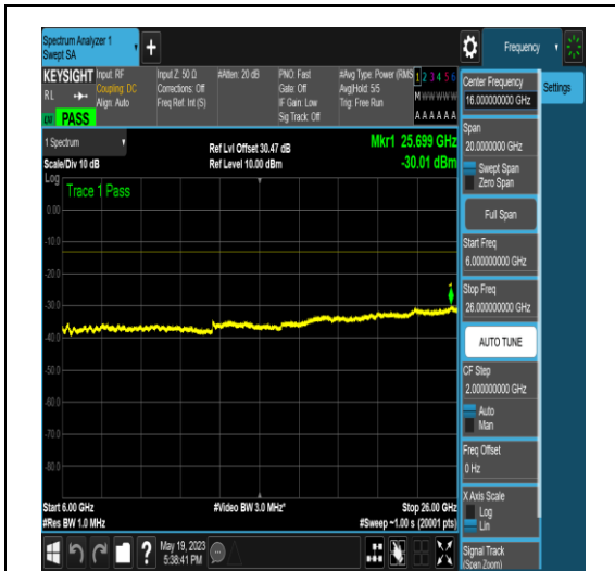
NTNV_N77-3700-3980_PC2_30_50_H_TID17_N S_01_6000_26000_#1
