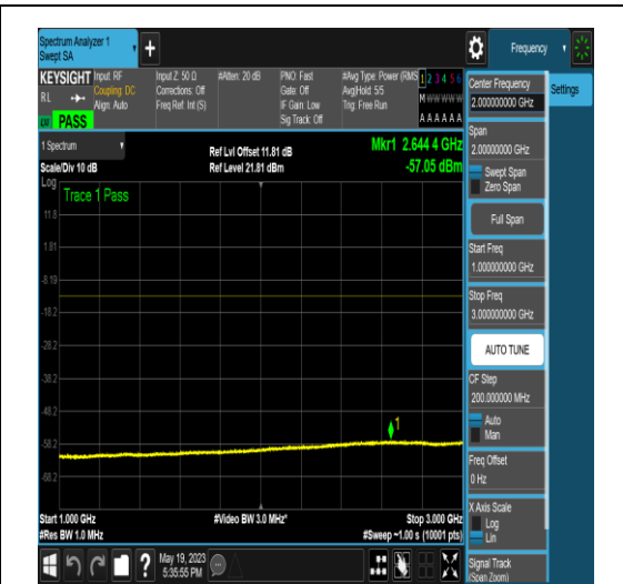
NTNV_N77-3700-3980_PC2_30_50_H_TID16_N S_01_1000_3000_#1
