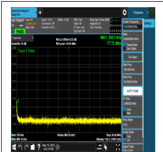
NTNV_N77-3700-3980_PC2_30_60_L_TID4_NS_01_0.15_30_#1
