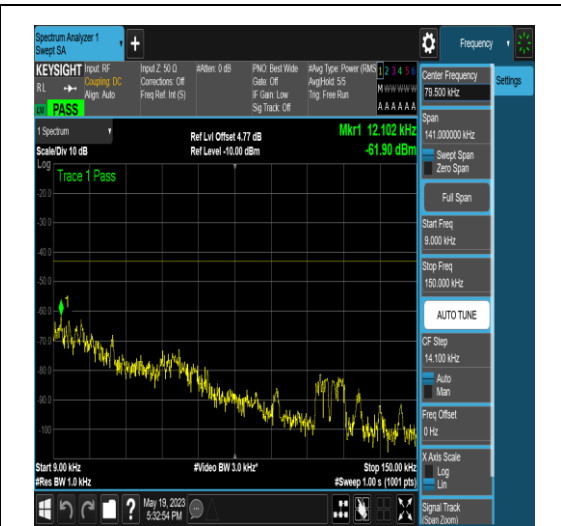
NTNV_N77-3700-3980_PC2_30_50_H_TID18_NS_01_0.009_0.15_#1
