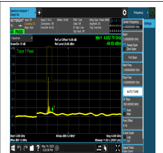
NTNV_N77-3700-3980_PC2_30_50_H_TID4_NS _01_3000_6000_#1
