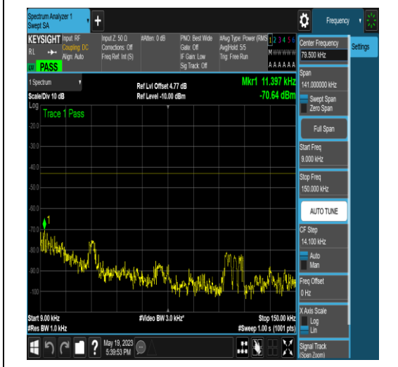
NTNV_N77-3700-3980_PC2_30_60_L_TID6_NS_01_0.009_0.15_#1
