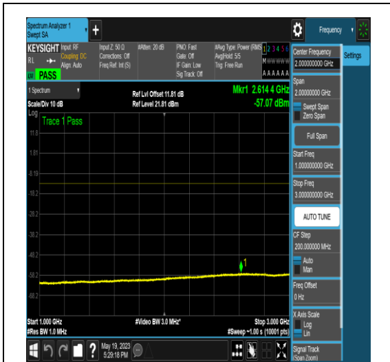
NTNV_N77-3700-3980_PC2_30_50_H_TID4_NS _01_1000_3000_#1
