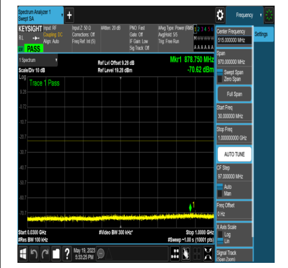
NTNV_N77-3700-3980_PC2_30_50_H_TID18_NS_01_30_1000_#1
