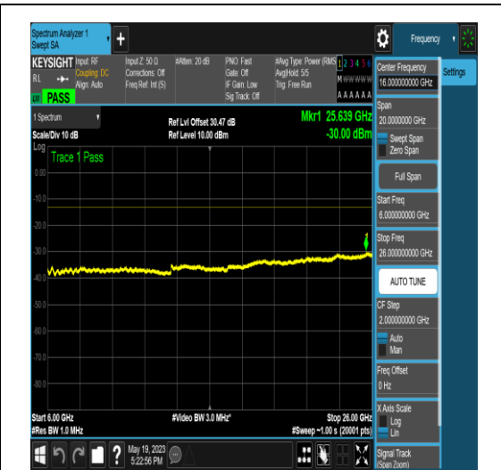
NTNV_N77-3700-3980_PC2_30_50_M_TID16_N S_01_6000_26000_#1
