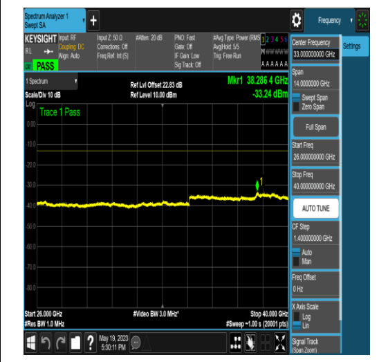
NTNV_N77-3700-3980_PC2_30_50_H_TID4_NS _01_26000_40000_#1
