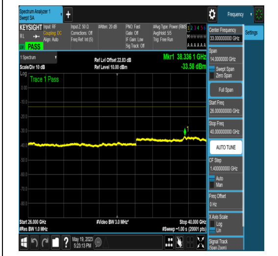
NTNV_N77-3700-3980_PC2_30_50_M_TID16_N S_01_26000_40000_#1
