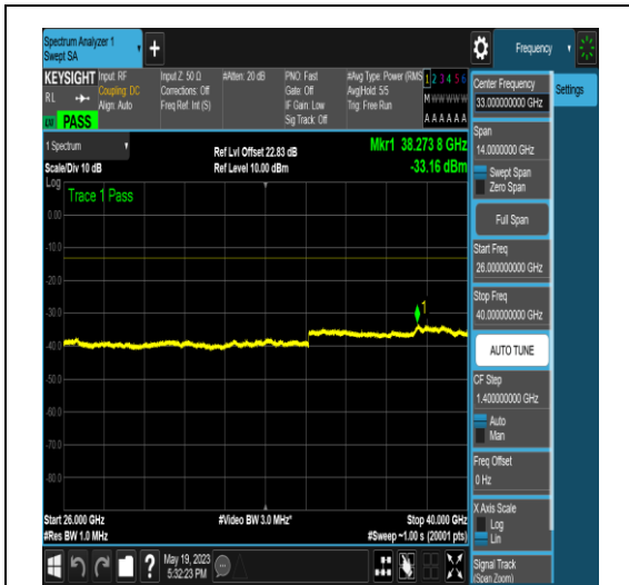
NTNV_N77-3700-3980_PC2_30_50_H_TID5_NS_01_26000_40000_#1
