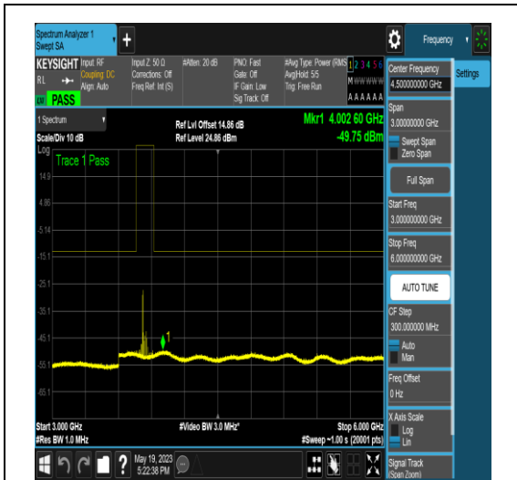
NTNV_N77-3700-3980_PC2_30_50_M_TID16_N S_01_3000_6000_#1
