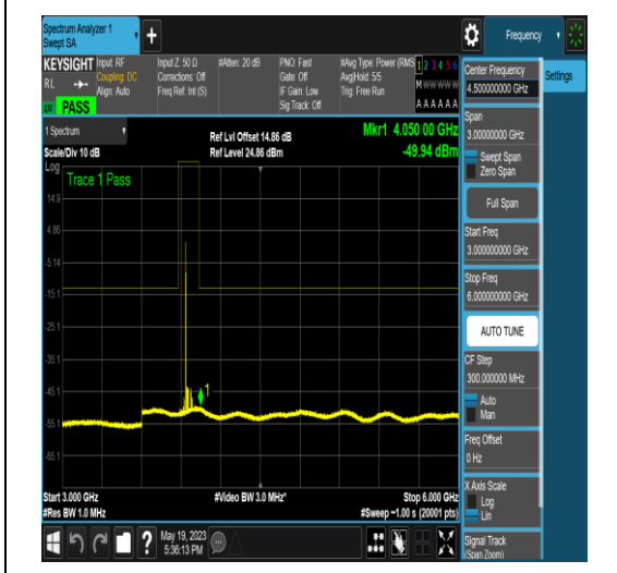
NTNV_N77-3700-3980_PC2_30_50_H_TID16_N S_01_3000_6000_#1
