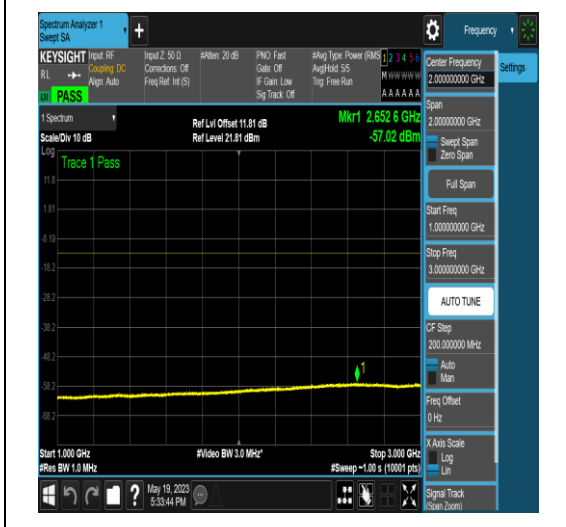
NTNV_N77-3700-3980_PC2_30_50_H_TID18_NS_01_0.15_30_#1
