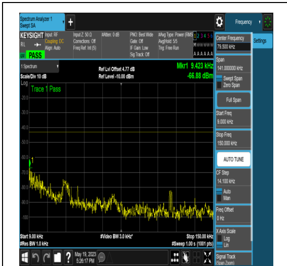
NTNV_N77-3700-3980_PC2_30_50_H_TID6_NS _01_0.009_0.15_#1
