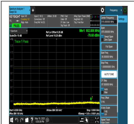
NTNV_N77-3700-3980_PC2_30_50_H_TID16_N S_01_30_1000_#1
