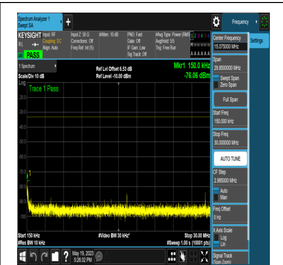
NTNV_N77-3700-3980_PC2_30_50_H_TID6_NS _01_0.15_30_#1
