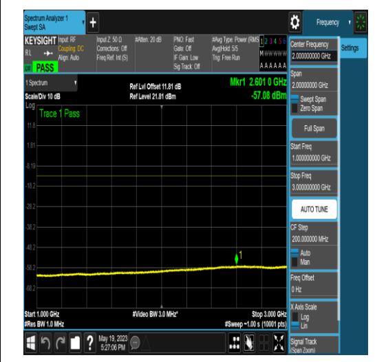
NTNV_N77-3700-3980_PC2_30_50_H_TID6_NS _01_1000_3000_#1
