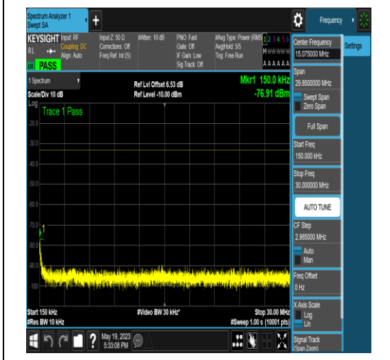
NTNV_N77-3700-3980_PC2_30_50_H_TID18_NS_01_0.15_30_#1
