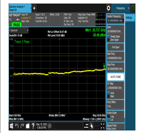
NTNV_N77-3700-3980_PC2_30_50_H_TID16_N S_01_6000_26000_#1
