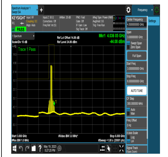
NTNV_N77-3700-3980_PC2_30_50_H_TID6_NS _01_30_1000_#1
