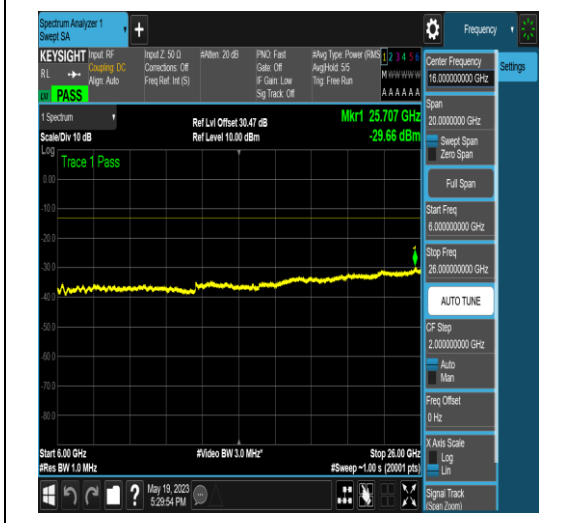
NTNV_N77-3700-3980_PC2_30_50_H_TID4_NS _01_6000_26000_#1
