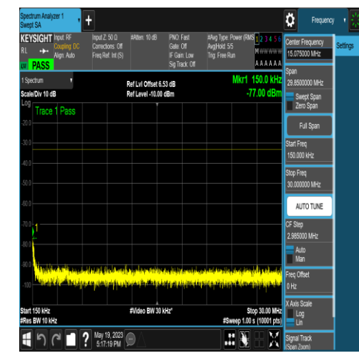
NTNV_N77-3700-3980_PC2_30_50_M_TID5_NS _01_0.15_30_#1
