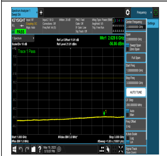
NTNV_N77-3700-3980_PC2_30_50_L_TID17_NS _01_0.15_30_#1
