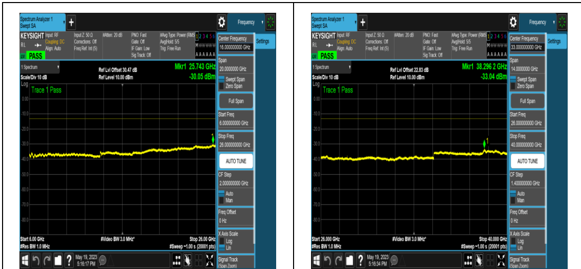
NTNV_N77-3700-3980_PC2_30_50_M_TID4_NS _01_6000_26000_#1
