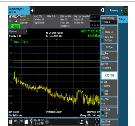
NTNV_N77-3700-3980_PC2_30_50_L_TID17_NS _01_0.009_0.15_#1
