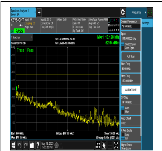
NTNV_N77-3700-3980_PC2_30_50_L_TID5_NS_01_0.009_0.15_#1
