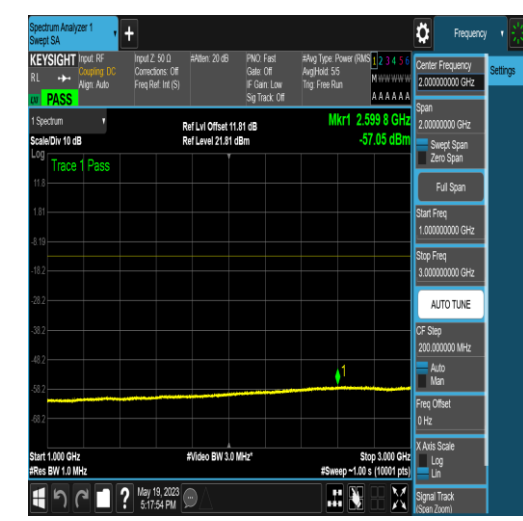
NTNV_N77-3700-3980_PC2_30_50_M_TID5_NS _01_0.15_30_#1
