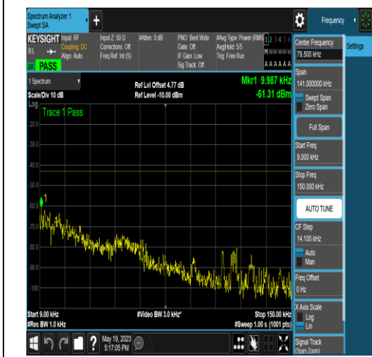
NTNV_N77-3700-3980_PC2_30_50_M_TID5_NS _01_0.009_0.15_#1
