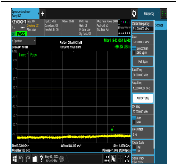
NTNV_N77-3700-3980_PC2_30_50_M_TID6_NS _01_30_1000_#1
