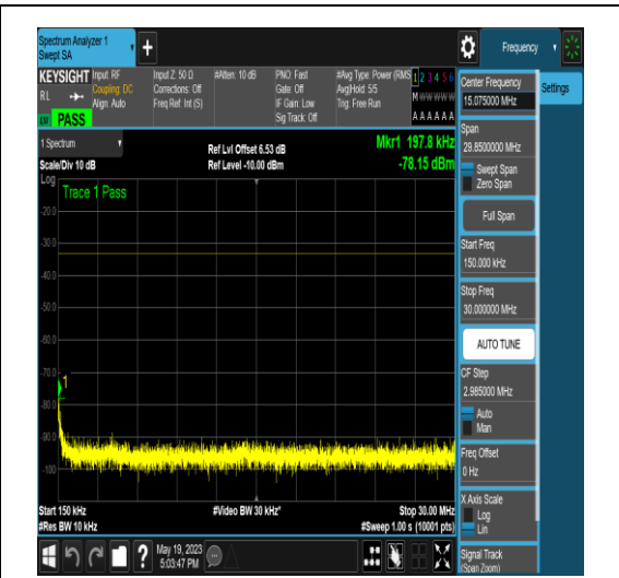
NTNV_N77-3700-3980_PC2_30_50_L_TID5_NS_01_0.15_30_#1
