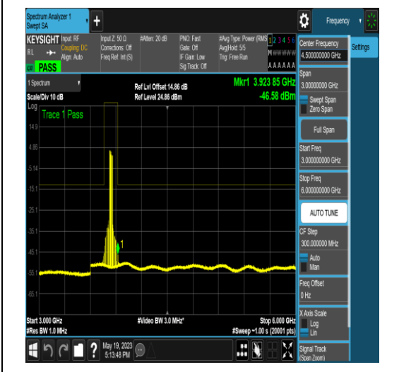
NTNV_N77-3700-3980_PC2_30_50_M_TID6_NS _01_3000_6000_#1
