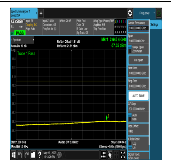
NTNV_N77-3700-3980_PC2_30_50_M_TID6_NS _01_1000_3000_#1
