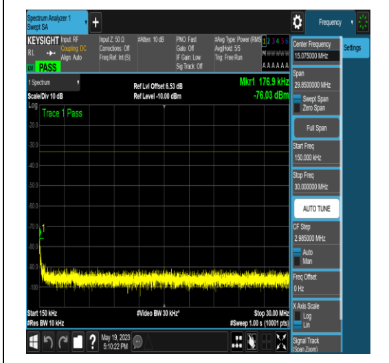
NTNV_N77-3700-3980_PC2_30_50_L_TID17_NS _01_0.15_30_#1
