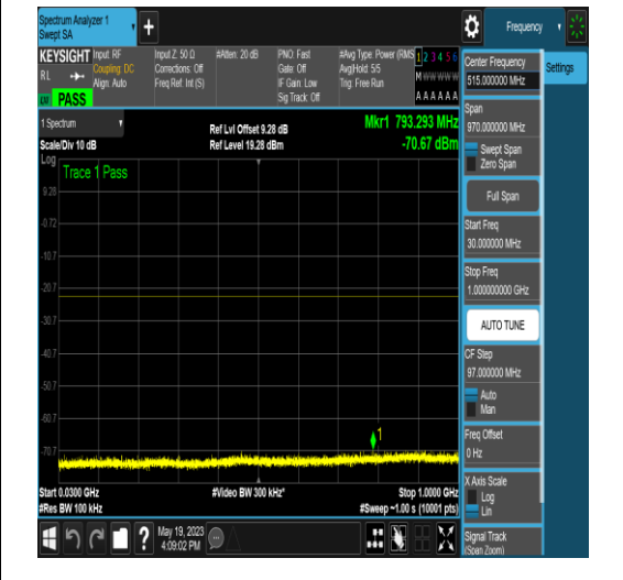
NTNV_N77-3700-3980_PC2_30_20_H_TID17_N S_01_0_009_0.15_#1
