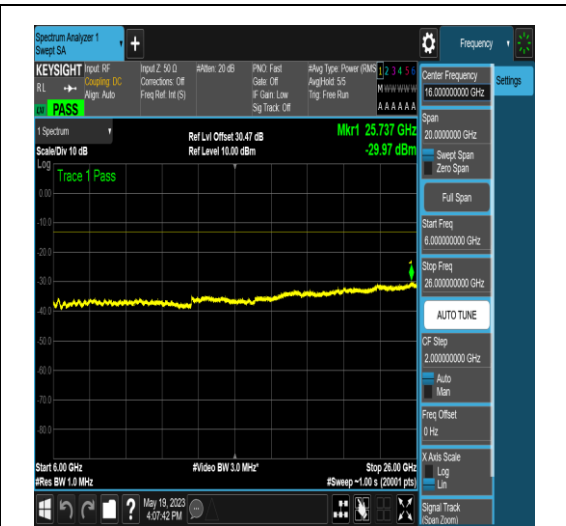
NTNV_N77-3700-3980_PC2_30_20_H_TID16_N S_01_6000_26000_#1
