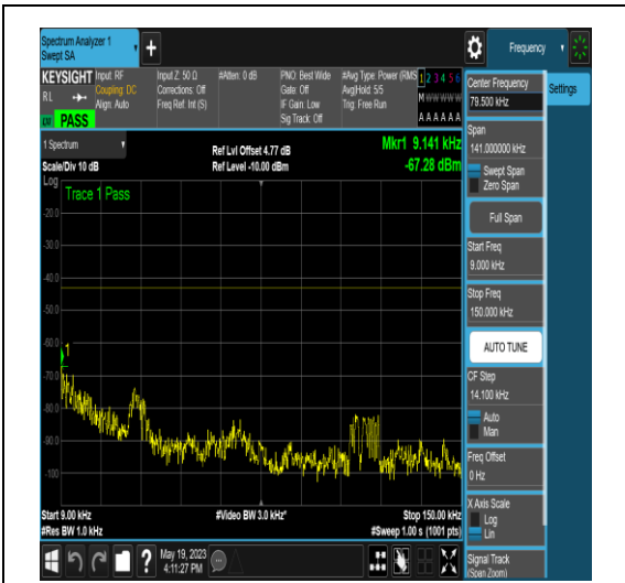
NTNV_N77-3700-3980_PC2_30_40_L_TID6_NS_01_0.009_0.15_#1
