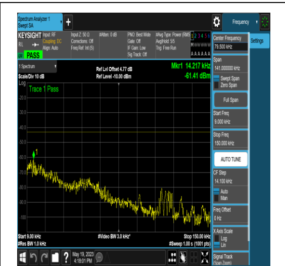
NTNV_N77-3700-3980_PC2_30_40_L_TID18_NS_01_0.009_0.15_#1
