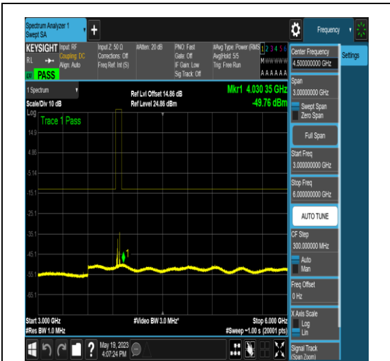
NTNV_N77-3700-3980_PC2_30_20_H_TID16_N S_01_3000_6000_#1
