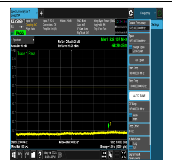
NTNV_N77-3700-3980_PC2_30_40_M_TID4_NS _01_30_1000_#1
