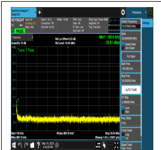
NTNV_N77-3700-3980_PC2_30_40_M_TID4_NS _01_0.15_30_#1
