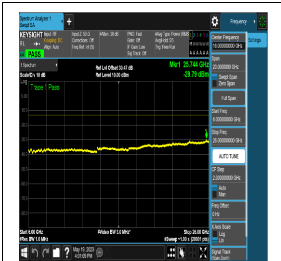
NTNV_N77-3700-3980_PC2_30_20_H_TID4_NS _01_6000_26000_#1
