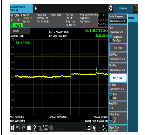
NTNV_N77-3700-3980_PC2_30_20_M_TID6_NS _01_26000_40000_#1
