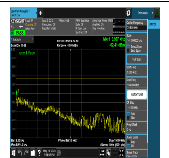
NTNV_N77-3700-3980_PC2_30_20_M_TID17_N S_01_0.009_0.15_#1
