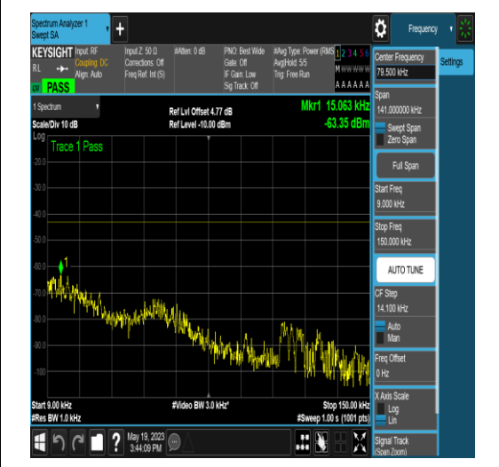
NTNV_N77-3700-3980_PC2_30_20_M_TID4_NS _01_0.009_0.15_#1
