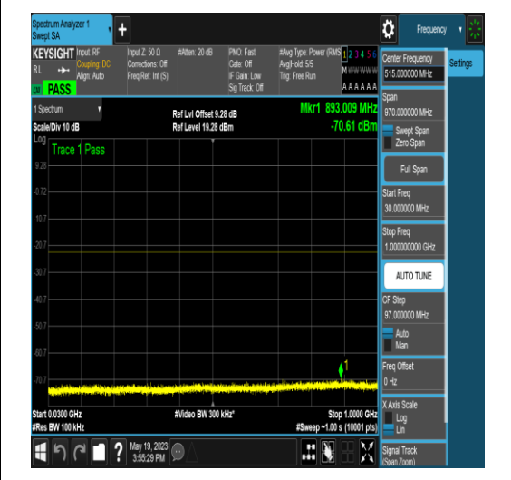
NTNV_N77-3700-3980_PC2_30_20_M_TID17_N S_01_30_1000_#1
