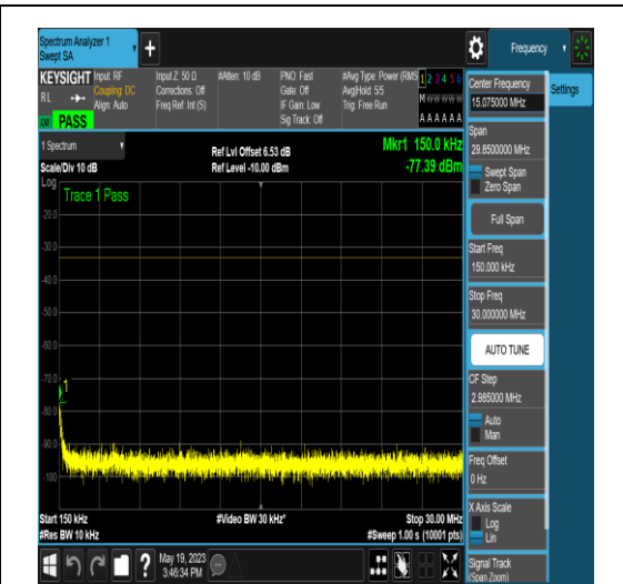
NTNV_N77-3700-3980_PC2_30_20_M_TID5_NS _01_0.15_30_#1
