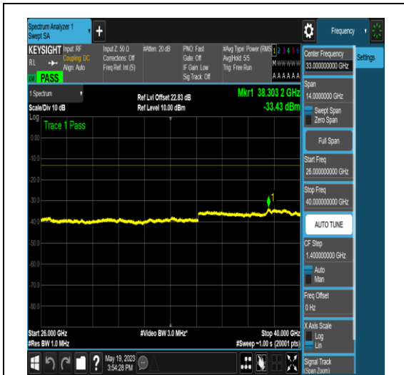
NTNV_N77-3700-3980_PC2_30_20_M_TID16_N S_01_26000_40000_#1
