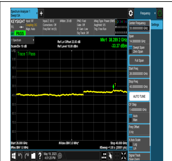
NTNV_N77-3700-3980_PC2_30_20_H_TID4_NS _01_26000_40000_#1
