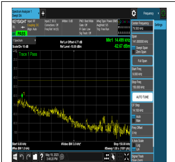
NTNV_N77-3700-3980_PC2_30_20_M_TID5_NS _01_0.009_0.15_#1
