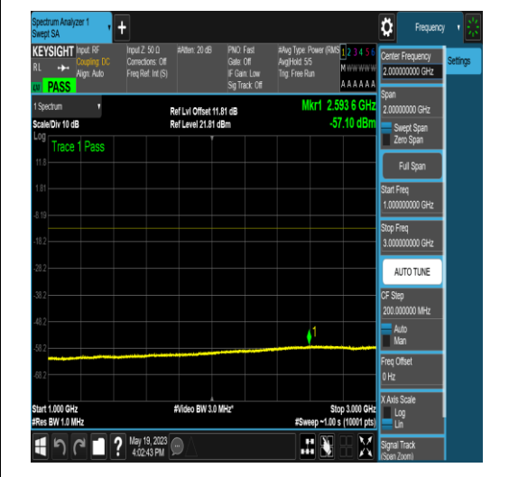
NTNV_N77-3700-3980_PC2_30_20_H_TID5_NS _01_0.15_30_#1
