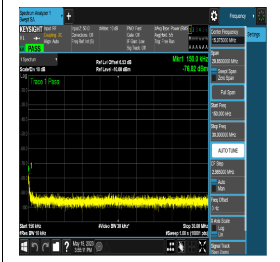
NTNV_N77-3700-3980_PC2_30_20_M_TID17_N S_01_0.15_30_#1
