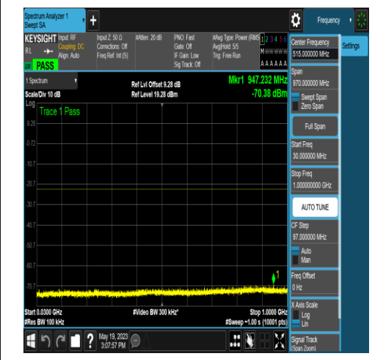
NTNV_N77-3700-3980_PC2_30_15_M_TID18_NS_01_30_1000_#1
