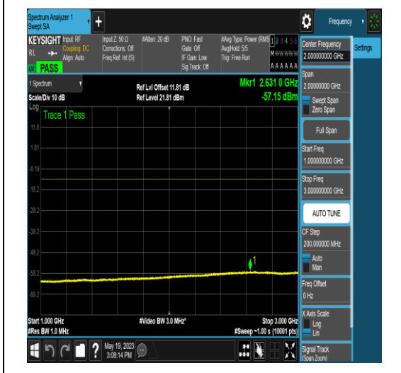
NTNV_N77-3700-3980_PC2_30_15_M_TID18_NS_01_0.15_30_#1
