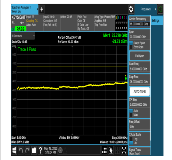
NTNV_N77-3700-3980_PC2_30_15_H_TID4_NS _01_1000_3000_#1
