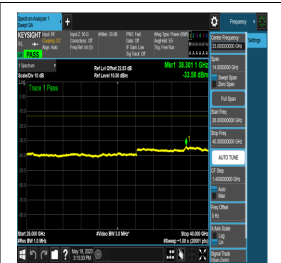
NTNV_N77-3700-3980_PC2_30_15_M_TID17_N S_01_26000_40000_#1
