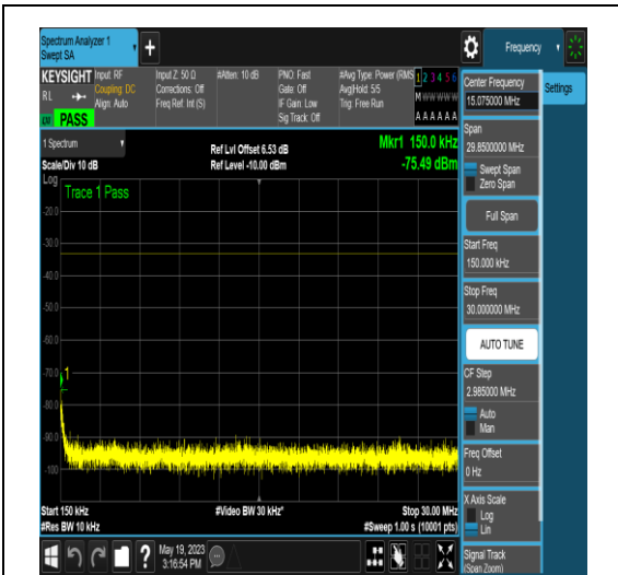
NTNV_N77-3700-3980_PC2_30_15_H_TID4_NS _01_0.15_30_#1
