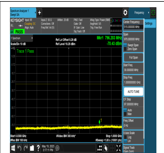
NTNV_N77-3700-3980_PC2_30_15_H_TID4_NS _01_30_1000_#1
