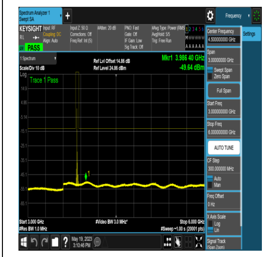
NTNV_N77-3700-3980_PC2_30_15_M_TID16_N S_01_3000_6000_#1
