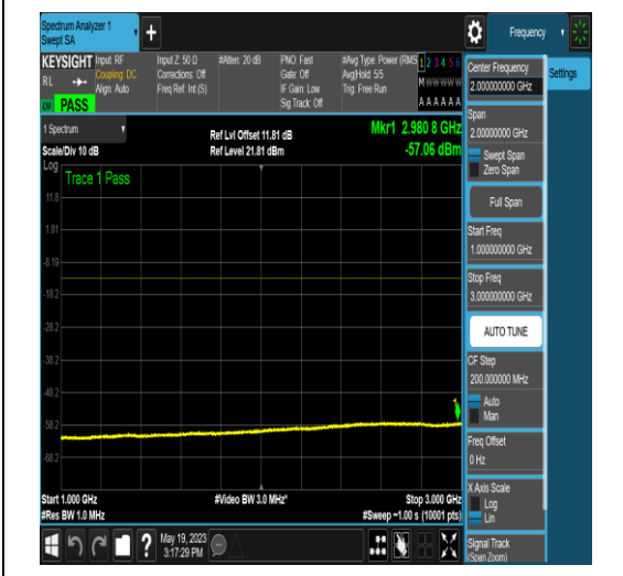
NTNV_N77-3700-3980_PC2_30_15_H_TID4_NS _01_1000_3000_#1
