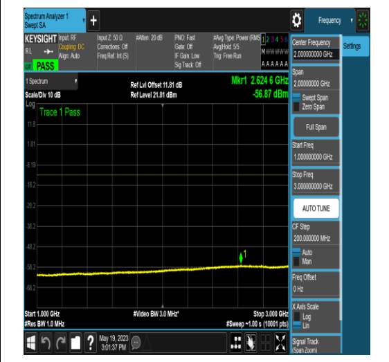
NTNV_N77-3700-3980_PC2_30_15_M_TID6_NS _01_1000_3000_#1
