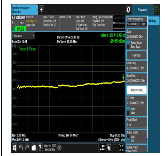
NTNV_N77-3700-3980_PC2_30_15_M_TID4_NS _01_6000_26000_#1
