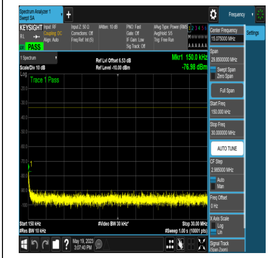
NTNV_N77-3700-3980_PC2_30_15_M_TID18_NS_01_0.15_30_#1
