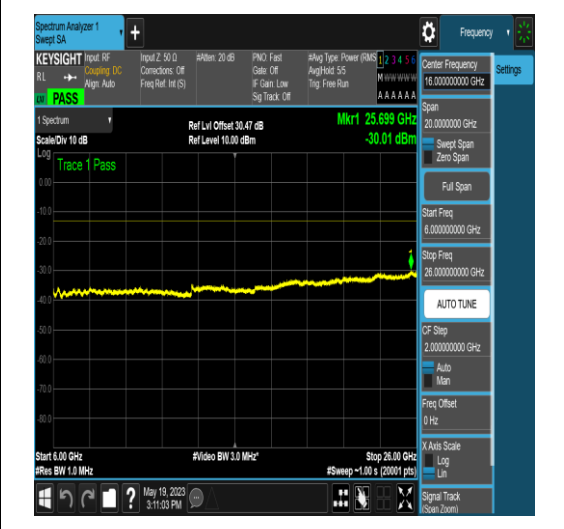
NTNV_N77-3700-3980_PC2_30_15_M_TID16_N S_01_6000_26000_#1
