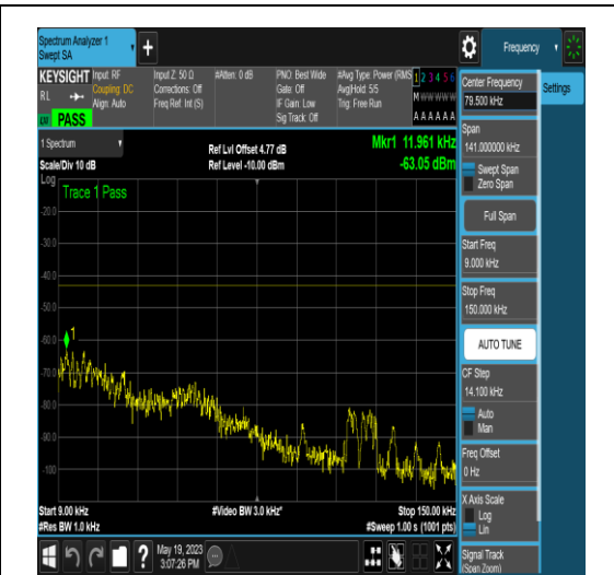
NTNV_N77-3700-3980_PC2_30_15_M_TID18_NS_01_0.009_0.15_#1
