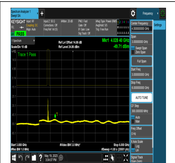
NTNV_N77-3700-3980_PC2_30_15_M_TID4_NS _01_3000_6000_#1
