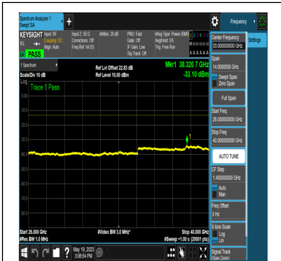
NTNV_N77-3700-3980_PC2_30_15_M_TID5_NS_01_26000_40000_#1
