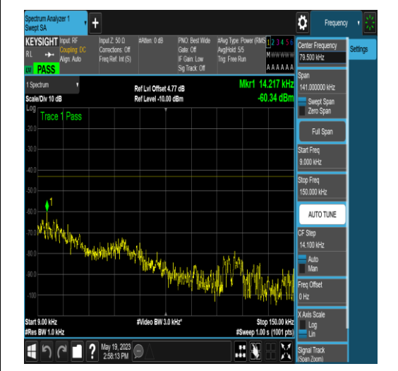
NTNV_N77-3700-3980_PC2_30_15_L_TID17_NS _01_0.009_0.15_#1
