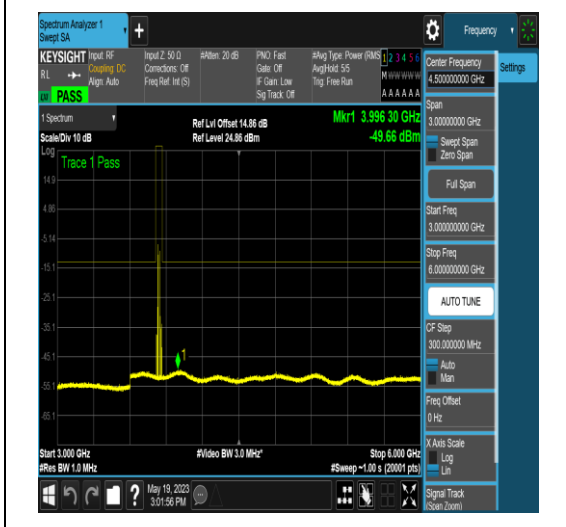
NTNV_N77-3700-3980_PC2_30_15_M_TID6_NS _01_30_1000_#1
