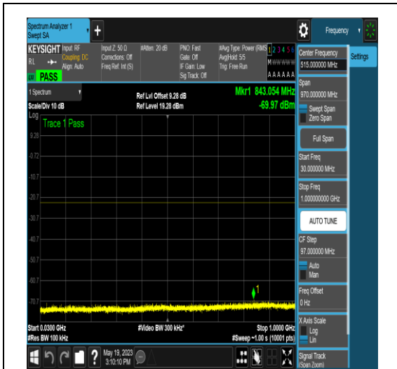
NTNV_N77-3700-3980_PC2_30_15_M_TID16_N S_01_30_1000_#1
