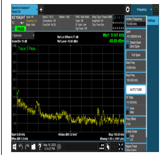
NTNV_N77-3700-3980_PC2_30_15_H_TID6_NS _01_0.009_0.15_#1
