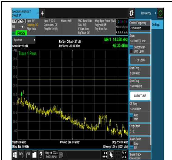
NTNV_N77-3700-3980_PC2_30_15_M_TID6_NS _01_0.009_0.15_#1
