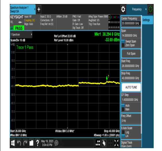
NTNV_N77-3700-3980_PC2_30_15_M_TID4_NS _01_26000_40000_#1
