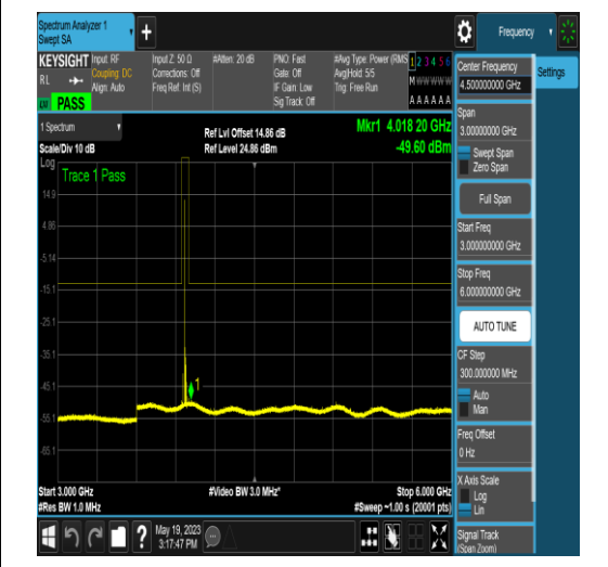
NTNV_N77-3700-3980_PC2_30_15_H_TID4_NS _01_3000_6000_#1
