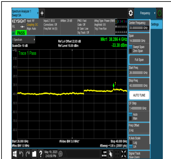
NTNV_N77-3700-3980_PC2_30_10_H_TID16_N S_01_26000_40000_#1
