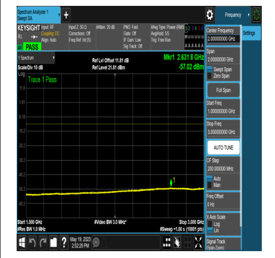
NTNV_N77-3700-3980_PC2_30_15_L_TID5_NS_01_0.15_30_#1
