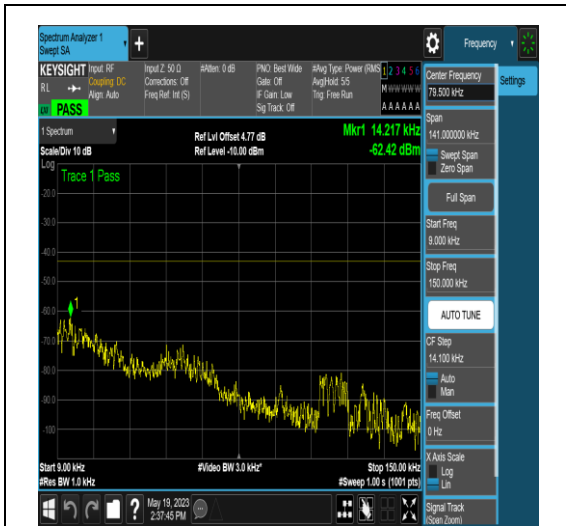
NTNV_N77-3700-3980_PC2_30_10_H_TID5_NS _01_0.009_0.15_#1
