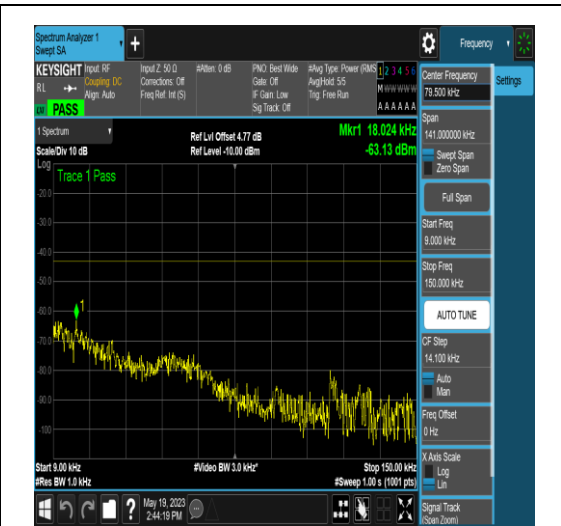
NTNV_N77-3700-3980_PC2_30_10_H_TID17_N S_01_0.009_0.15_#1
