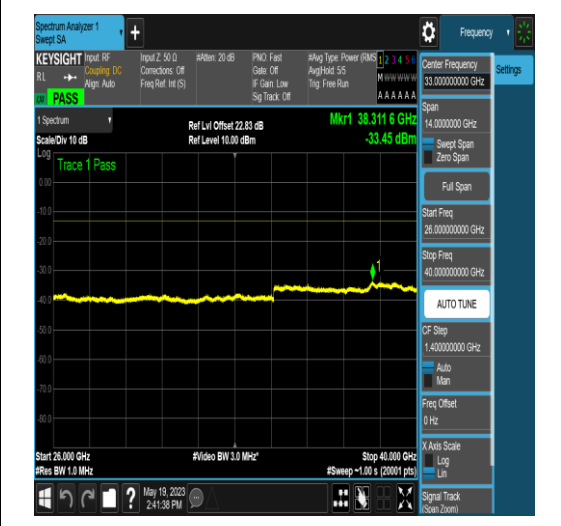
NTNV_N77-3700-3980_PC2_30_10_H_TID18_N S_01_26000_40000_#1
