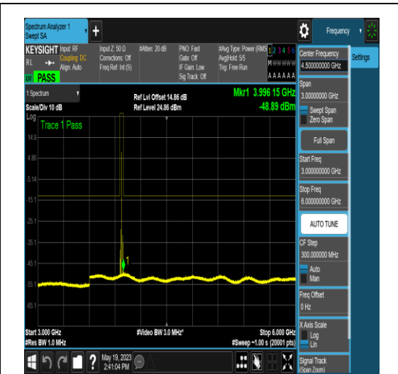
NTNV_N77-3700-3980_PC2_30_10_H_TID18_N S_01_3000_6000_#1
