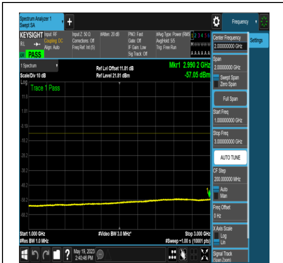
NTNV_N77-3700-3980_PC2_30_10_H_TID18_N S_01_1000_3000_#1
