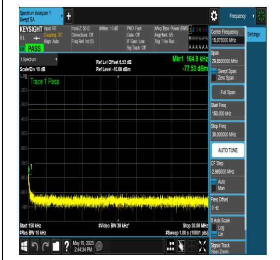
NTNV_N77-3700-3980_PC2_30_10_H_TID17_N S_01_0.15_30_#1
