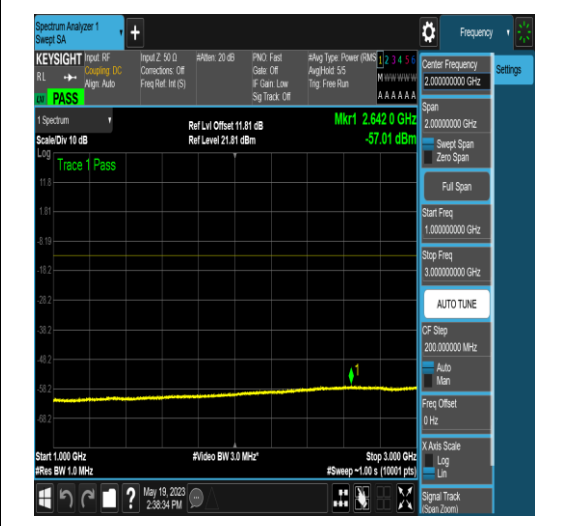
NTNV_N77-3700-3980_PC2_30_10_H_TID5_NS _01_1000_3000_#1
