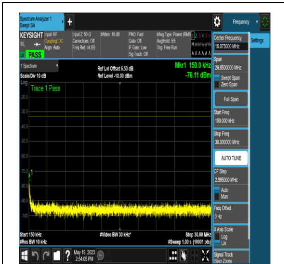
NTNV_N77-3700-3980_PC2_30_15_L_TID18_NS _01_0.15_30_#1
