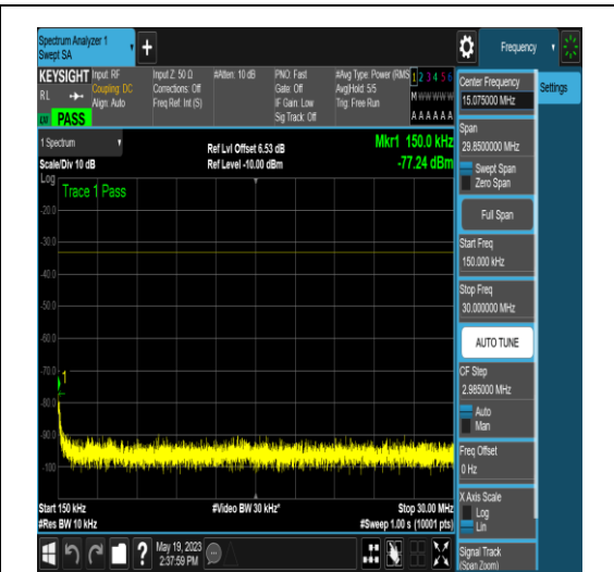
NTNV_N77-3700-3980_PC2_30_10_H_TID5_NS _01_0.15_30_#1
