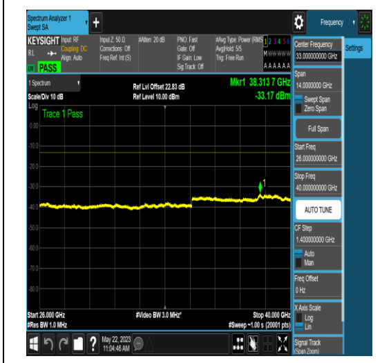
NTNV_N77-3700-3980_PC2_30_80_H_TID5_NS _01_26000_40000_#1
