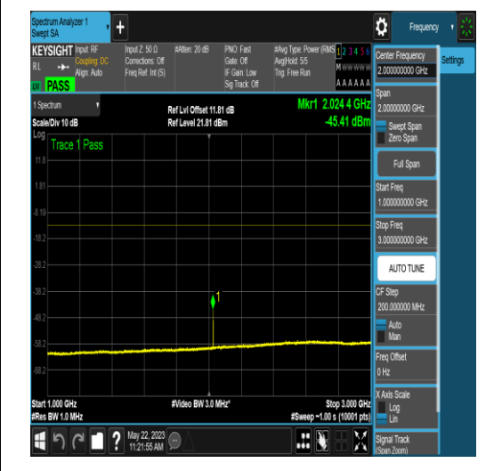
NTNV_N77-3700-3980_PC2_30_90_L_TID16_NS _01_0.15_30_#1
