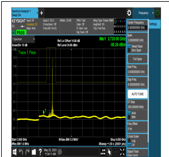
NTNV_N77-3700-3980_PC2_30_80_H_TID5_NS _01_3000_6000_#1
