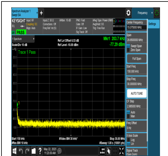
NTNV_N77-3700-3980_PC2_30_90_L_TID17_NS _01_0.15_30_#1
