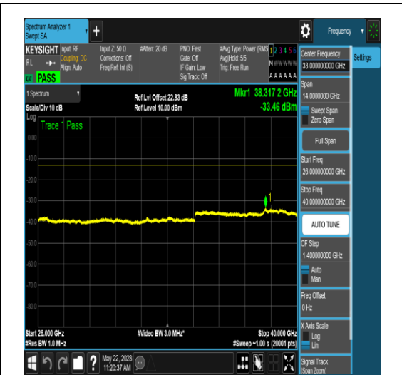
NTNV_N77-3700-3980_PC2_30_90_L_TID18_NS _01_26000_40000_#1
