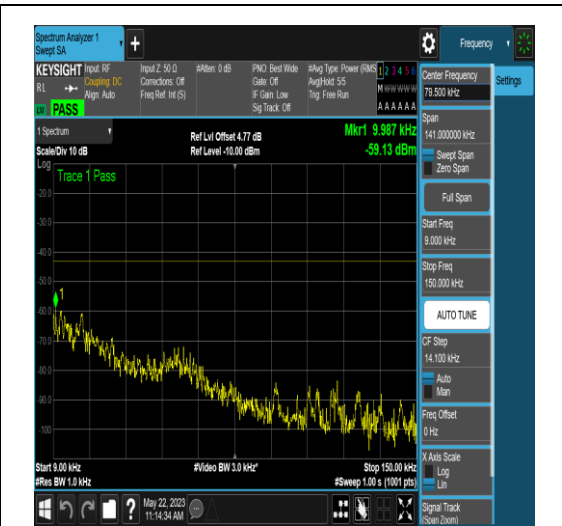
NTNV_N77-3700-3980_PC2_30_90_L_TID4_NS_01_0.009_0.15_#1
