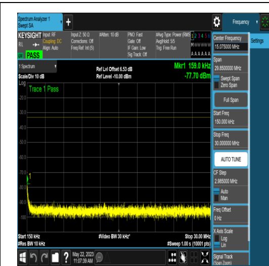
NTNV_N77-3700-3980_PC2_30_80_H_TID16_N S_01_0.15_30_#1
