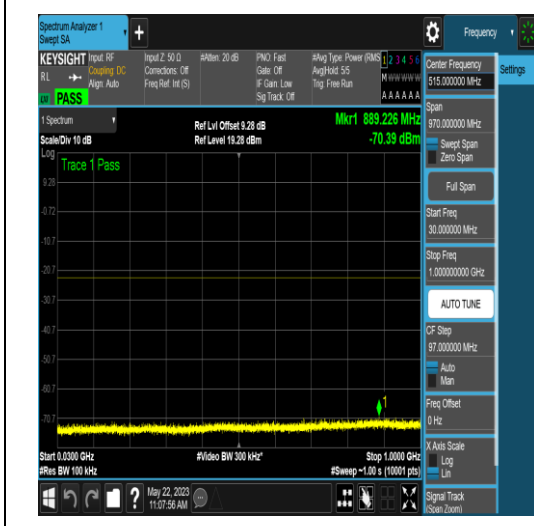
NTNV_N77-3700-3980_PC2_30_80_H_TID16_N S_01_30_1000_#1
