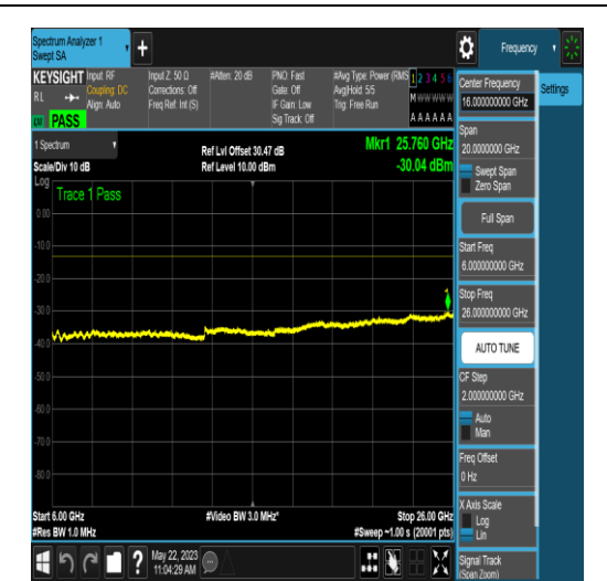
NTNV_N77-3700-3980_PC2_30_80_H_TID5_NS _01_6000_26000_#1
