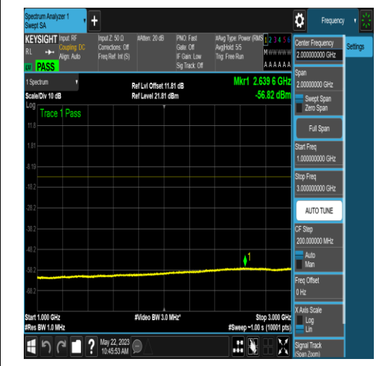
NTNV_N77-3700-3980_PC2_30_80_M_TID6_NS _01_1000_3000_#1
