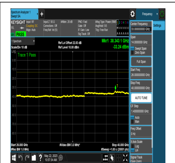
NTNV_N77-3700-3980_PC2_30_80_M_TID17_N S_01_26000_40000_#1
