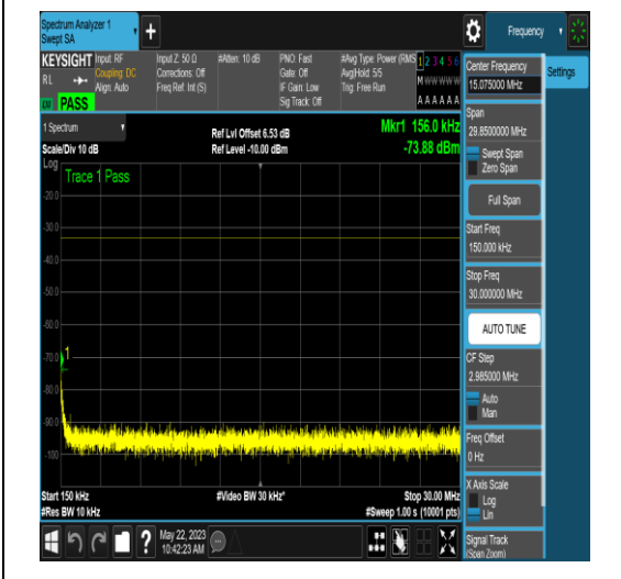
NTNV_N77-3700-3980_PC2_30_80_L_TID16_NS _01_26000_40000_#1
