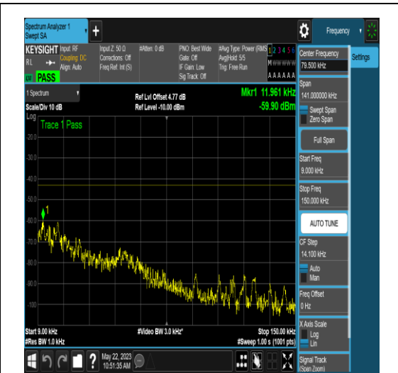
NTNV_N77-3700-3980_PC2_30_80_M_TID18_NS_01_0.009_0.15_#1
