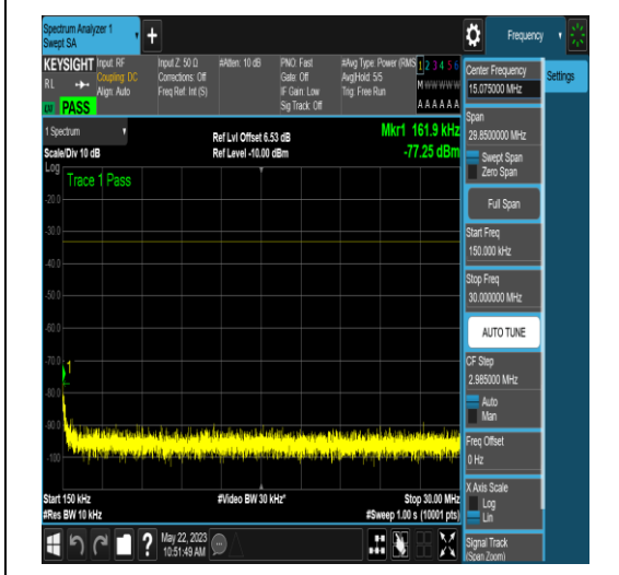
NTNV_N77-3700-3980_PC2_30_80_M_TID18_NS_01_0.15_30_#1
