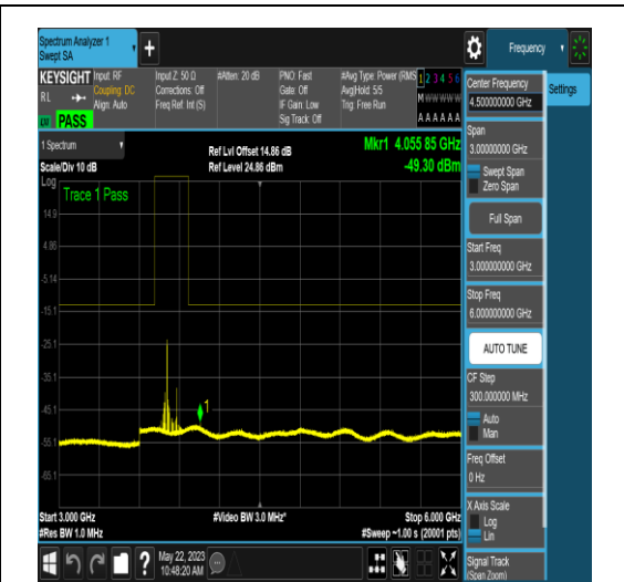
NTNV_N77-3700-3980_PC2_30_80_M_TID4_NS _01_3000_6000_#1
