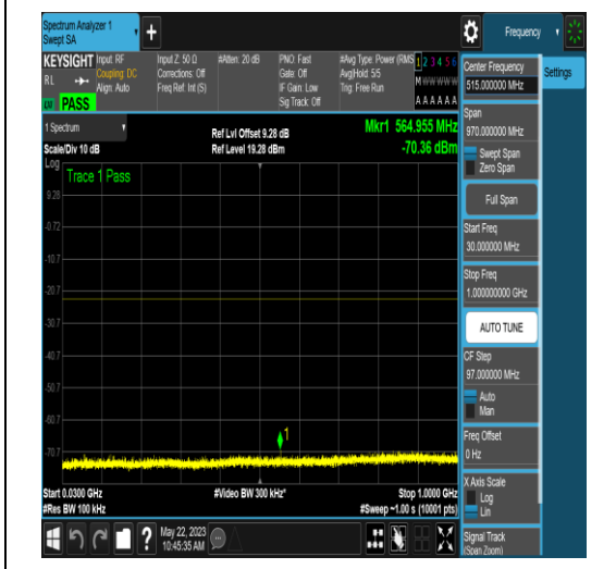
NTNV_N77-3700-3980_PC2_30_80_M_TID6_NS _01_30_1000_#1
