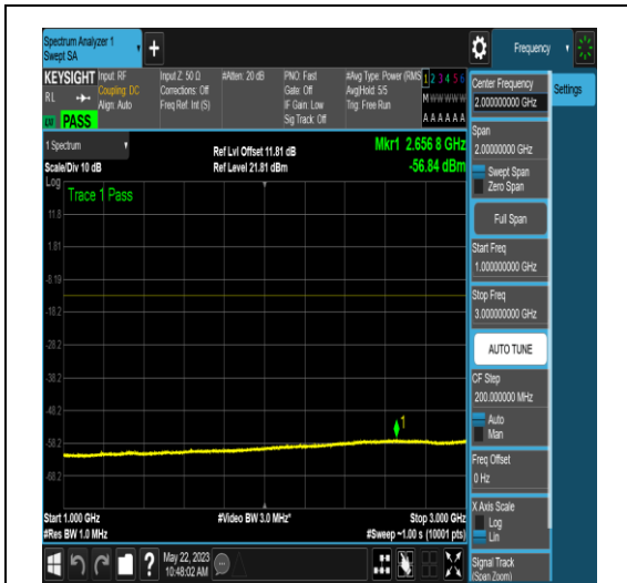
NTNV_N77-3700-3980_PC2_30_80_M_TID4_NS _01_1000_3000_#1
