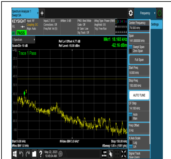
NTNV_N77-3700-3980_PC2_30_80_M_TID6_NS _01_0.009_0.15_#1
