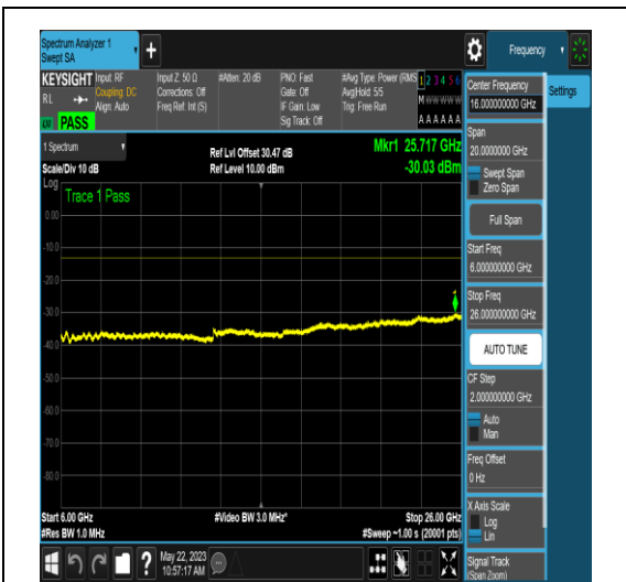
NTNV_N77-3700-3980_PC2_30_80_M_TID17_N S_01_6000_26000_#1
