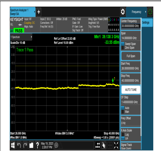
NTNV_N77-3700-3980_PC2_30_10_M_TID18_N S_01_26000_40000_#1
