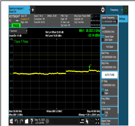
NTNV_N77-3700-3980_PC2_30_10_M_TID6_NS_01_26000_40000_#1
