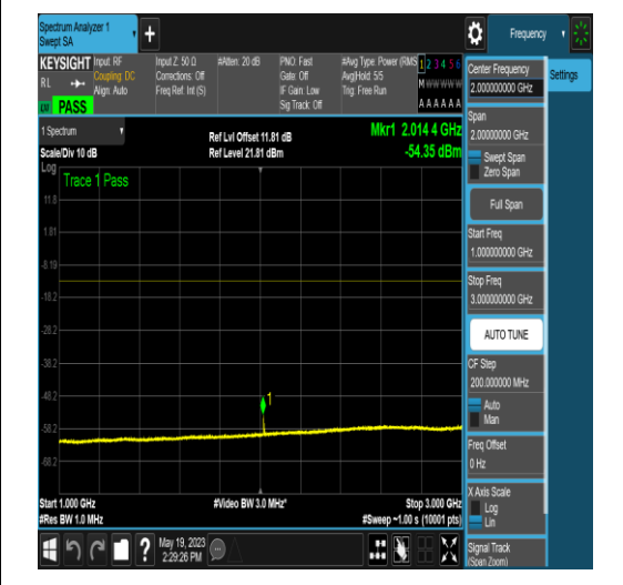
NTNV_N77-3700-3980_PC2_30_10_M_TID16_N S_01_0.15_30_#1
