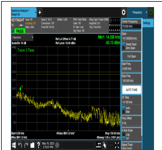
NTNV_N77-3700-3980_PC2_30_10_L_TID16_NS _01_0.009_0.15_#1
