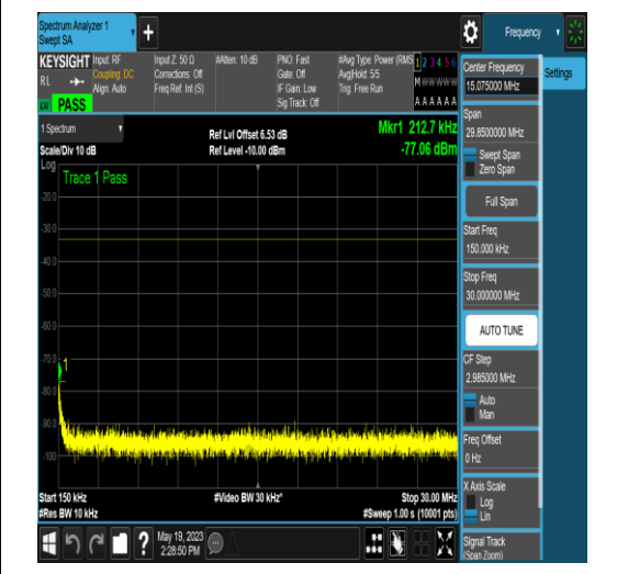
NTNV_N77-3700-3980_PC2_30_10_M_TID16_N S_01_0.15_30_#1
