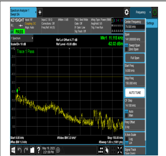
NTNV_N77-3700-3980_PC2_30_10_M_TID4_NS_01_0.009_0.15_#1
