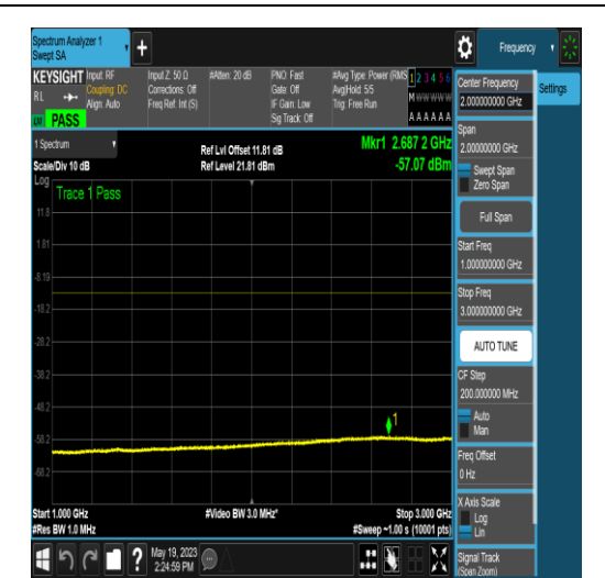
NTNV_N77-3700-3980_PC2_30_10_M_TID5_NS _01_1000_3000_#1
