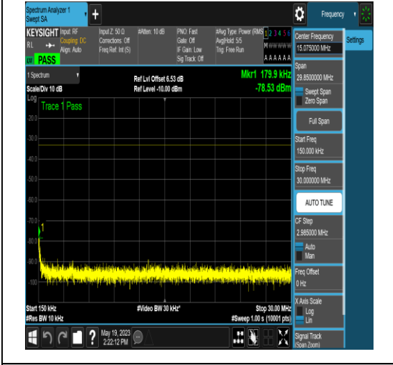
NTNV_N77-3700-3980_PC2_30_10_M_TID4_NS_01_0.15_30_#1
