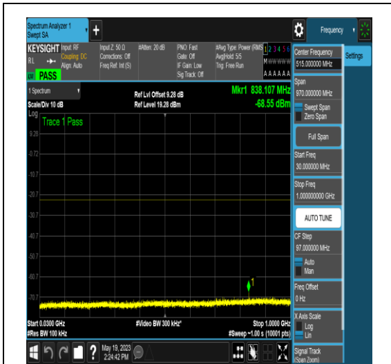
NTNV_N77-3700-3980_PC2_30_10_M_TID5_NS _01_30_1000_#1
