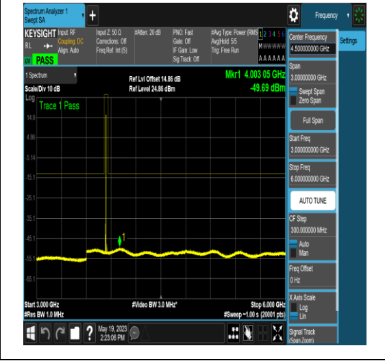
NTNV_N77-3700-3980_PC2_30_10_M_TID4_NS_01_30_1000_#1
