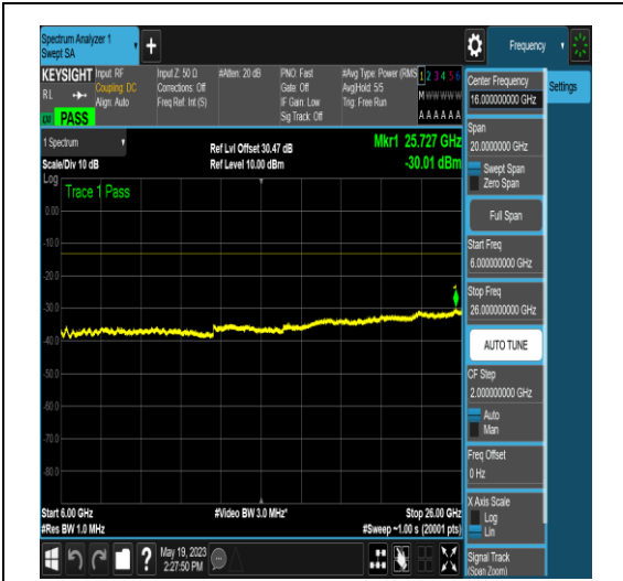
NTNV_N77-3700-3980_PC2_30_10_M_TID18_N S_01_6000_26000_#1
