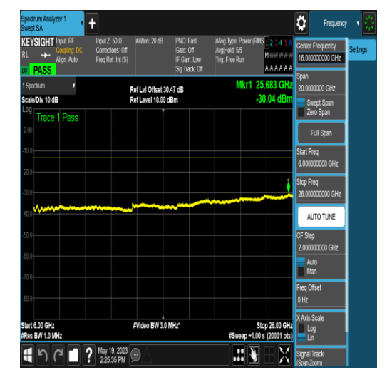
NTNV_N77-3700-3980_PC2_30_10_M_TID5_NS _01_6000_26000_#1
