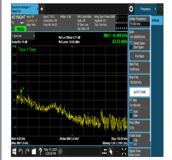
NTNV_N77-3700-3980_PC2_30_10_M_TID16_N S_01_0.009_0.15_#1
