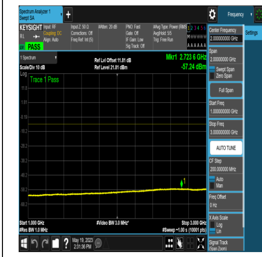
NTNV_N77-3700-3980_PC2_30_10_M_TID17_N S_01_1000_3000_#1
