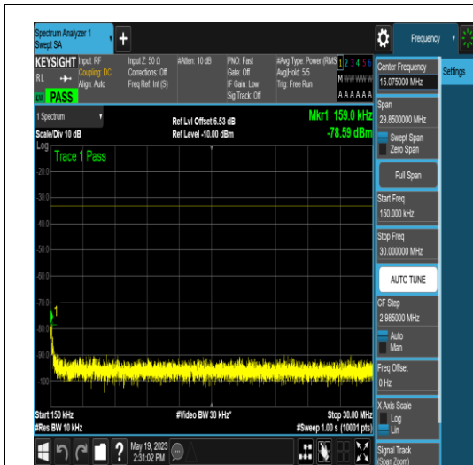
NTNV_N77-3700-3980_PC2_30_10_M_TID17_N S_01_0.15_30_#1
