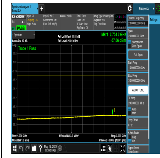
NTNV_N77-3700-3980_PC2_30_100_H_TID18_N S_01_0.15_30_#1
