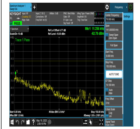
NTNV_N77-3700-3980_PC2_30_10_L_TID6_NS 01_0.009_0.15_#1
