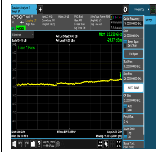
NTNV_N77-3700-3980_PC2_30_100_H_TID4_N S_01_6000_26000_#1
