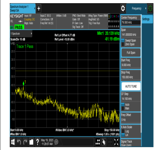
NTNV_N77-3700-3980_PC2_30_100_M_TID17_ NS_01_0.009_0.15_#1
