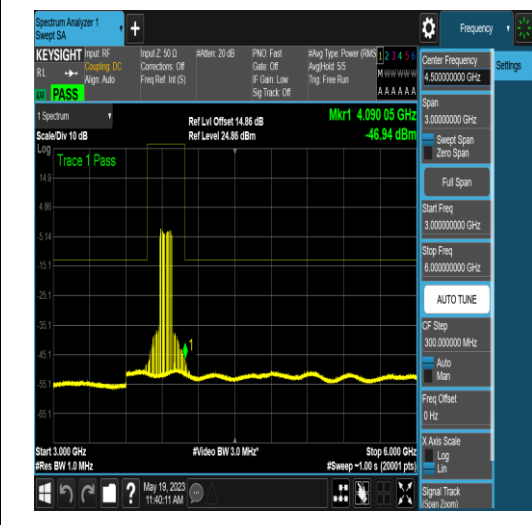
NTNV_N77-3700-3980_PC2_30_100_H_TID18_N S_01_30_1000_#1
