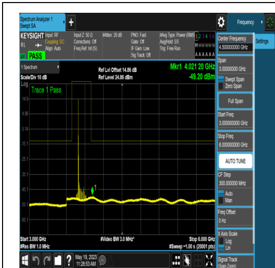
NTNV_N77-3700-3980_PC2_30_100_M_TID16_ NS_01_3000_6000_#1
