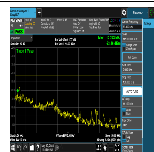
NTNV_N77-3700-3980_PC2_30_100_H_TID18_N S_01_0.009_0.15_#1
