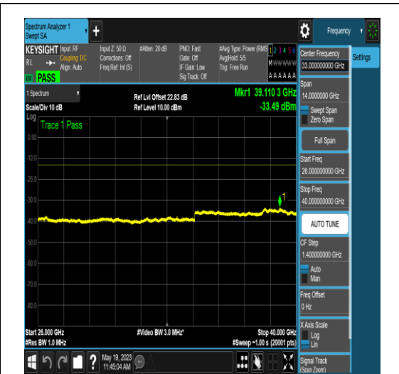
NTNV_N77-3700-3980_PC2_30_100_H_TID17_N S_01_26000_40000_#1
