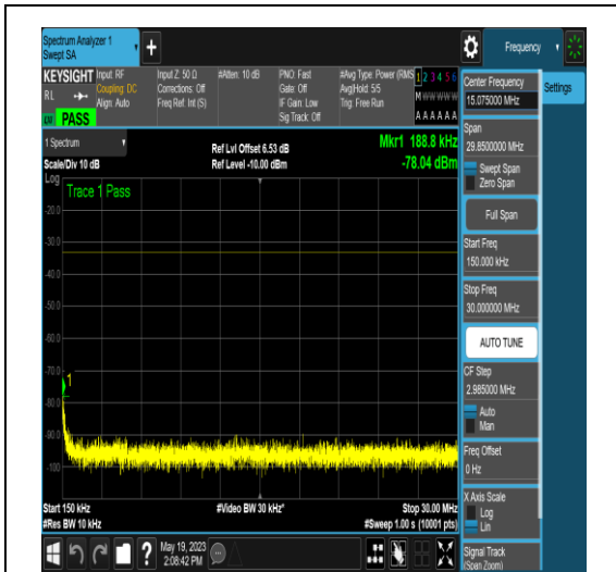
NTNV_N77-3700-3980_PC2_30_10_L_TID4_NS_01_0.15_30_#1
