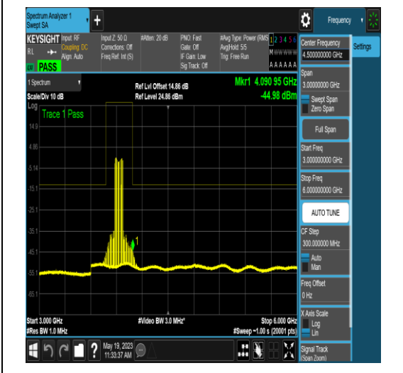
NTNV_N77-3700-3980_PC2_30_100_H_TID6_N S_01_30_1000_#1
