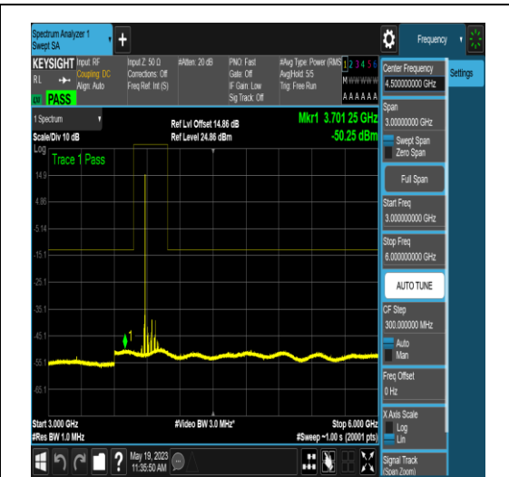
NTNV_N77-3700-3980_PC2_30_100_H_TID4_N S_01_3000_6000_#1
