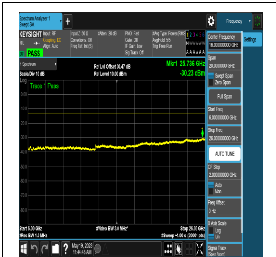
NTNV_N77-3700-3980_PC2_30_100_H_TID17_N S_01_6000_26000_#1
