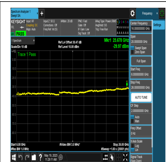
NTNV_N77-3700-3980_PC2_30_100_M_TID16_ NS_01_6000_26000_#1
