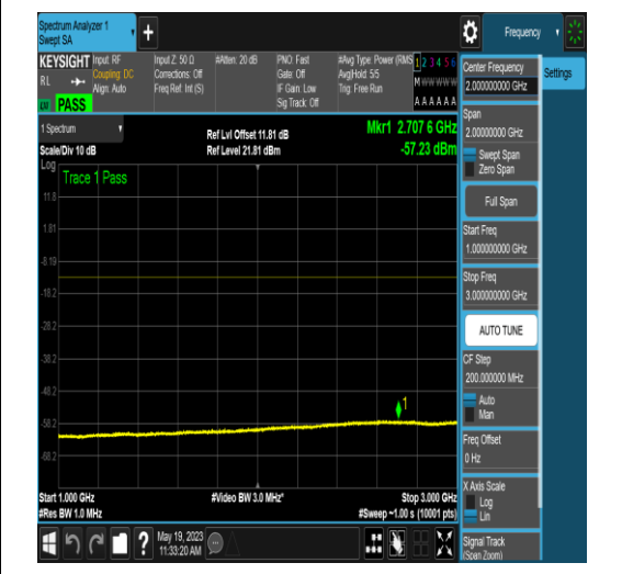
NTNV_N77-3700-3980_PC2_30_100_H_TID6_N S_01_1000_3000_#1
