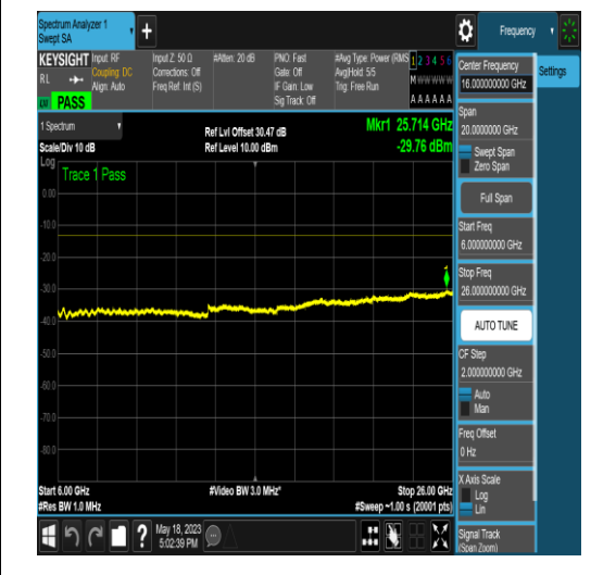
NTNV_N77-3450-3550_PC2_30_80_M_TID5_N/A _1000_3000_#1
