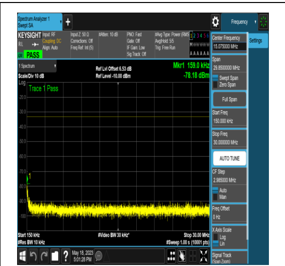
NTNV_N77-3450-3550_PC2_30_80_M_TID5_N/A _0.15_30_#1
