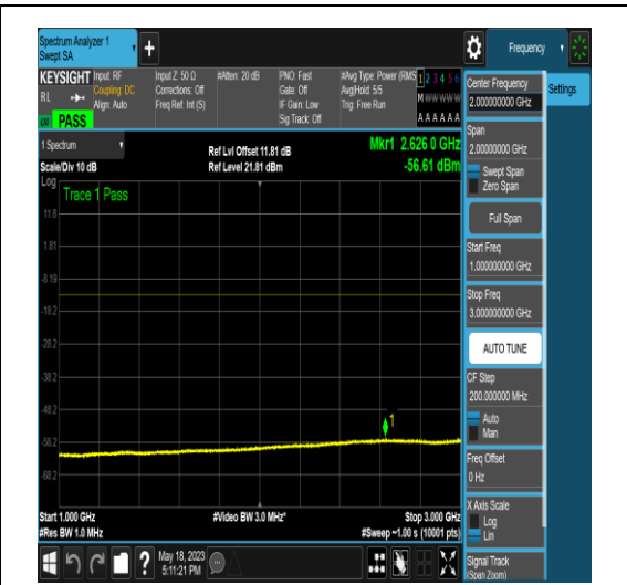
NTNV_N77-3450-3550_PC2_30_80_H_TID6_N/A _1000_3000_#1
