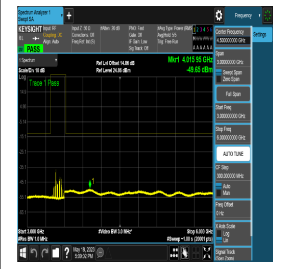
NTNV_N77-3450-3550_PC2_30_80_M_TID17_NV A_30_1000_#1
