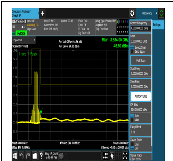
NTNV_N77-3450-3550_PC2_30_80_M_TID6_N/A _3000_6000_#1
