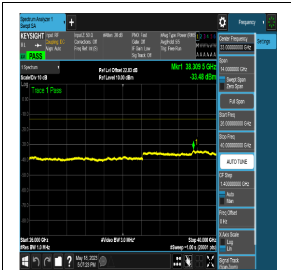
NTNV_N77-3450-3550_PC2_30_80_M_TID16_NV A_26000_40000_#1
