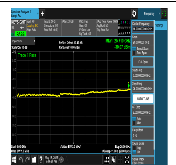
NTNV_N77-3450-3550_PC2_30_80_M_TID6_N/A _6000_26000_#1
