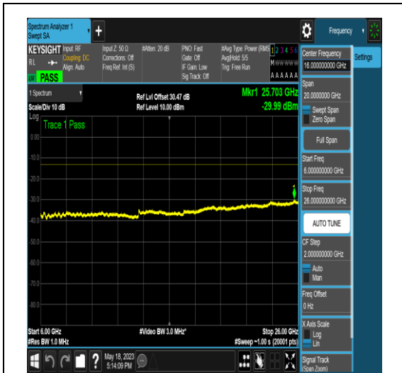
NTNV_N77-3450-3550_PC2_30_80_H_TID4_N/A _6000_26000_#1
