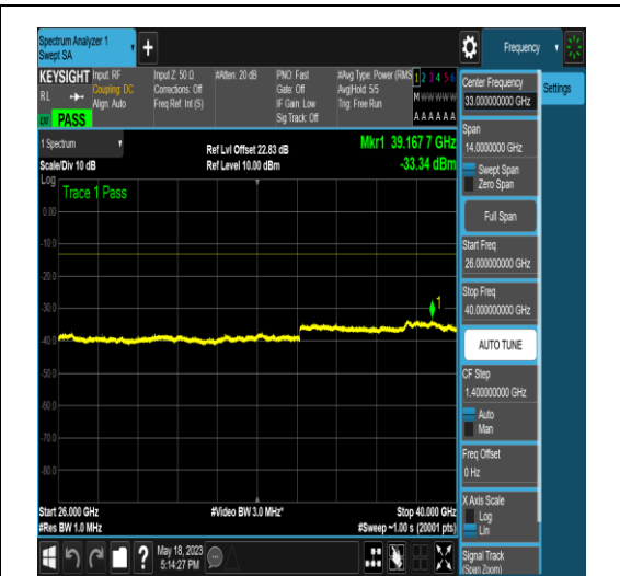
NTNV_N77-3450-3550_PC2_30_80_H_TID4_N/A _26000_40000_#1
