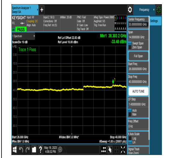
NTNV_N77-3450-3550_PC2_30_80_M_TID6_N/A _26000_40000_#1
