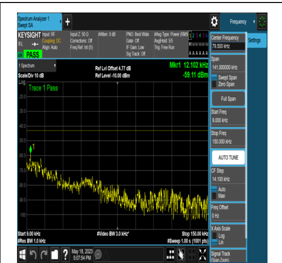
NTNV_N77-3450-3550_PC2_30_80_M_TID17_NV A_0.009_0.15_#1
