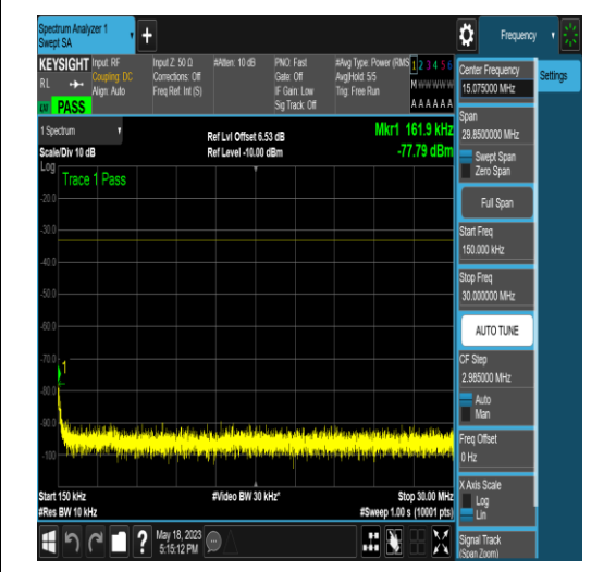
NTNV_N77-3450-3550_PC2_30_80_H_TID5_N/A _0.15_30_#1
