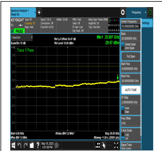
NTNV_N77-3450-3550_PC2_30_80_L_TID18_N/ A_6000_26000_#1
