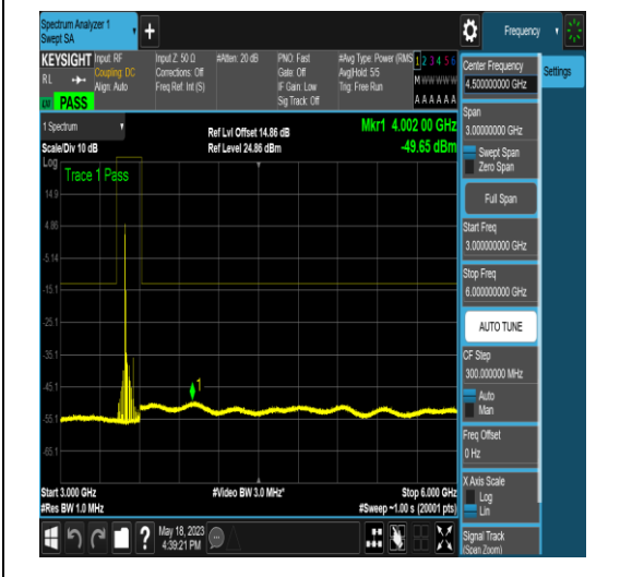
NTNV_N77-3450-3550_PC2_30_60_H_TID16_N/A_30_1000_#1
