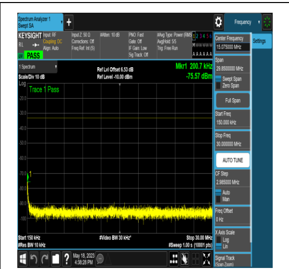
NTNV_N77-3450-3550_PC2_30_60_H_TID16_N/A_0.15_30_#1
