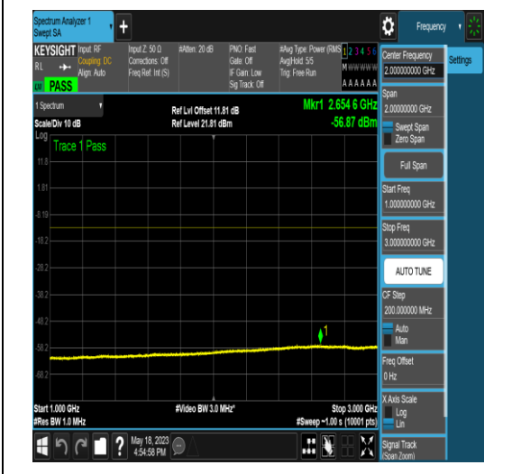
NTNV_N77-3450-3550_PC2_30_80_L_TID17_N/ A_1000_3000_#1
