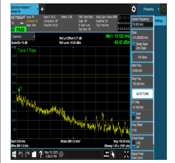
NTNV_N77-3450-3550_PC2_30_60_H_TID18_N/ A_0.009_0.15_#1
