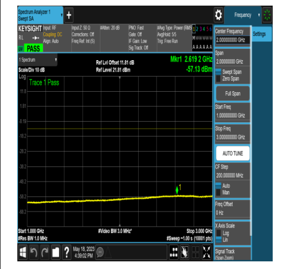
NTNV_N77-3450-3550_PC2_30_60_H_TID16_N/A_1000_3000_#1
