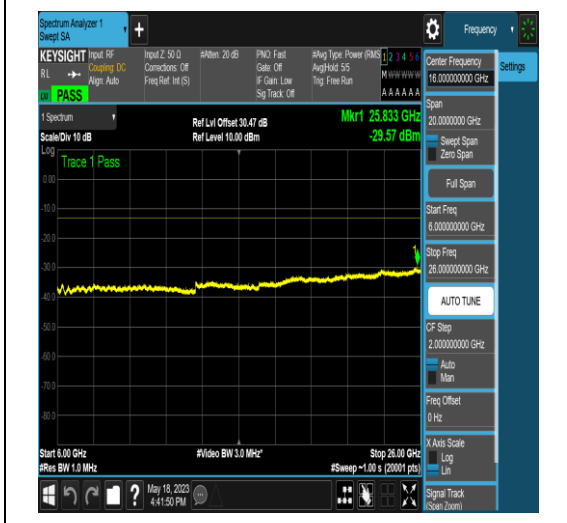
NTNV_N77-3450-3550_PC2_30_60_H_TID17_N/ A_6000_26000_#1
