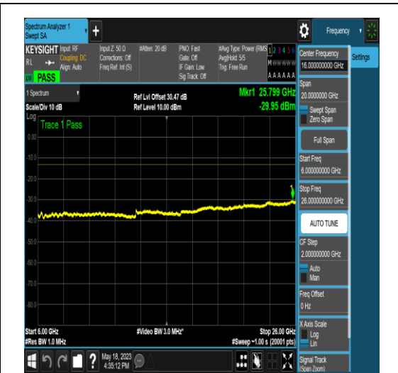
NTNV_N77-3450-3550_PC2_30_60_H_TID5_N/A _6000_26000_#1
