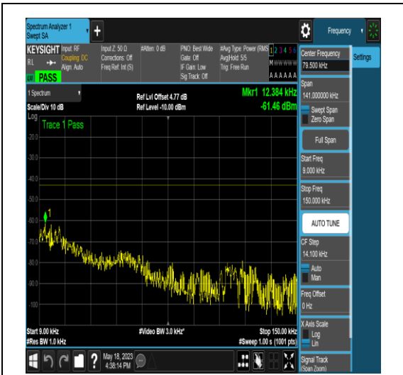
NTNV_N77-3450-3550_PC2_30_60_H_TID16_N/A_0.009_0.15_#1
