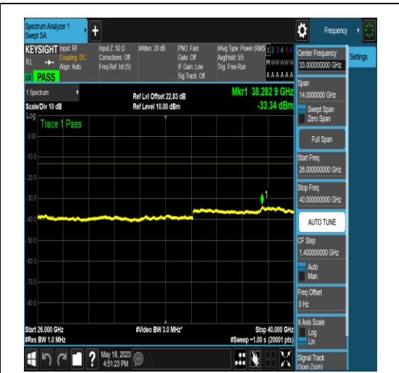
NTNV_N77-3450-3550_PC2_30_80_L_TID18_N/ A_26000_40000_#1
