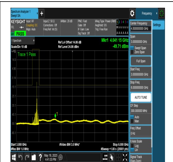
NTNV_N77-3450-3550_PC2_30_60_H_TID17_N/ A_3000_6000_#1
