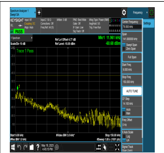
NTNV_N77-3450-3550_PC2_30_80_L_TID4_N/A _0.009_0.15_#1
