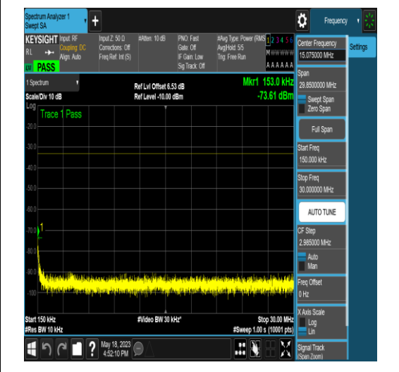
NTNV_N77-3450-3550_PC2_30_80_L_TID16_N/ A_0.15_30_#1
