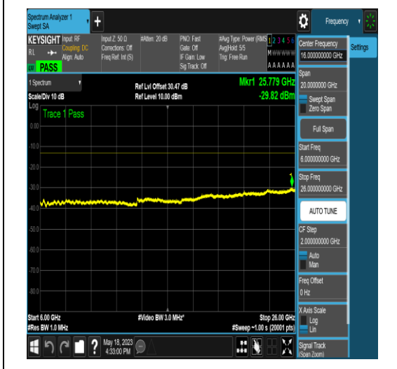
NTNV_N77-3450-3550_PC2_30_60_H_TID4_N/A _1000_3000_#1
