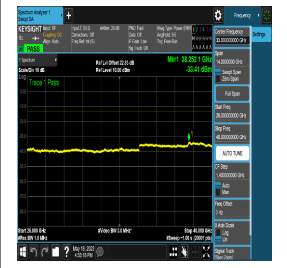
NTNV_N77-3450-3550_PC2_30_60_H_TID4_N/A _3000_6000_#1
