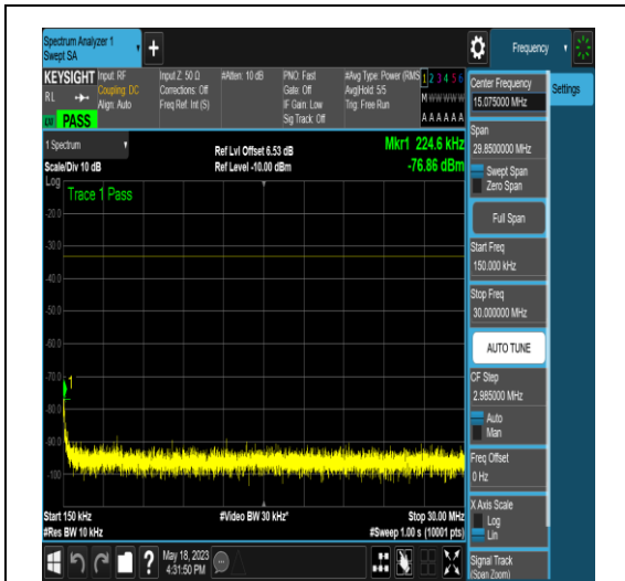
NTNV_N77-3450-3550_PC2_30_60_H_TID4_N/A _0.15_30_#1
