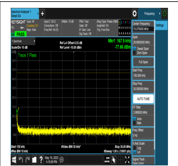
NTNV_N77-3450-3550_PC2_30_60_M_TID6_N/A _0.15_30_#1
