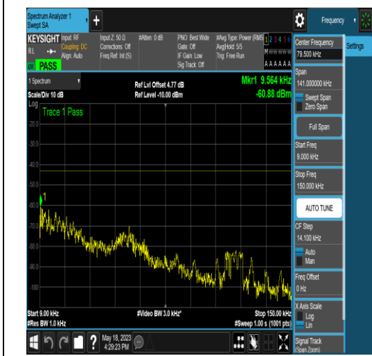
NTNV_N77-3450-3550_PC2_30_60_H_TID6_N/A_0.009_0.15_#1
