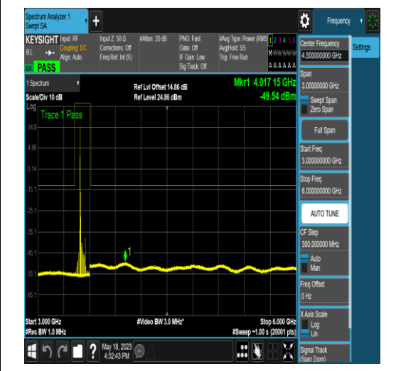
NTNV_N77-3450-3550_PC2_30_60_H_TID4_N/A _3000_6000_#1
