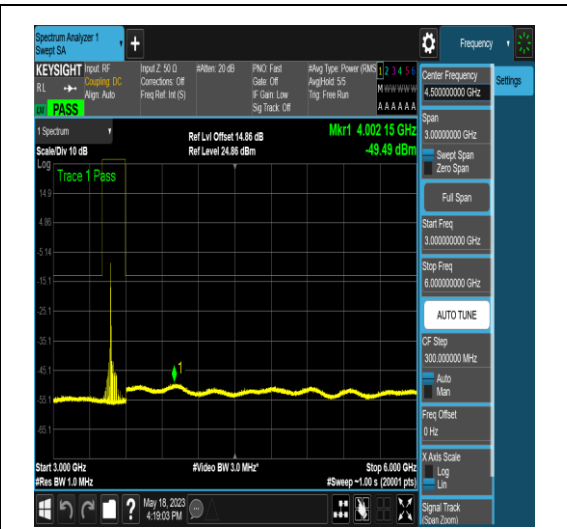
NTNV_N77-3450-3550_PC2_30_60_M_TID4_N/A _3000_6000_#1
