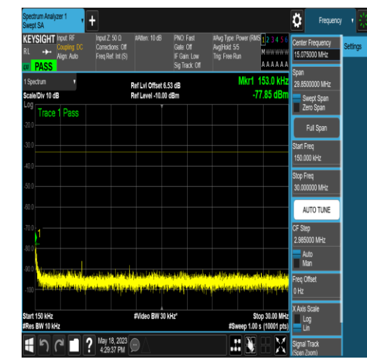
NTNV_N77-3450-3550_PC2_30_60_H_TID6_N/A_0.15_30_#1
