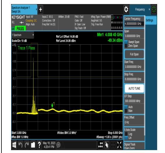
NTNV_N77-3450-3550_PC2_30_60_M_TID16_N/A_3000_6000_#1
