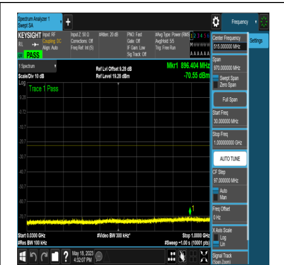
NTNV_N77-3450-3550_PC2_30_60_H_TID4_N/A _30_1000_#1
