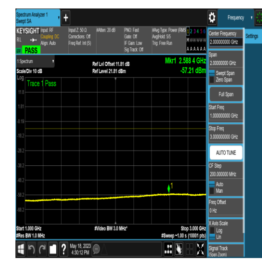
NTNV_N77-3450-3550_PC2_30_60_H_TID6_N/A_0.15_30_#1
