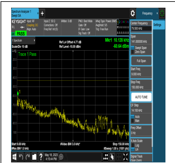
NTNV_N77-3450-3550_PC2_30_60_M_TID6_N/A _0.009_0.15_#1
