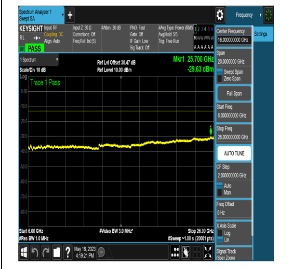
NTNV_N77-3450-3550_PC2_30_60_M_TID4_N/A _6000_26000_#1
