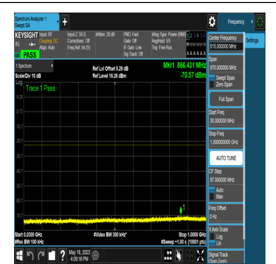
NTNV_N77-3450-3550_PC2_30_60_L_TID18_N/ A_30_1000_#1
