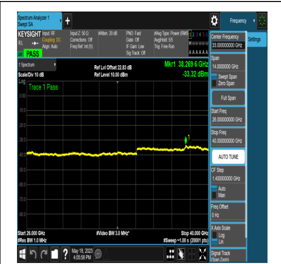
NTNV_N77-3450-3550_PC2_30_60_L_TID4_N/A _26000_40000_#1
