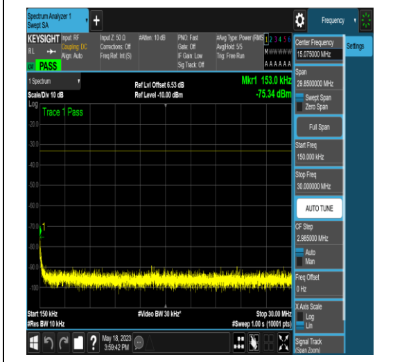
NTNV_N77-3450-3550_PC2_30_50_H_TID17_N/A_0.15_30_#1
