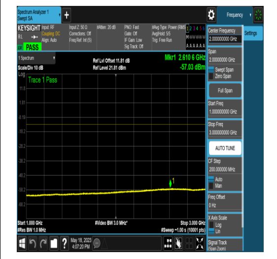
NTNV_N77-3450-3550_PC2_30_60_L_TID5_N/A _0.15_30_#1
