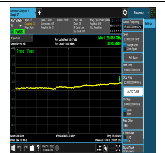
NTNV_N77-3450-3550_PC2_30_50_H_TID6_N/A _6000_26000_#1
