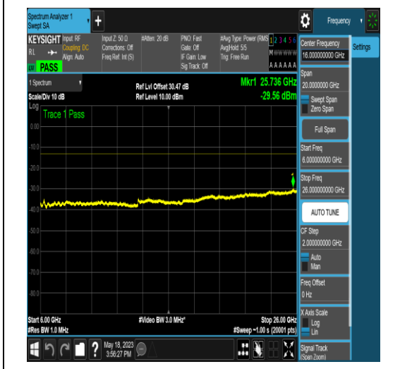
NTNV_N77-3450-3550_PC2_30_50_H_TID18_N/A_6000_26000_#1
