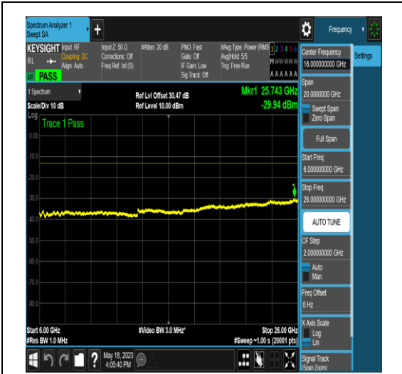
NTNV_N77-3450-3550_PC2_30_60_L_TID4_N/A _6000_26000_#1
