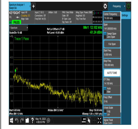
NTNV_N77-3450-3550_PC2_30_60_L_TID5_N/A _0.009_0.15_#1
