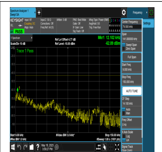
NTNV_N77-3450-3550_PC2_30_50_H_TID17_N/A_0.009_0.15_#1
