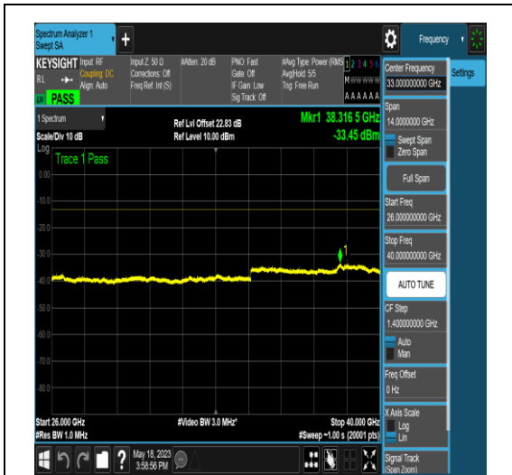
NTNV_N77-3450-3550_PC2_30_50_H_TID16_N/A_26000_40000_#1
