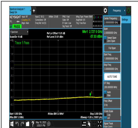
NTNV_N77-3450-3550_PC2_30_50_H_TID18_N/A_1000_3000_#1
