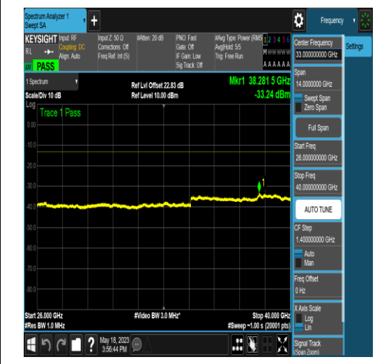
NTNV_N77-3450-3550_PC2_30_50_H_TID18_N/A_26000_40000_#1
