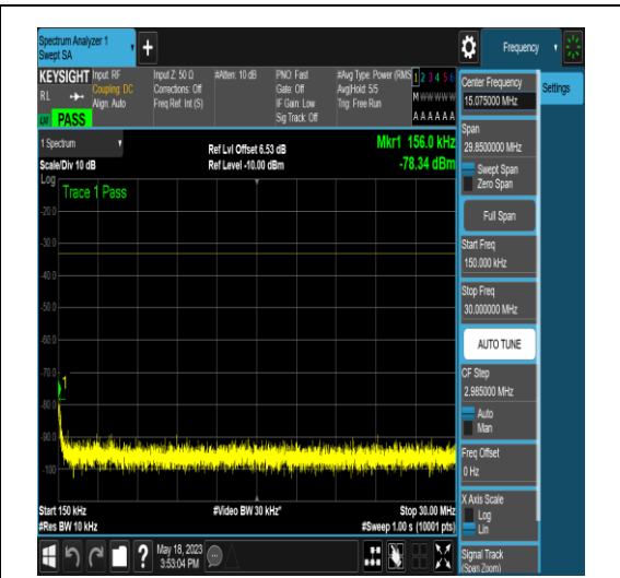
NTNV_N77-3450-3550_PC2_30_50_H_TID5_N/A _0.15_30_#1
