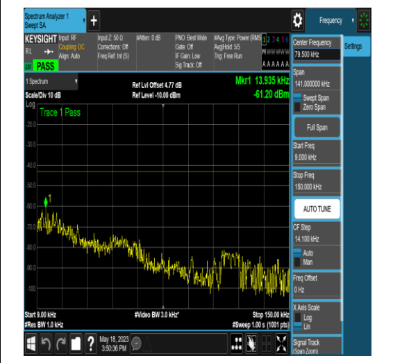
NTNV_N77-3450-3550_PC2_30_50_H_TID4_N/A _0.009_0.15_#1
