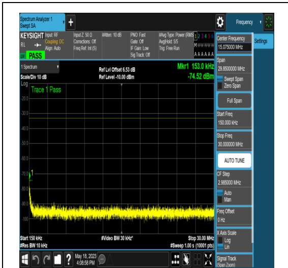
NTNV_N77-3450-3550_PC2_30_60_L_TID18_N/ A_0.15_30_#1
