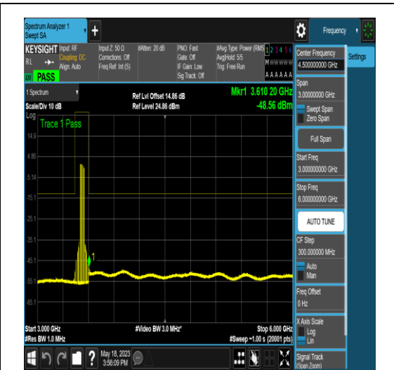
NTNV_N77-3450-3550_PC2_30_50_H_TID18_N/A_3000_6000_#1
