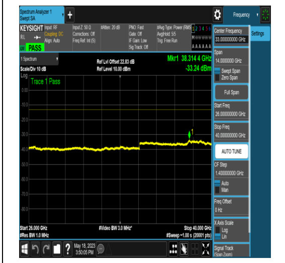
NTNV_N77-3450-3550_PC2_30_50_H_TID6_N/A _26000_40000_#1
