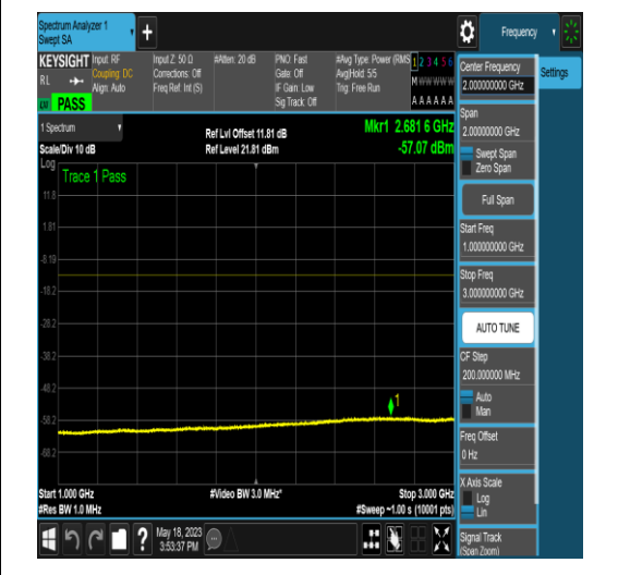
NTNV_N77-3450-3550_PC2_30_50_H_TID5_N/A _1000_3000_#1
