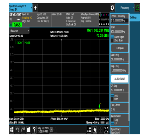
NTNV_N77-3450-3550_PC2_30_50_H_TID17_N/A_30_1000_#1
