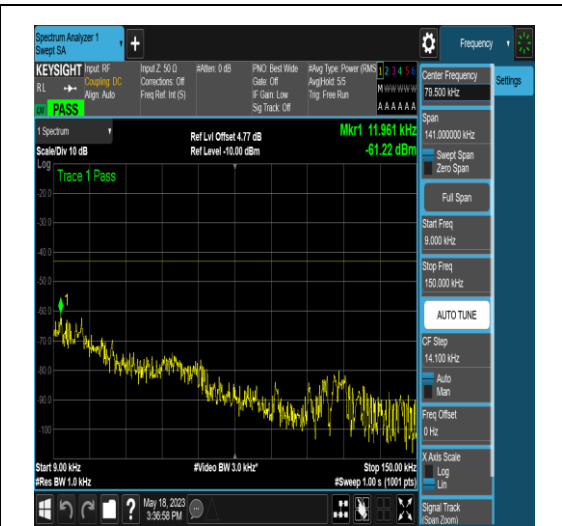
NTNV_N77-3450-3550_PC2_30_50_M_TID4_N/A _0.009_0.15_#1
