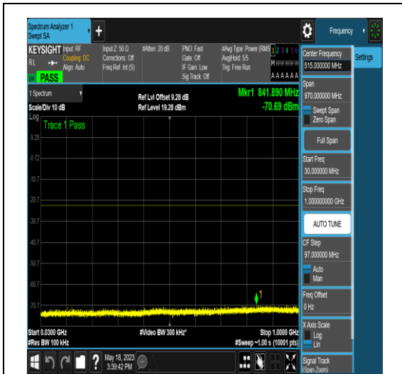
NTNV_N77-3450-3550_PC2_30_50_M_TID5_N/A _30_1000_#1
