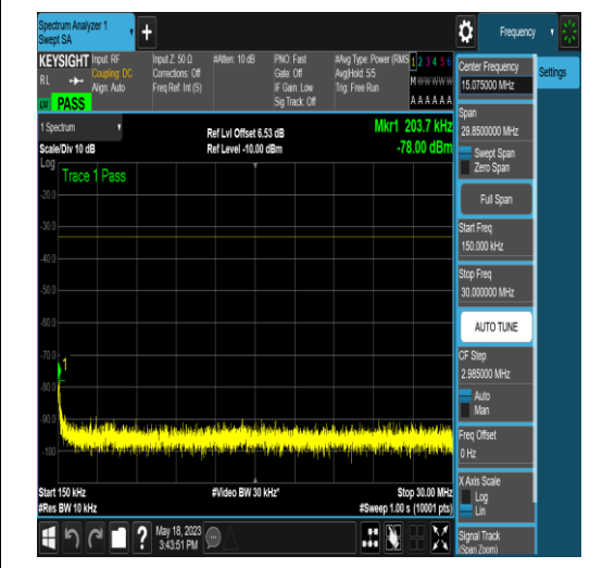
NTNV_N77-3450-3550_PC2_30_50_M_TID16_N/ A_0.15_30_#1
