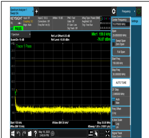
NTNV_N77-3450-3550_PC2_30_50_M_TID17_N/ A_0.15_30_#1
