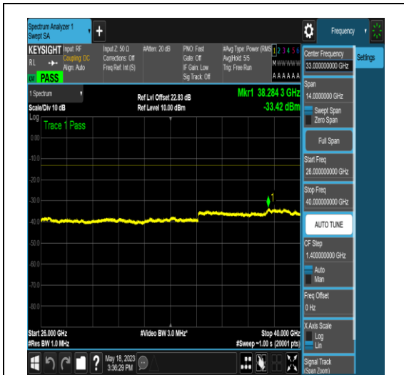
NTNV_N77-3450-3550_PC2_30_50_M_TID6_N/A _26000_40000_#1
