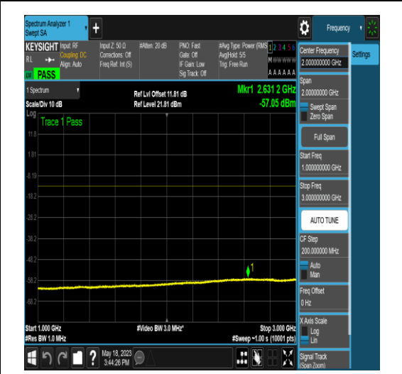
NTNV_N77-3450-3550_PC2_30_50_M_TID16_N/ A_0.15_30_#1
