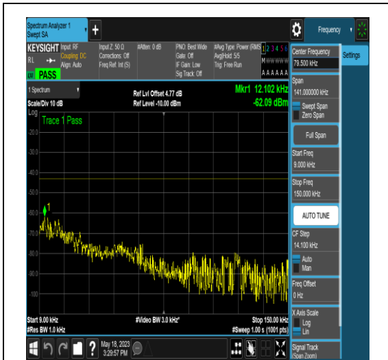
NTNV_N77-3450-3550_PC2_30_50_L_TID16_N/ A_0.009_0.15_#1
