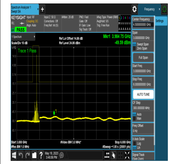
NTNV_N77-3450-3550_PC2_30_50_M_TID17_N/ A_3000_6000_#1
