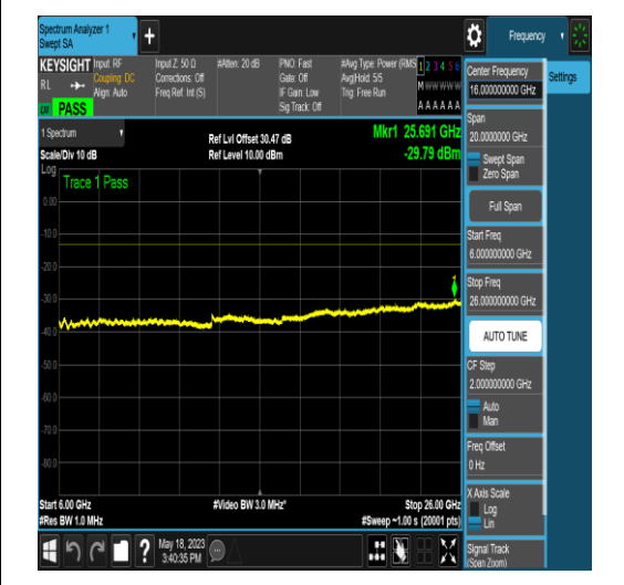
NTNV_N77-3450-3550_PC2_30_50_M_TID5_N/A _6000_26000_#1
