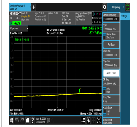
NTNV_N77-3450-3550_PC2_30_50_M_TID17_N/ A_1000_3000_#1
