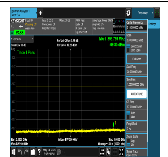
NTNV_N77-3450-3550_PC2_30_50_M_TID17_N/ A_30_1000_#1
