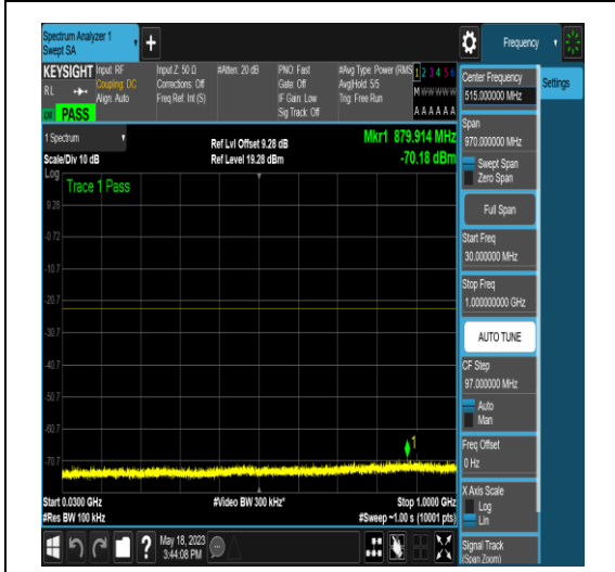
NTNV_N77-3450-3550_PC2_30_50_M_TID16_N/ A_0.009_0.15_#1
