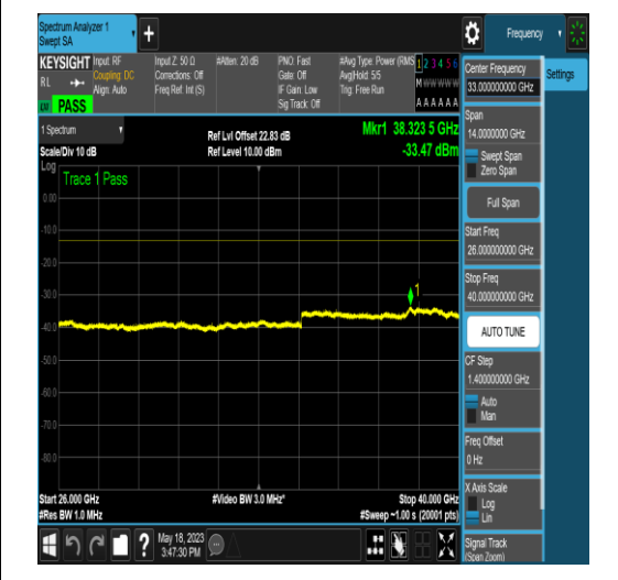
NTNV_N77-3450-3550_PC2_30_50_M_TID17_N/ A_3000_6000_#1
