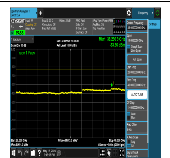
NTNV_N77-3450-3550_PC2_30_50_M_TID18_N/ A_26000_40000_#1
