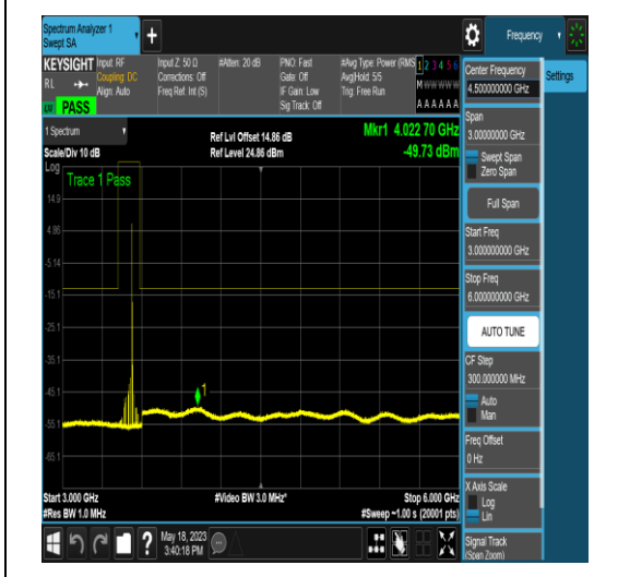
NTNV_N77-3450-3550_PC2_30_50_M_TID5_N/A _3000_6000_#1
