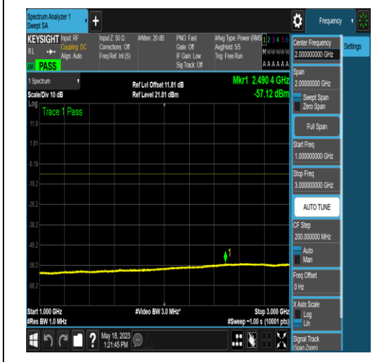
NTNV_N77-3450-3550_PC2_30_15_L_TID4_N/A _0.15_30_#1
