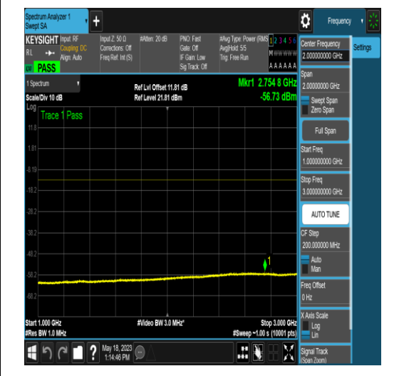
NTNV_N77-3450-3550_PC2_30_10_H_TID16_N/A_1000_3000_#1
