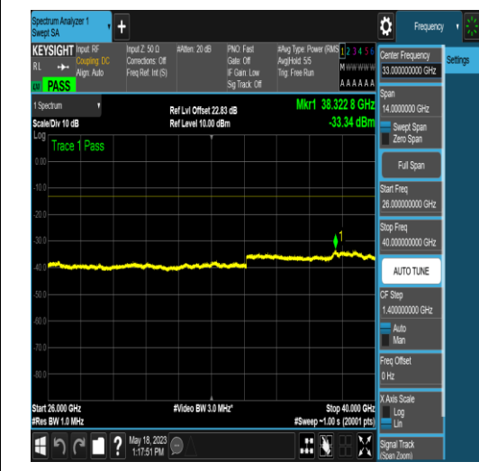
NTNV_N77-3450-3550_PC2_30_10_H_TID17_N/ A_26000_40000_#1
