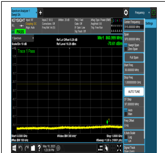
NTNV_N77-3450-3550_PC2_30_15_L_TID5_N/A _30_1000_#1
