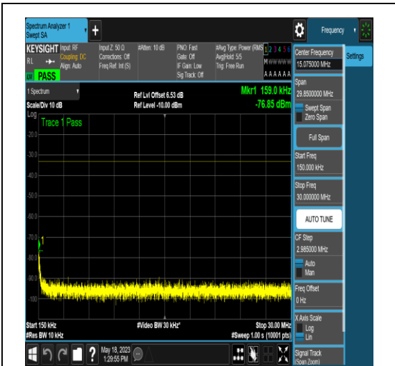
NTNV_N77-3450-3550_PC2_30_15_L_TID17_N/ A_0.15_30_#1
