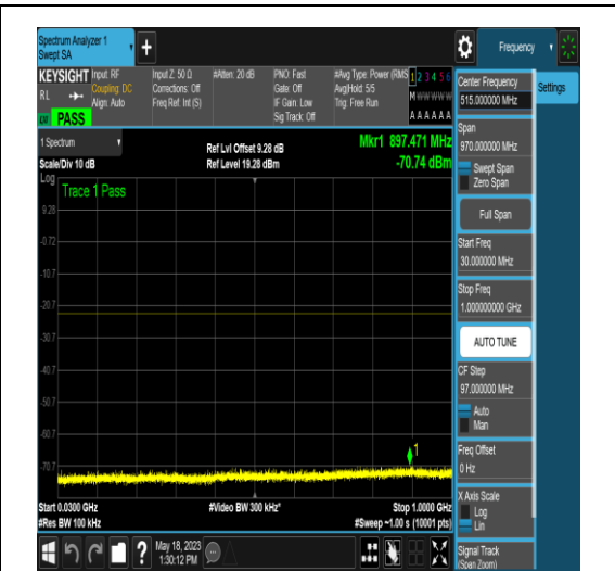
NTNV_N77-3450-3550_PC2_30_15_L_TID17_N/ A_30_1000_#1
