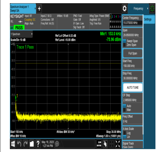
NTNV_N77-3450-3550_PC2_30_15_L_TID16_N/ A_0.15_30_#1
