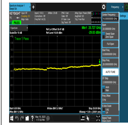
NTNV_N77-3450-3550_PC2_30_10_H_TID17_N/ A_6000_26000_#1
