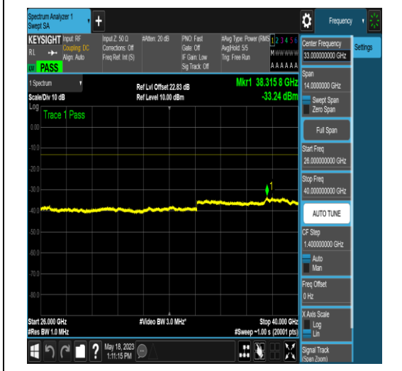
NTNV_N77-3450-3550_PC2_30_10_H_TID5_N/A _26000_40000_#1
