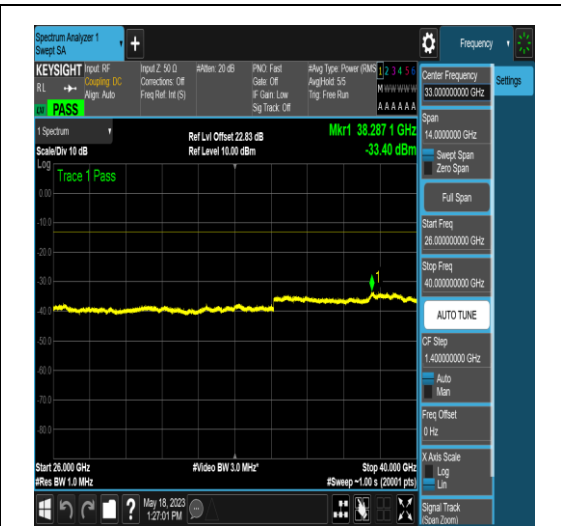
NTNV_N77-3450-3550_PC2_30_15_L_TID18_N/ A_26000_40000_#1
