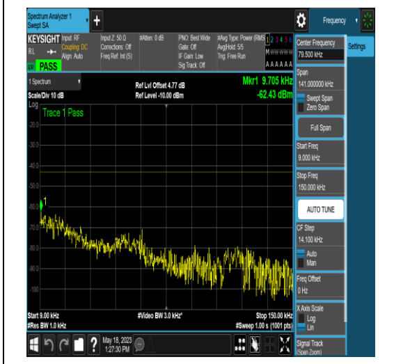
NTNV_N77-3450-3550_PC2_30_15_L_TID16_N/ A_0.009_0.15_#1
