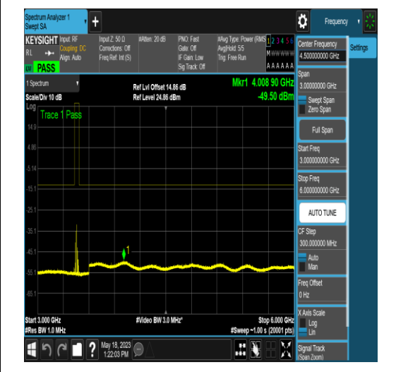
NTNV_N77-3450-3550_PC2_30_15_L_TID4_N/A _30_1000_#1
