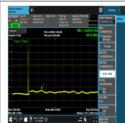
NTNV_N77-3450-3550_PC2_30_10_H_TID17_N/ A_3000_6000_#1
