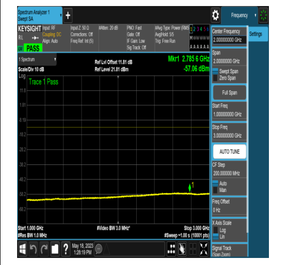
NTNV_N77-3450-3550_PC2_30_15_L_TID16_N/ A_0.15_30_#1
