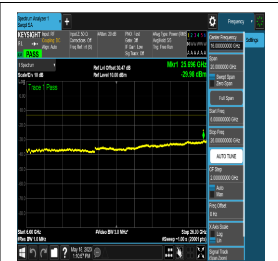
NTNV_N77-3450-3550_PC2_30_10_H_TID5_N/A _6000_26000_#1
