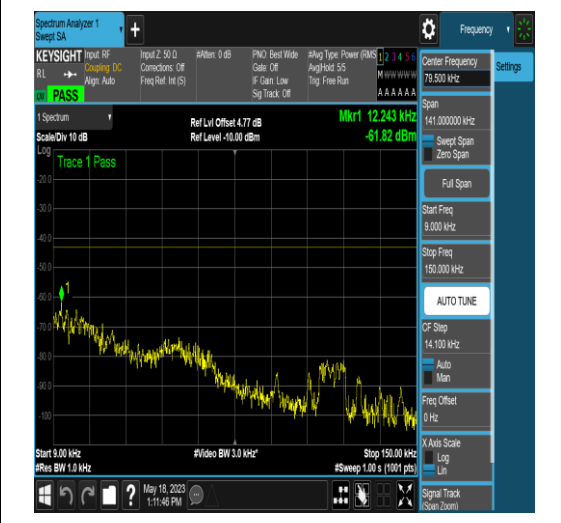
NTNV_N77-3450-3550_PC2_30_10_H_TID18_N/ A_0.009_0.15_#1
