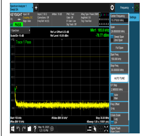
NTNV_N77-3450-3550_PC2_30_15_L_TID4_N/A _0.15_30_#1
