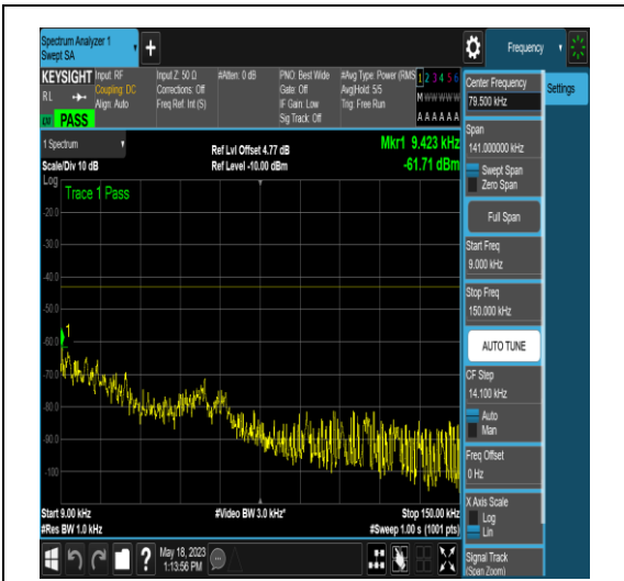
NTNV_N77-3450-3550_PC2_30_10_H_TID16_N/A_0.009_0.15_#1
