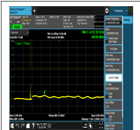
NTNV_N77-3450-3550_PC2_30_10_H_TID5_N/A _3000_6000_#1
