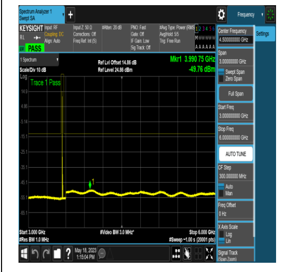
NTNV_N77-3450-3550_PC2_30_10_H_TID16_N/A_30_1000_#1
