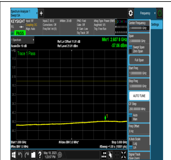
NTNV_N77-3450-3550_PC2_30_15_L_TID5_N/A _1000_3000_#1
