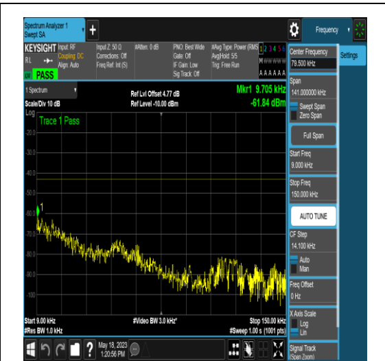
NTNV_N77-3450-3550_PC2_30_15_L_TID4_N/A _0.009_0.15_#1
