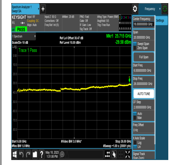
NTNV_N77-3450-3550_PC2_30_15_L_TID17_N/ A_1000_3000_#1
