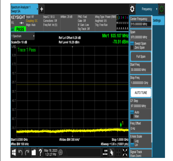
NTNV_N77-3450-3550_PC2_30_15_L_TID4_N/A _30_1000_#1
