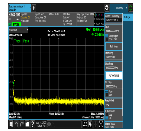
NTNV_N77-3450-3550_PC2_30_10_H_TID6_N/A_0.15_30_#1
