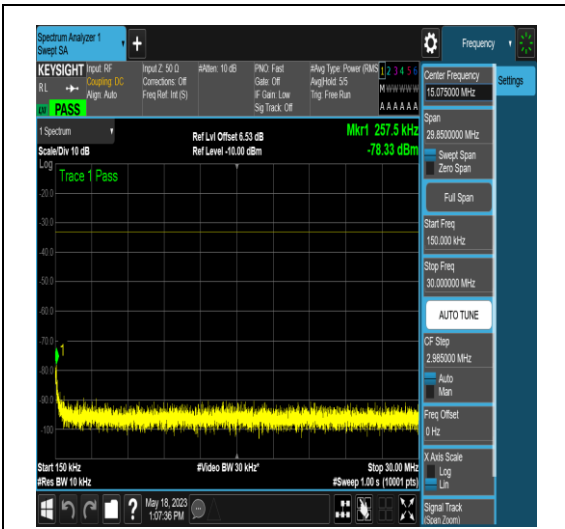
NTNV_N77-3450-3550_PC2_30_10_H_TID4_N/A _0.15_30_#1
