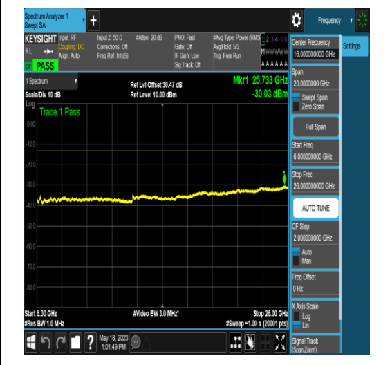
NTNV_N77-3450-3550_PC2_30_10_M_TID16_N/ A_6000_26000_#1
