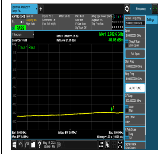
NTNV_N77-3450-3550_PC2_30_10_M_TID18_N/A_0.15_30_#1
