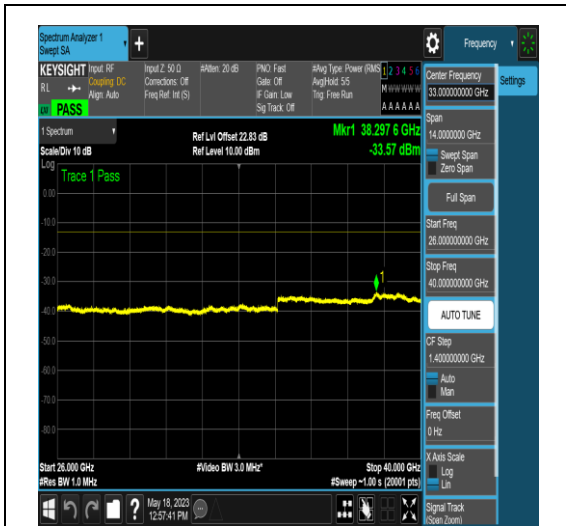
NTNV_N77-3450-3550_PC2_30_10_M_TID5_N/A_26000_40000_#1
