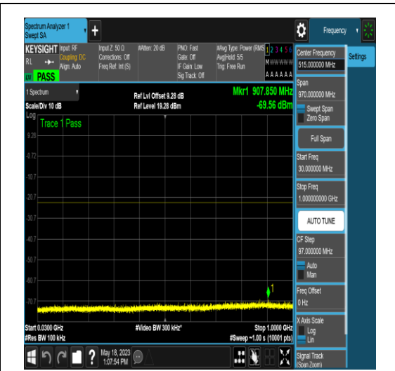
NTNV_N77-3450-3550_PC2_30_10_H_TID4_N/A _30_1000_#1
