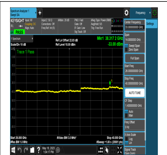
NTNV_N77-3450-3550_PC2_30_10_M_TID17_NV_A_26000_40000_#1
