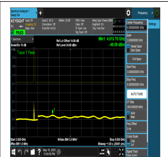
NTNV_N77-3450-3550_PC2_30_10_M_TID4_N/A _3000_6000_#1
