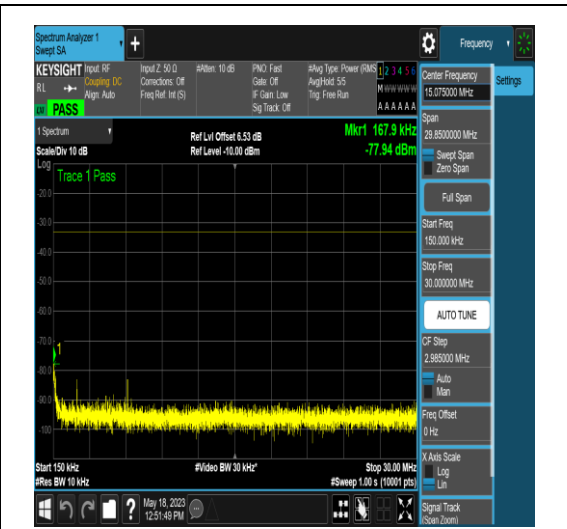
NTNV_N77-3450-3550_PC2_30_10_M_TID6_N/A _0.15_30_#1
