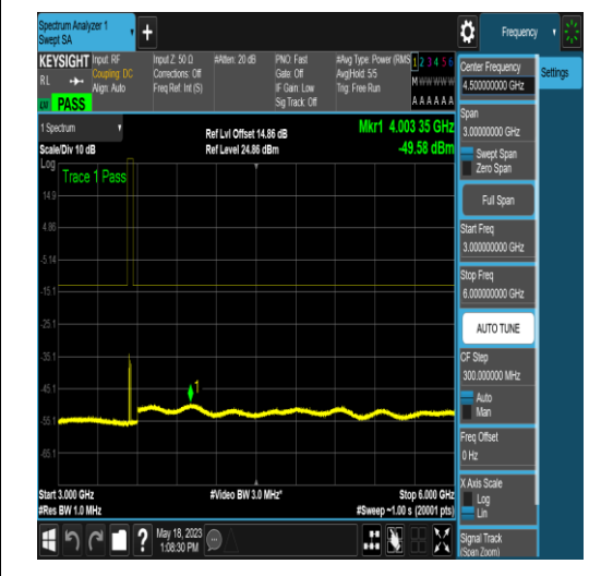
NTNV_N77-3450-3550_PC2_30_10_H_TID4_N/A _3000_6000_#1
