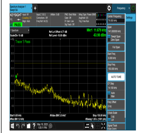
NTNV_N77-3450-3550_PC2_30_10_H_TID6_N/A_0.009_0.15_#1
