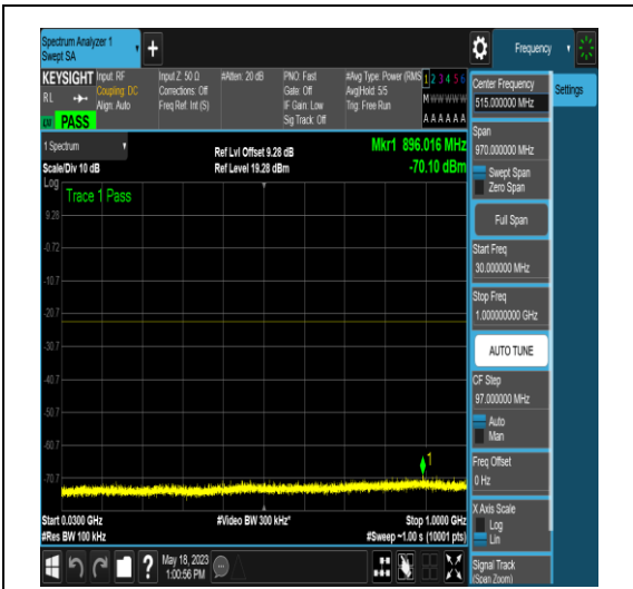
NTNV_N77-3450-3550_PC2_30_10_M_TID16_N/ A_30_1000_#1
