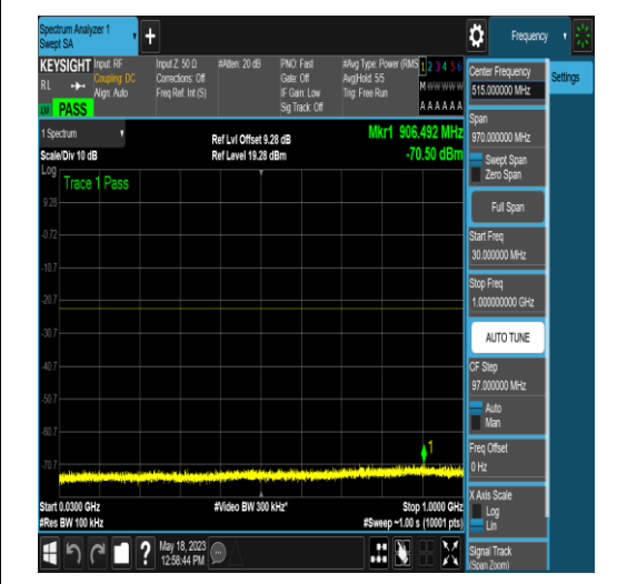
NTNV_N77-3450-3550_PC2_30_10_M_TID18_N/A_30_1000_#1
