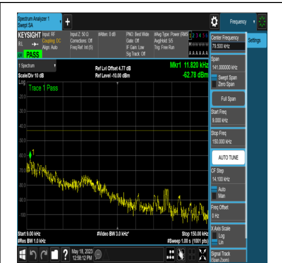
NTNV_N77-3450-3550_PC2_30_10_M_TID18_N/A_0.009_0.15_#1
