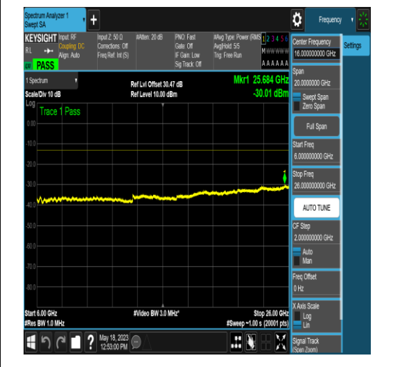
NTNV_N77-3450-3550_PC2_30_10_M_TID6_N/A _1000_3000_#1
