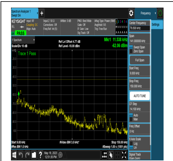
NTNV_N77-3450-3550_PC2_30_10_M_TID6_N/A _0.009_0.15_#1
