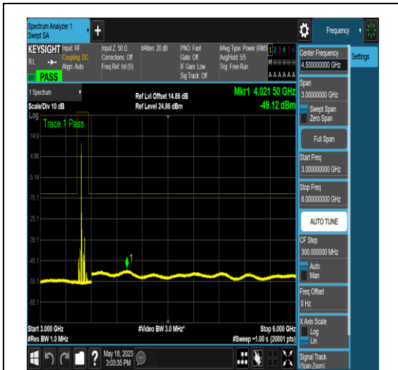
NTNV_N77-3450-3550_PC2_30_40_M_TID16_N/ A_3000_6000_#1
