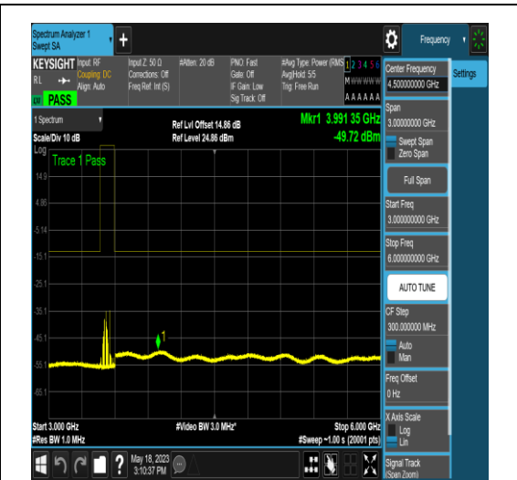
NTNV_N77-3450-3550_PC2_30_40_H_TID4_N/A _3000_6000_#1
