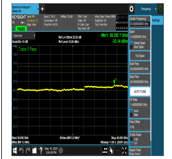
NTNV_N77-3450-3550_PC2_30_40_M_TID16_N/ A_26000_40000_#1
