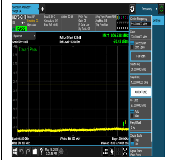
NTNV_N77-3450-3550_PC2_30_40_H_TID6_N/A _30_1000_#1
