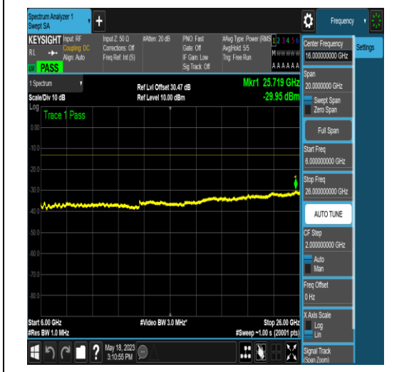
NTNV_N77-3450-3550_PC2_30_40_H_TID4_N/A _6000_26000_#1
