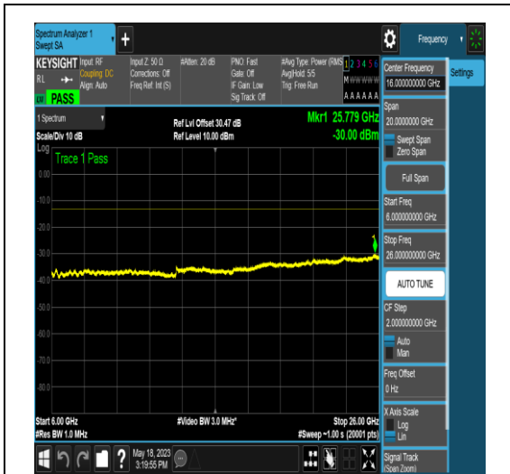
NTNV_N77-3450-3550_PC2_30_40_H_TID17_N/A_6000_26000_#1
