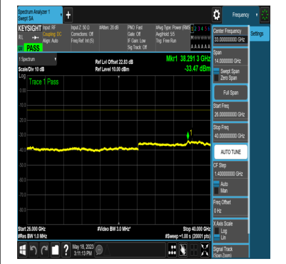
NTNV_N77-3450-3550_PC2_30_40_H_TID4_N/A _26000_40000_#1
