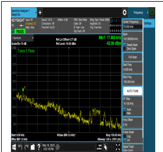
NTNV_N77-3450-3550_PC2_30_40_H_TID6_N/A _0.009_0.15_#1
