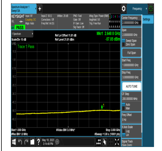
NTNV_N77-3450-3550_PC2_30_40_H_TID18_N/ A_0.15_30_#1
