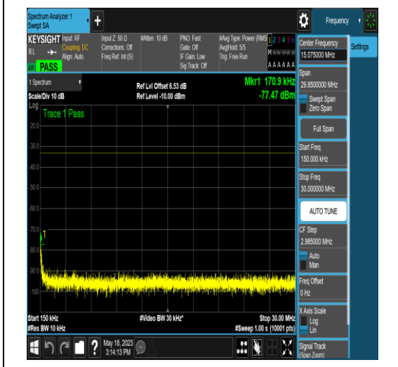
NTNV_N77-3450-3550_PC2_30_40_H_TID18_N/ A_0.15_30_#1
