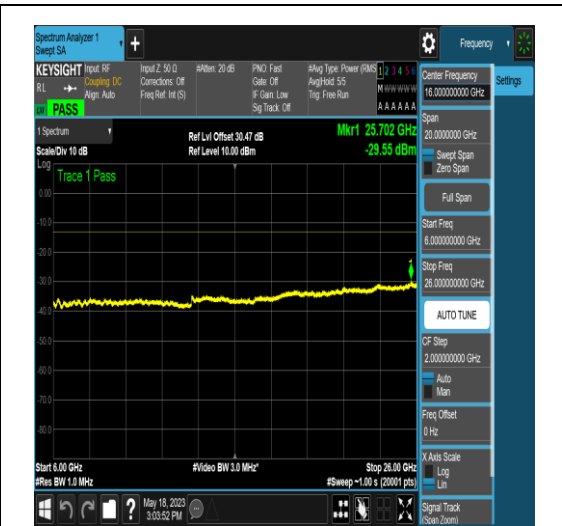
NTNV_N77-3450-3550_PC2_30_40_M_TID16_N/ A_6000_26000_#1
