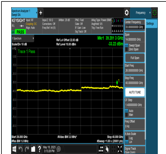
NTNV_N77-3450-3550_PC2_30_40_H_TID5_N/A _26000_40000_#1
