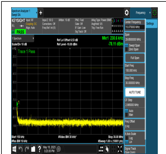
NTNV_N77-3450-3550_PC2_30_50_L_TID4_N/A _0.15_30_#1
