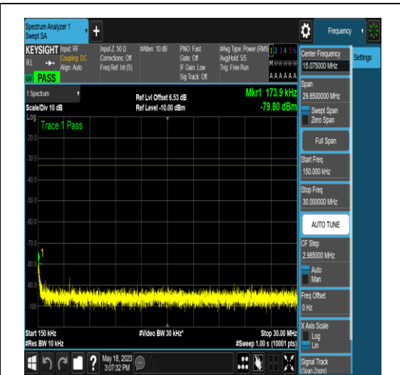
NTNV_N77-3450-3550_PC2_30_40_H_TID6_N/A _0.15_30_#1
