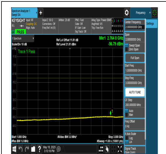
NTNV_N77-3450-3550_PC2_30_40_H_TID4_N/A _1000_3000_#1
