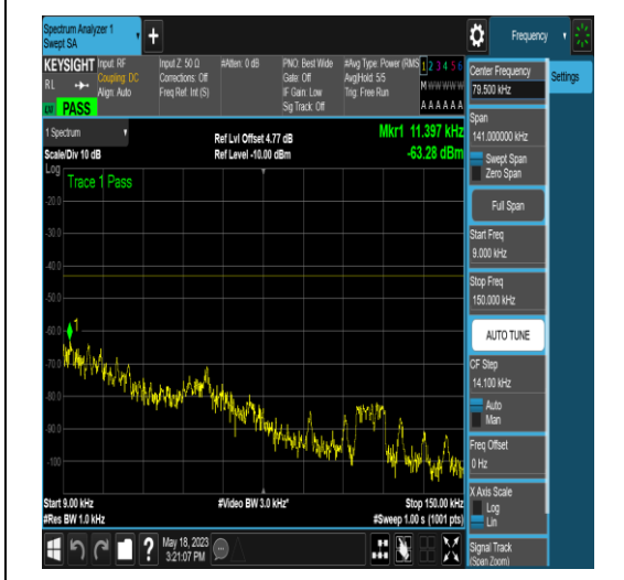
NTNV_N77-3450-3550_PC2_30_50_L_TID6_N/A_0.009_0.15_#1
