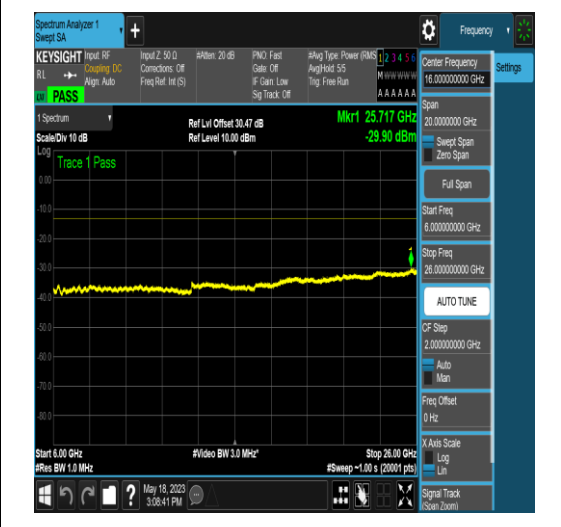
NTNV_N77-3450-3550_PC2_30_40_H_TID6_N/A _1000_3000_#1
