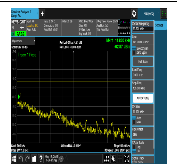
NTNV_N77-3450-3550_PC2_30_40_H_TID18_N/ A_0.009_0.15_#1
