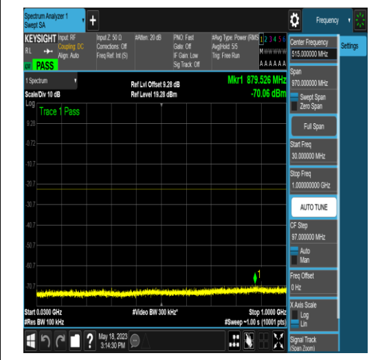
NTNV_N77-3450-3550_PC2_30_40_H_TID18_N/ A_30_1000_#1
