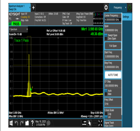
NTNV_N77-3450-3550_PC2_30_40_H_TID18_N/ A_30_1000_#1
