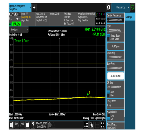
NTNV_N77-3450-3550_PC2_30_40_H_TID6_N/A _1000_3000_#1
