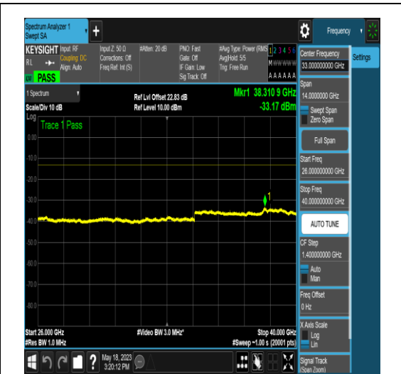
NTNV_N77-3450-3550_PC2_30_40_H_TID17_N/A_26000_40000_#1
