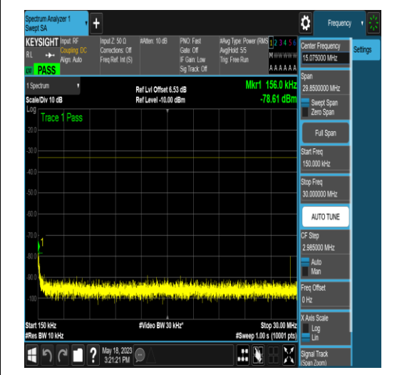
NTNV_N77-3450-3550_PC2_30_50_L_TID6_N/A_0.15_30_#1
