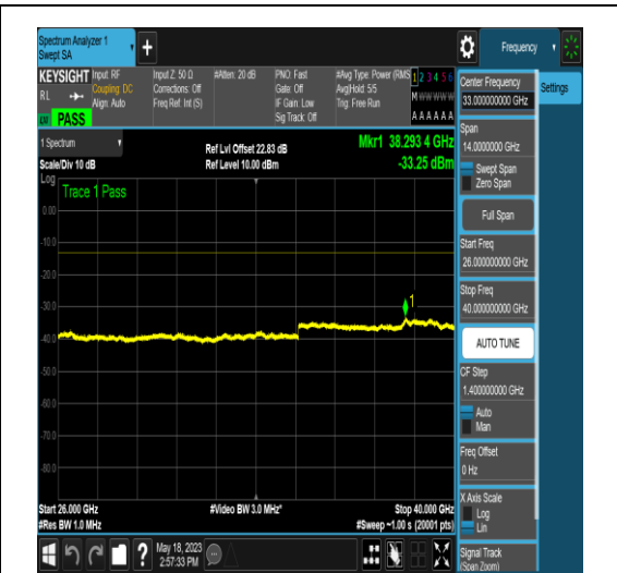
NTNV_N77-3450-3550_PC2_30_40_M_TID4_N/A _26000_40000_#1
