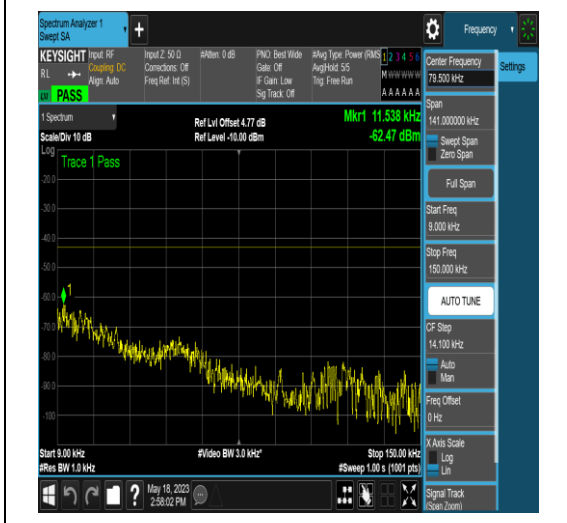
NTNV_N77-3450-3550_PC2_30_40_M_TID5_N/A _0.009_0.15_#1
