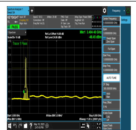
NTNV_N77-3450-3550_PC2_30_40_L_TID18_N/A_3000_6000_#1
