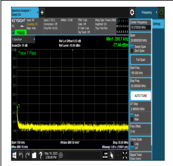
NTNV_N77-3450-3550_PC2_30_40_M_TID4_N/A _0.15_30_#1
