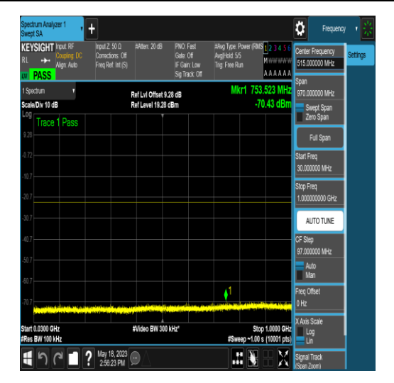
NTNV_N77-3450-3550_PC2_30_40_M_TID4_N/A _30_1000_#1
