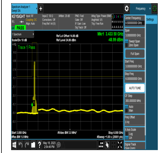
NTNV_N77-3450-3550_PC2_30_40_M_TID6_N/A _3000_6000_#1
