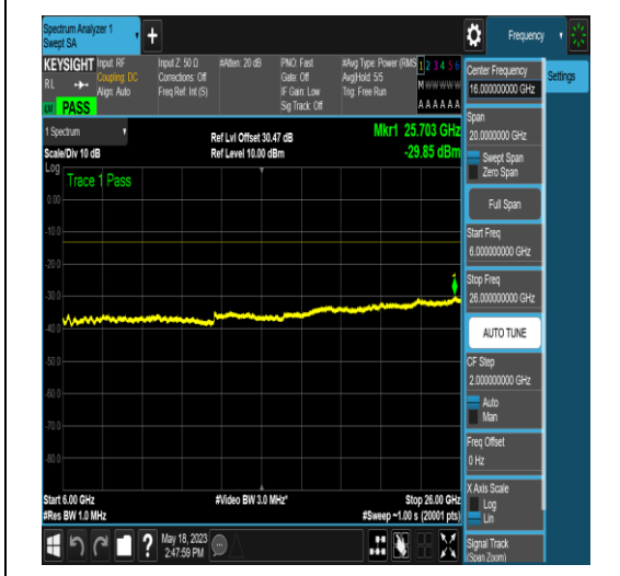
NTNV_N77-3450-3550_PC2_30_40_L_TID18_N/A_6000_26000_#1
