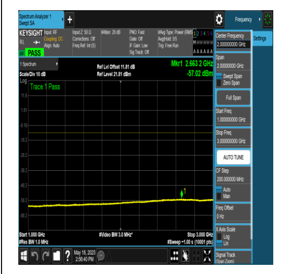
NTNV_N77-3450-3550_PC2_30_40_M_TID4_N/A _1000_3000_#1
