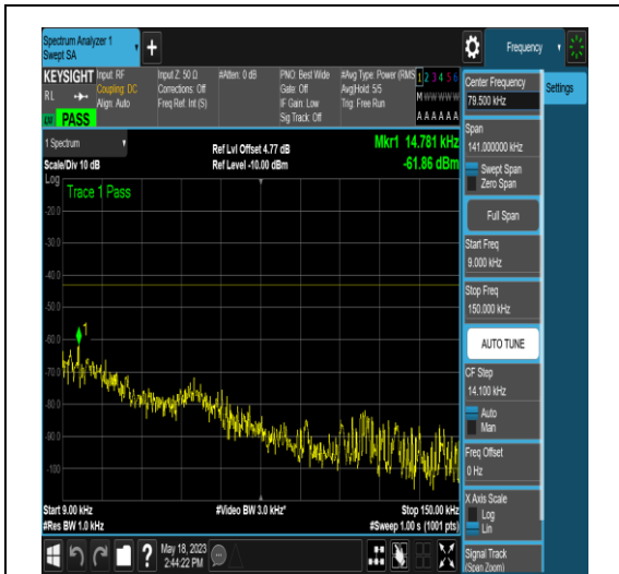
NTNV_N77-3450-3550_PC2_30_40_L_TID5_N/A _0.009_0.15_#1
