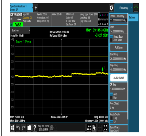
NTNV_N77-3450-3550_PC2_30_40_M_TID6_N/A _3000_6000_#1
