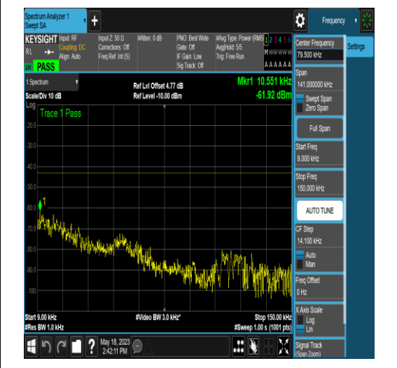
NTNV_N77-3450-3550_PC2_30_40_L_TID4_N/A _0.009_0.15_#1
