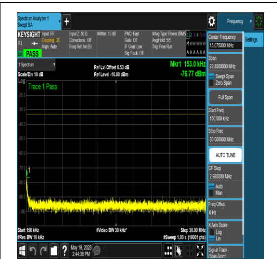
NTNV_N77-3450-3550_PC2_30_40_L_TID5_N/A _0.15_30_#1
