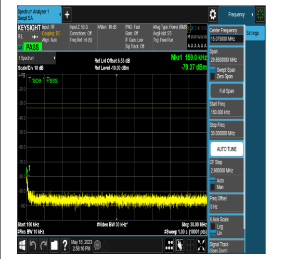
NTNV_N77-3450-3550_PC2_30_40_M_TID5_N/A _0.15_30_#1
