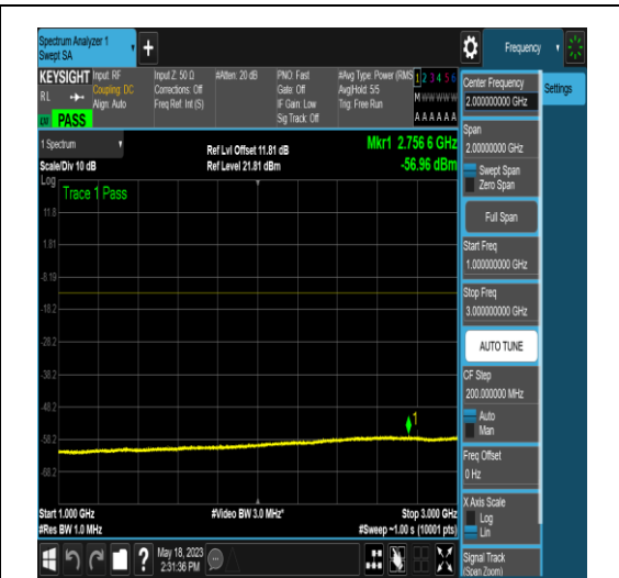
NTNV_N77-3450-3550_PC2_30_20_H_TID5_N/A _1000_3000_#1
