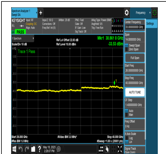
NTNV_N77-3450-3550_PC2_30_20_H_TID6_N/A _26000_40000_#1
