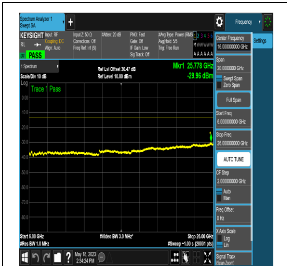
NTNV_N77-3450-3550_PC2_30_20_H_TID18_N/A_6000_26000_#1
