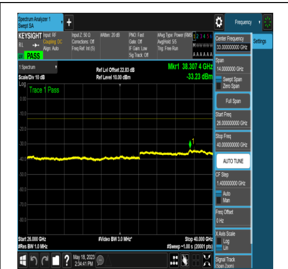
NTNV_N77-3450-3550_PC2_30_20_H_TID18_N/A_26000_40000_#1
