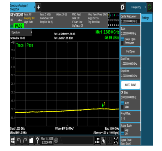
NTNV_N77-3450-3550_PC2_30_20_M_TID16_N/ A_1000_3000_#1
