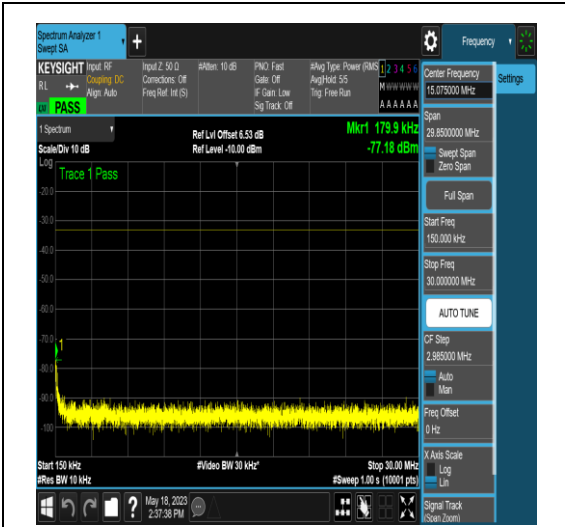
NTNV_N77-3450-3550_PC2_30_20_H_TID17_N/ A_0.15_30_#1
