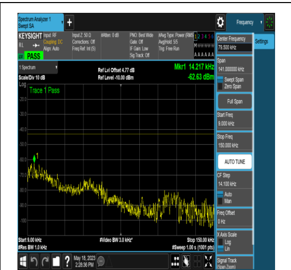
NTNV_N77-3450-3550_PC2_30_20_H_TID4_N/A _0.009_0.15_#1
