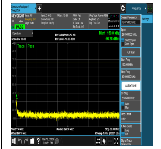
NTNV_N77-3450-3550_PC2_30_20_H_TID4_N/A _0.15_30_#1
