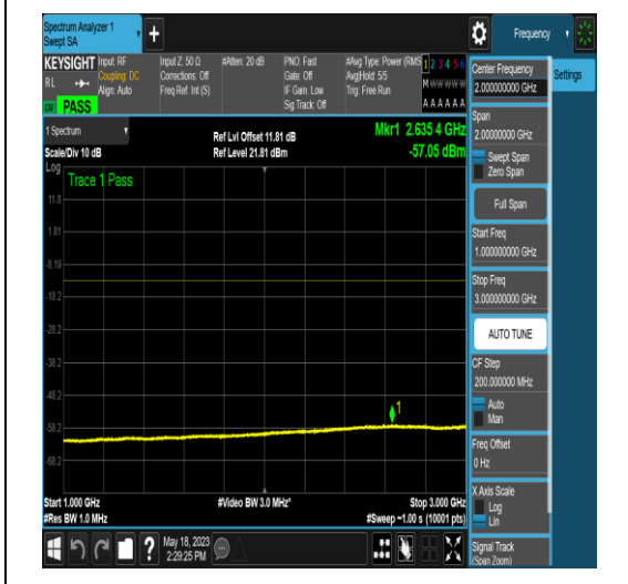
NTNV_N77-3450-3550_PC2_30_20_H_TID4_N/A _0.15_30_#1
