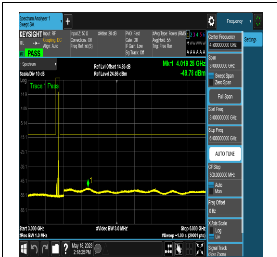
NTNV_N77-3450-3550_PC2_30_20_M_TID5_N/A _3000_6000_#1
