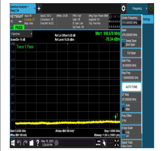
NTNV_N77-3450-3550_PC2_30_20_H_TID4_N/A _30_1000_#1
