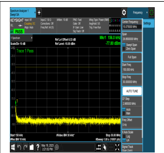
NTNV_N77-3450-3550_PC2_30_20_M_TID16_N/ A_0.15_30_#1
