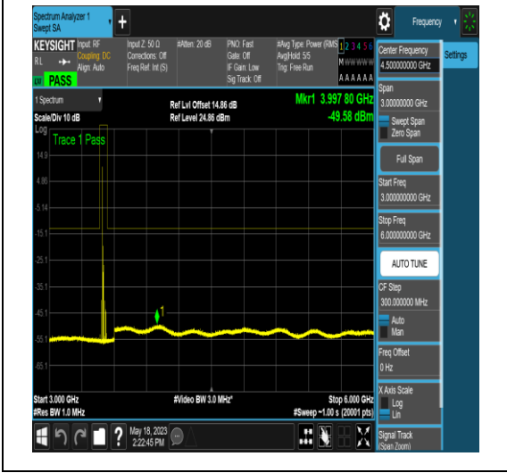
NTNV_N77-3450-3550_PC2_30_20_M_TID16_N/ A_30_1000_#1
