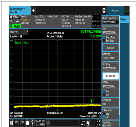
NTNV_N77-3450-3550_PC2_30_20_H_TID5_N/A _30_1000_#1
