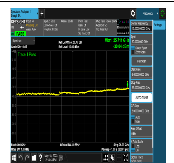
NTNV_N77-3450-3550_PC2_30_20_M_TID5_N/A _6000_26000_#1
