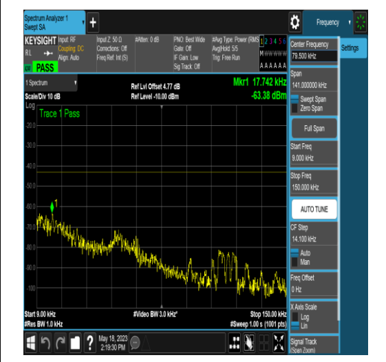
NTNV_N77-3450-3550_PC2_30_20_M_TID18_N/ A_0.009_0.15_#1
