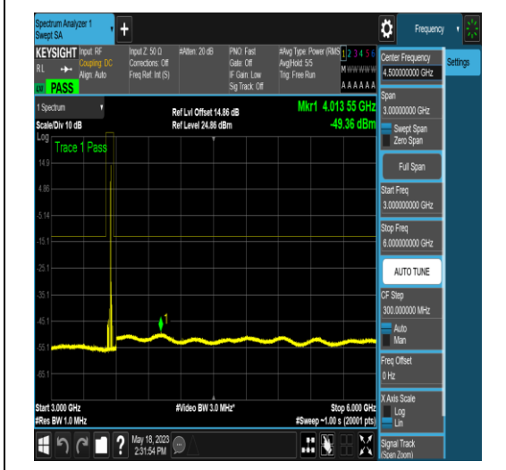
NTNV_N77-3450-3550_PC2_30_20_H_TID5_N/A _3000_6000_#1
