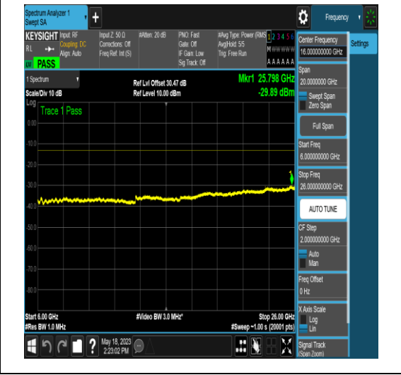
NTNV_N77-3450-3550_PC2_30_20_M_TID16_N/ A_1000_3000_#1
