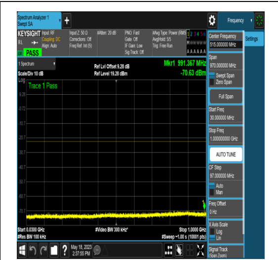
NTNV_N77-3450-3550_PC2_30_20_H_TID17_N/ A_30_1000_#1
