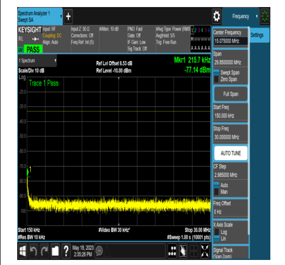
NTNV_N77-3450-3550_PC2_30_20_H_TID16_N/A_0.15_30_#1
