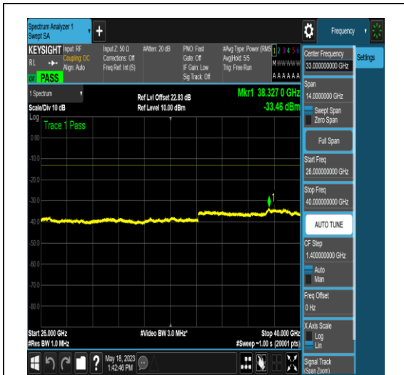
NTNV_N77-3450-3550_PC2_30_15_M_TID16_N/A_26000_40000_#1
