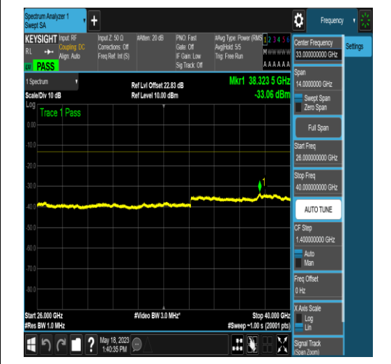
NTNV_N77-3450-3550_PC2_30_15_M_TID18_N/ A_26000_40000_#1
