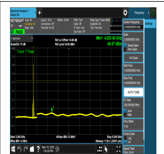
NTNV_N77-3450-3550_PC2_30_15_M_TID18_N/ A_3000_6000_#1
