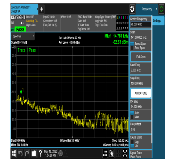
NTNV_N77-3450-3550_PC2_30_15_M_TID4_N/A _0.009_0.15_#1
