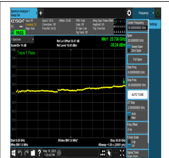
NTNV_N77-3450-3550_PC2_30_15_M_TID6_N/A _6000_26000_#1
