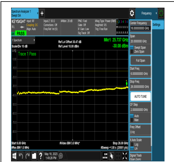
NTNV_N77-3450-3550_PC2_30_15_H_TID4_N/A _6000_26000_#1
