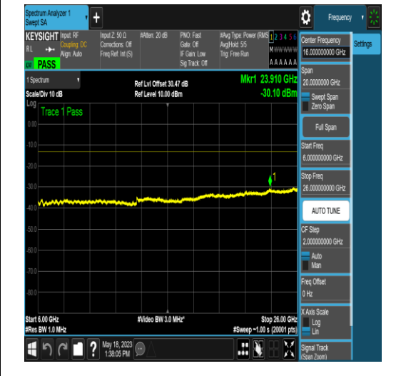
NTNV_N77-3450-3550_PC2_30_15_M_TID5_N/A _1000_3000_#1
