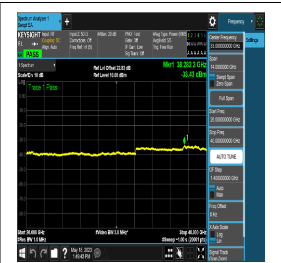
NTNV_N77-3450-3550_PC2_30_15_H_TID4_N/A _26000_40000_#1
