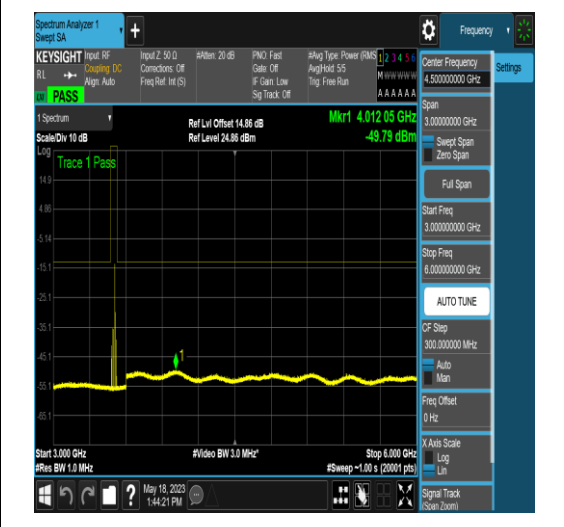
NTNV_N77-3450-3550_PC2_30_15_M_TID17_N/A_30_1000_#1
