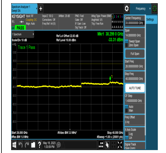
NTNV_N77-3450-3550_PC2_30_15_M_TID6_N/A _26000_40000_#1
