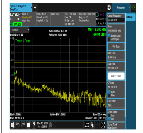
NTNV_N77-3450-3550_PC2_30_15_M_TID18_N/ A_6000_26000_#1
