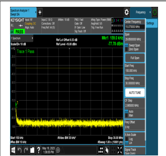
NTNV_N77-3450-3550_PC2_30_15_M_TID5_N/A _0.15_30_#1
