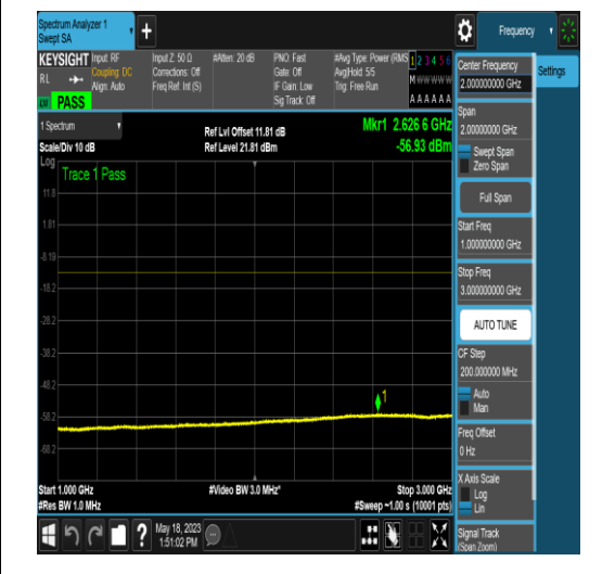
NTNV_N77-3450-3550_PC2_30_15_H_TID5_N/A _0.15_30_#1
