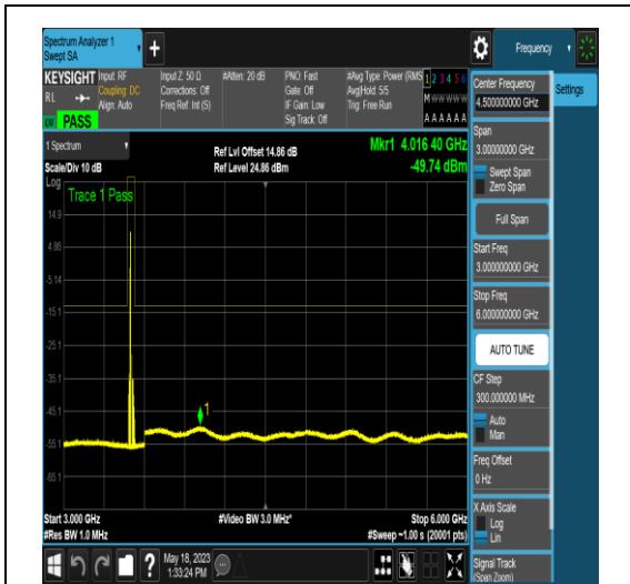
NTNV_N77-3450-3550_PC2_30_15_M_TID6_N/A _3000_6000_#1
