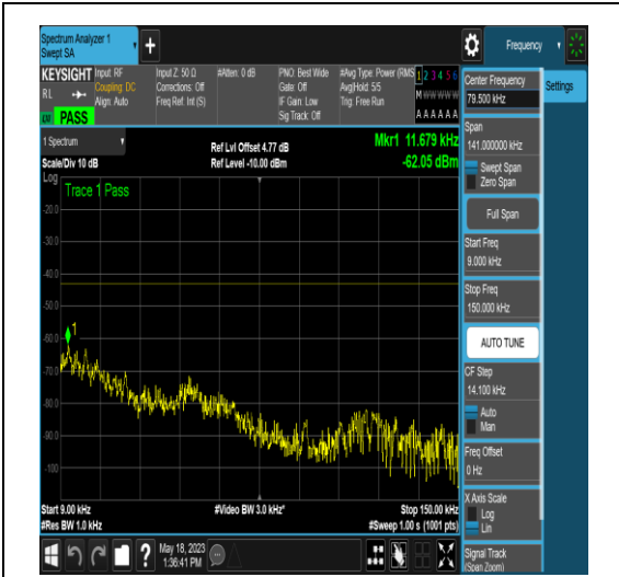
NTNV_N77-3450-3550_PC2_30_15_M_TID5_N/A _0.009_0.15_#1
