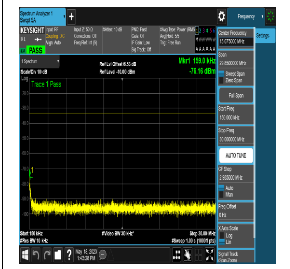
NTNV_N77-3450-3550_PC2_30_15_M_TID17_N/A_0.15_30_#1
