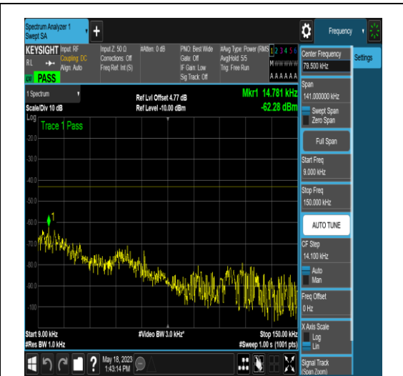
NTNV_N77-3450-3550_PC2_30_15_M_TID17_N/A_0.009_0.15_#1
