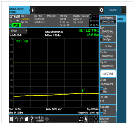
NTNV_N77-3450-3550_PC2_30_15_M_TID18_N/ A_1000_3000_#1
