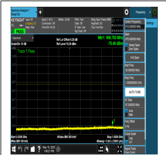
NTNV_N77-3450-3550_PC2_30_15_H_TID6_N/A _30_1000_#1
