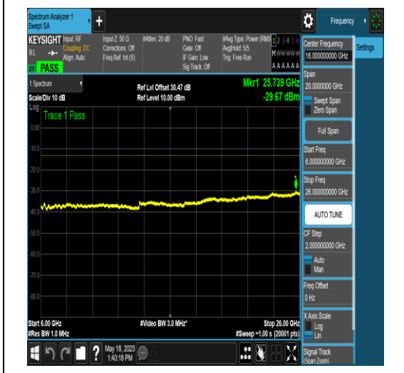
NTNV_N77-3450-3550_PC2_30_15_M_TID18_N/ A_6000_26000_#1
