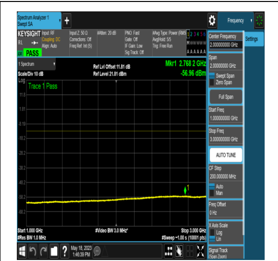
NTNV_N77-3450-3550_PC2_30_15_H_TID6_N/A _1000_3000_#1
