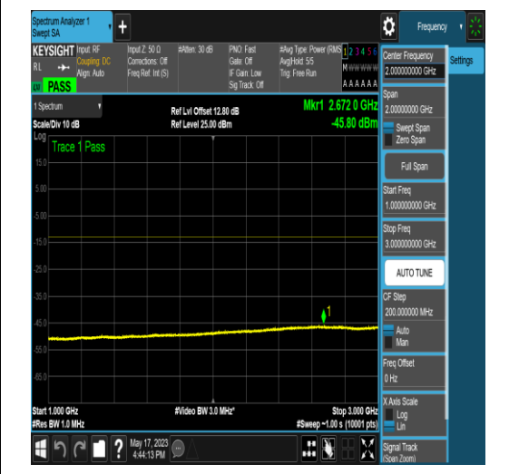
NTNV_N71_PC3_15_10_M_TID17_N/A_1000_30 00_#1
