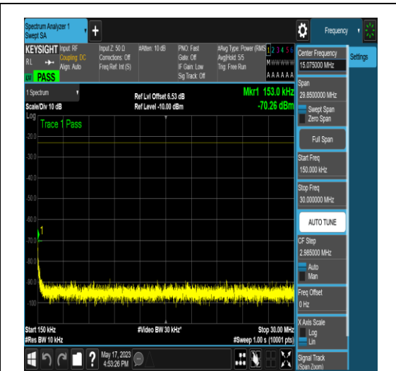
NTNV_N71_PC3_15_10_H_TID16_N/A_0.15_30 #1
