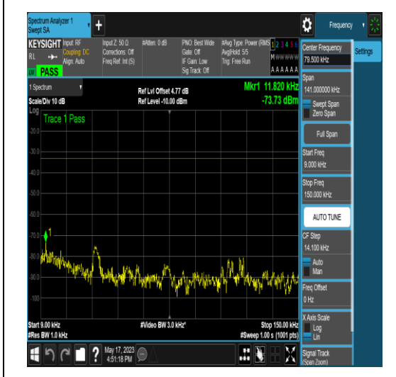
NTNV_N71_PC3_15_10_H_TID5_N/A_3000_120_00_#1
