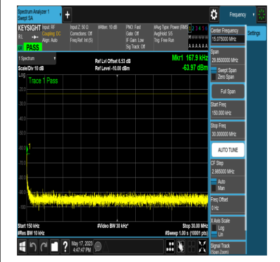
NTNV_N71_PC3_15_10_H_TID4_N/A_0.15_30_# 1
