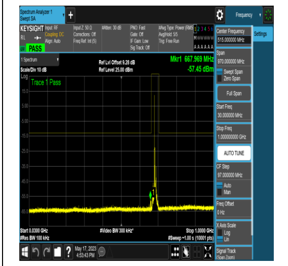
NTNV_N71_PC3_15_10_H_TID16_N/A_30_1000 _#1
