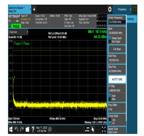
NTNV_N71_PC3_15_10_M_TID5_N/A_0.15_30 #1
