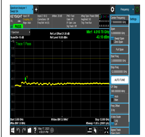
NTNV_N71_PC3_15_10_H_TID5_N/A_3000_120_00_#1
