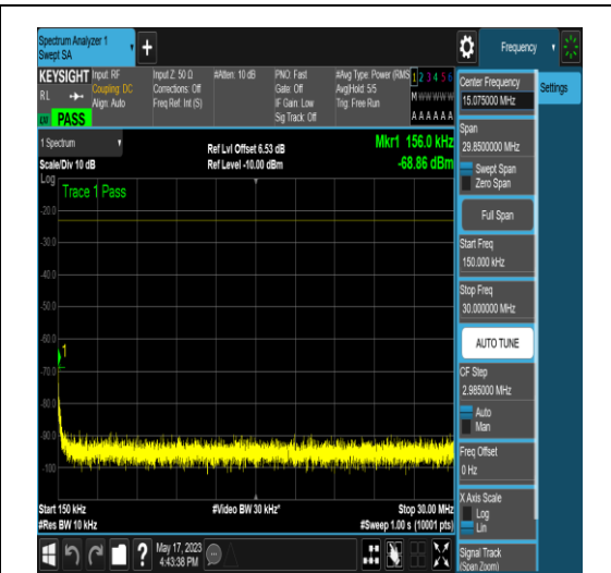
NTNV_N71_PC3_15_10_M_TID17_N/A_0.15_30 _#1
