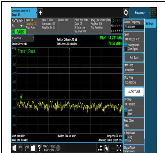
NTNV_N71_PC3_15_10_H_TID16_N/A_0.009_0. 15_#1
