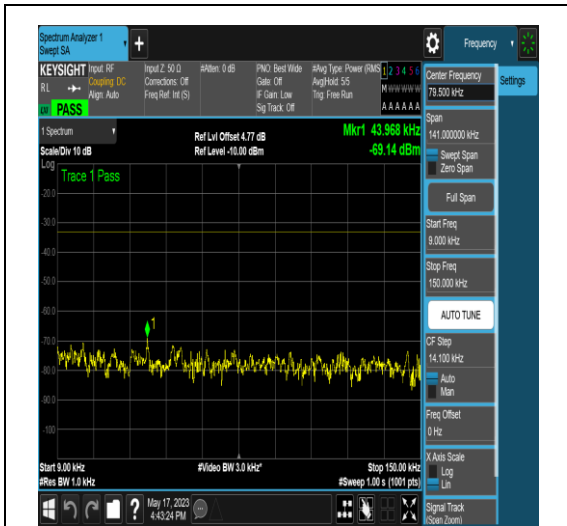
NTNV_N71_PC3_15_10_M_TID17_N/A_0.009_0. 15_#1
