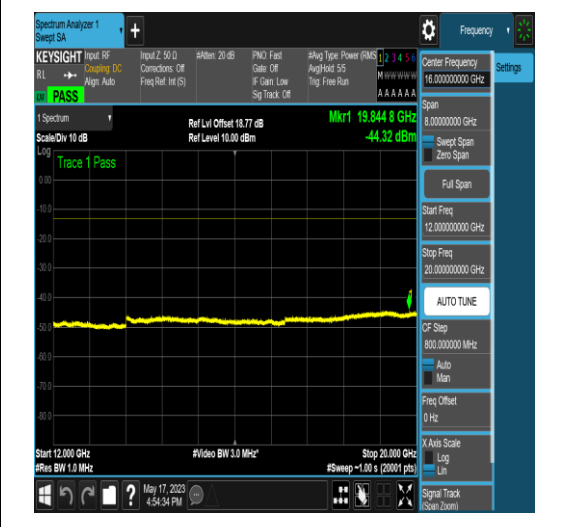
NTNV_N71_PC3_15_10_H_TID16_N/A_1000_30 00_#1
