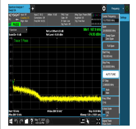
NTNV_N71_PC3_15_10_H_TID5_N/A_12000_20_000_#1
