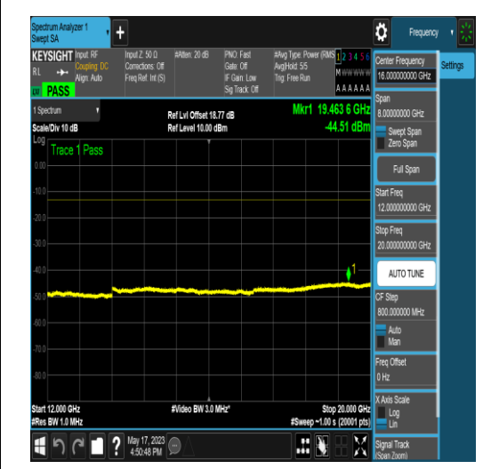
NTNV_N71_PC3_15_10_H_TID5_N/A_12000_20_000_#1
