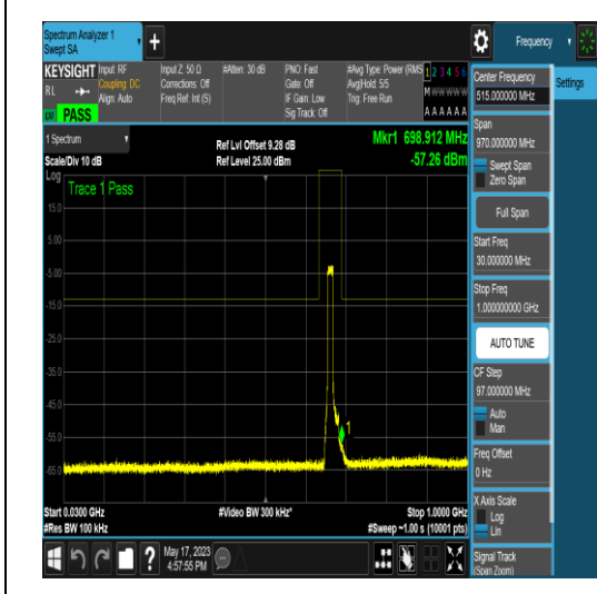
NTNV_N71_PC3_15_15_L_TID6_N/A_0.009_0.1 5_#1
