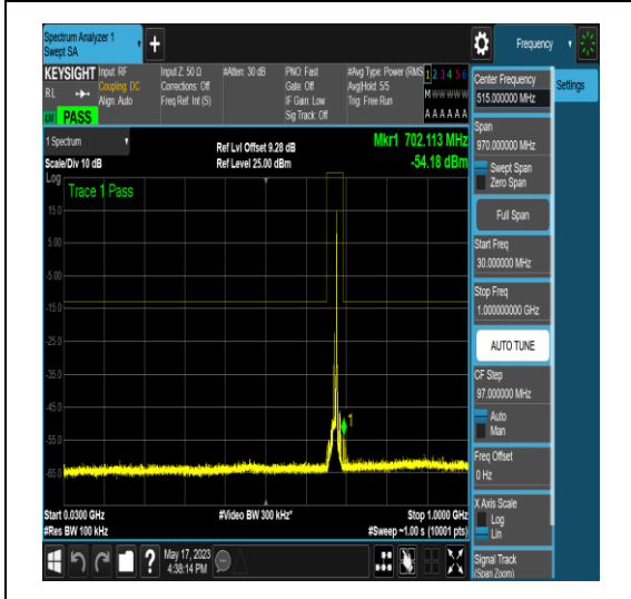
NTNV_N71_PC3_15_10_M_TID5_N/A_0.009_0.1 5_#1
