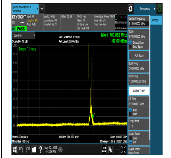
NTNV_N71_PC3_15_10_M_TID17_N/A_30_1000 _#1
