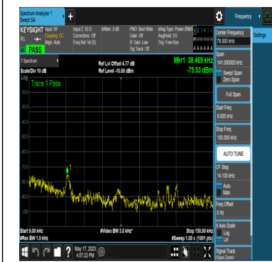
NTNV_N71_PC3_15_15_L_TID6_N/A_0.009_0.1 5_#1
