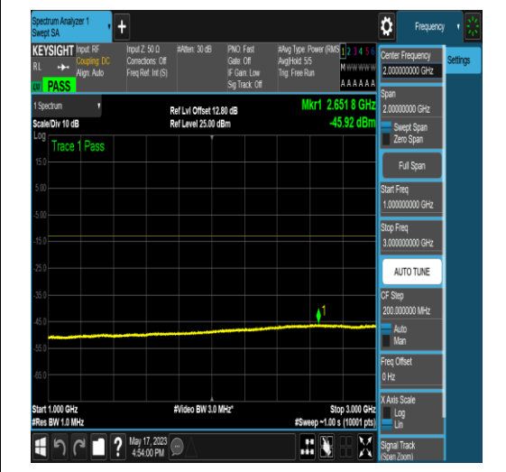
NTNV_N71_PC3_15_10_H_TID16_N/A_1000_30 00_#1
