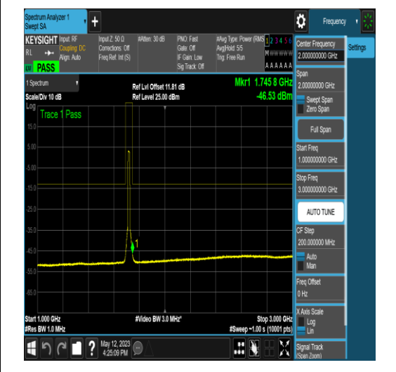
NTNV_N66_PC3_15_15_L_TID18_N/A_0.15_30_#1
