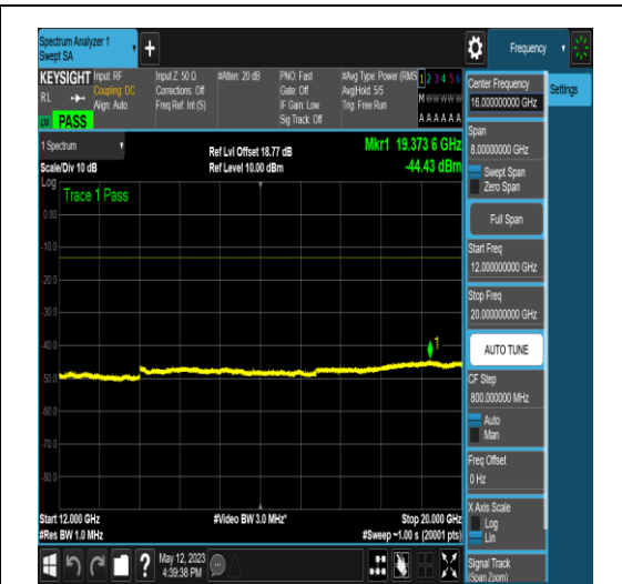
NTNV_N66_PC3_15_15_M_TID16_N/A_12000_2_0000_#1
