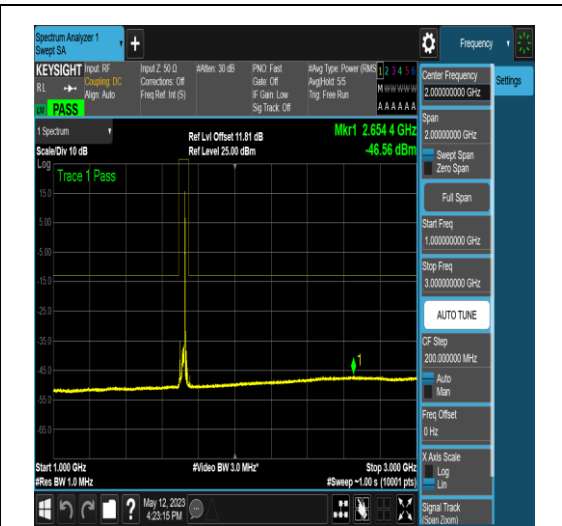
NTNV_N66_PC3_15_15_L_TID5_N/A_1000_300_0_#1
