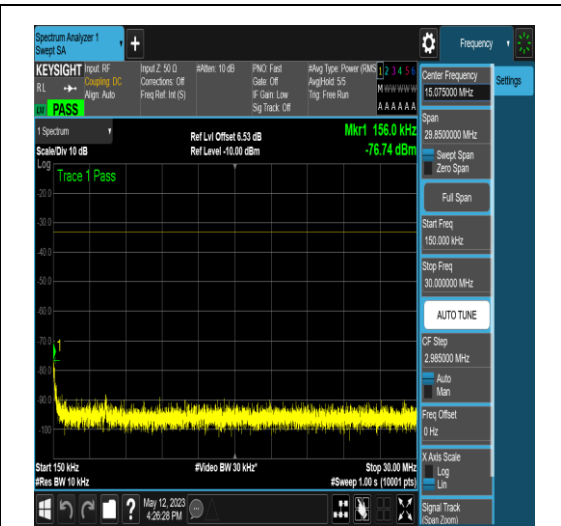
NTNV_N66_PC3_15_15_L_TID16_N/A_0.15_30 #1
