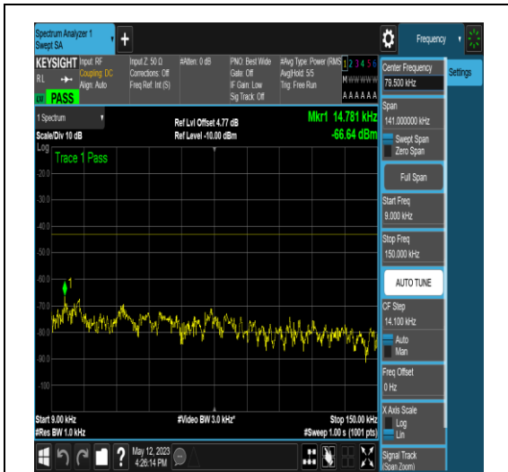
NTNV_N66_PC3_15_15_L_TID16_N/A_0.009_0. 15_#1
