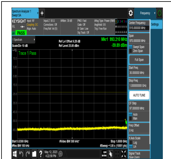
NTNV_N66_PC3_15_15_L_TID5_N/A_30_1000_#1
