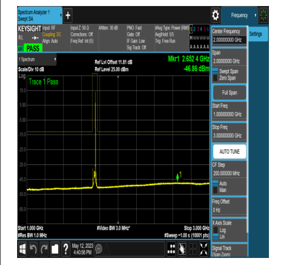
NTNV_N66_PC3_15_15_M_TID17_N/A_0.15_30_#1
