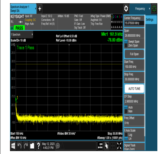
NTNV_N66_PC3_15_15_M_TID17_N/A_0.15_30_#1
