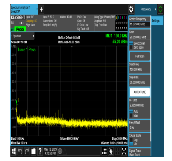
NTNV_N66_PC3_15_15_L_TID5_N/A_12000_20_000_#1
