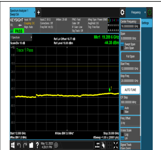
NTNV_N66_PC3_15_15_L_TID17_N/A_12000_20000_#1
