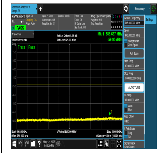
NTNV_N66_PC3_15_15_M_TID17_N/A_0.009_0_15_#1
