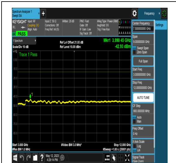
NTNV_N66_PC3_15_15_L_TID17_N/A_3000_12000_#1
