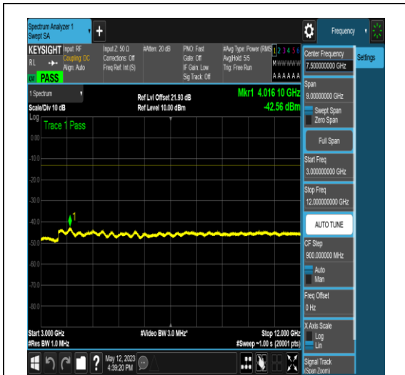
NTNV_N66_PC3_15_15_M_TID16_N/A_3000_12_000_#1
