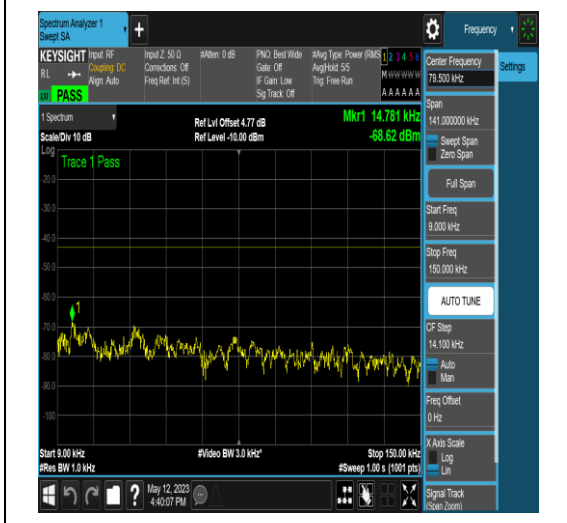
NTNV_N66_PC3_15_15_M_TID17_N/A_0.009_0_15_#1
