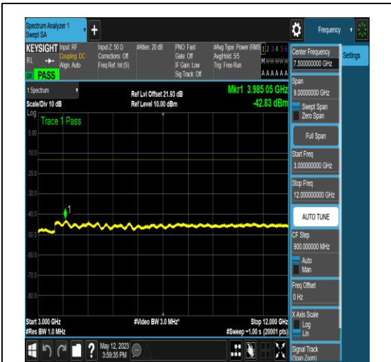
NTNV_N66_PC3_15_10_M_TID5_N/A_3000_120 00_#1
