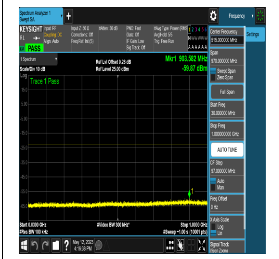
NTNV_N66_PC3_15_10_H_TID17_N/A_30_1000 _#1
