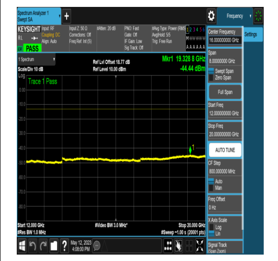
NTNV_N66_PC3_15_10_H_TID6_N/A_12000_20_000_#1
