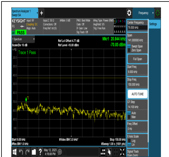
NTNV_N66_PC3_15_10_H_TID17_N/A_0.009_0. 15_#1
