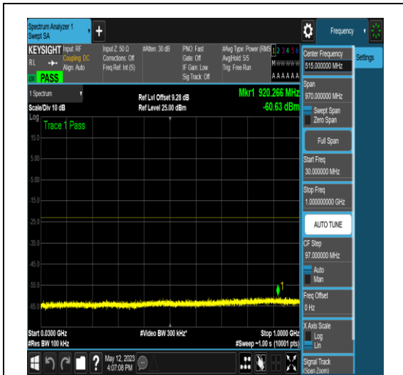
NTNV_N66_PC3_15_10_H_TID6_N/A_30_1000_#1
