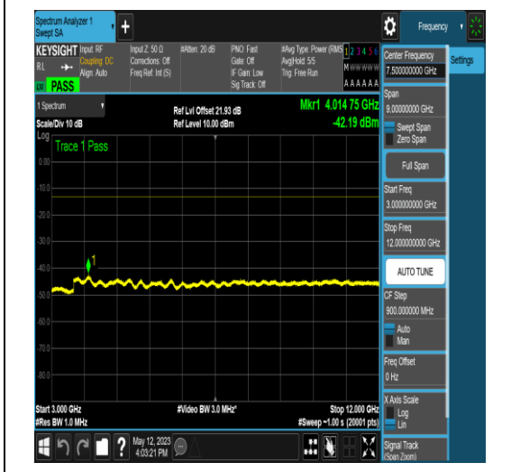
NTNV_N66_PC3_15_10_M_TID16_N/A_3000_12
