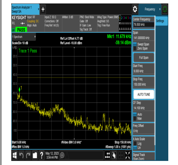
NTNV_N66_PC3_15_10_M_TID6_N/A_0.009_0.1 5_#1
