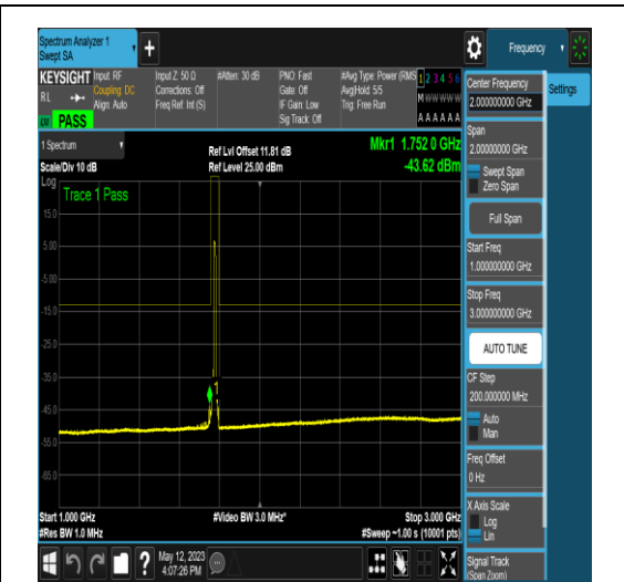
NTNV_N66_PC3_15_10_H_TID6_N/A_1000_300_0_#1
