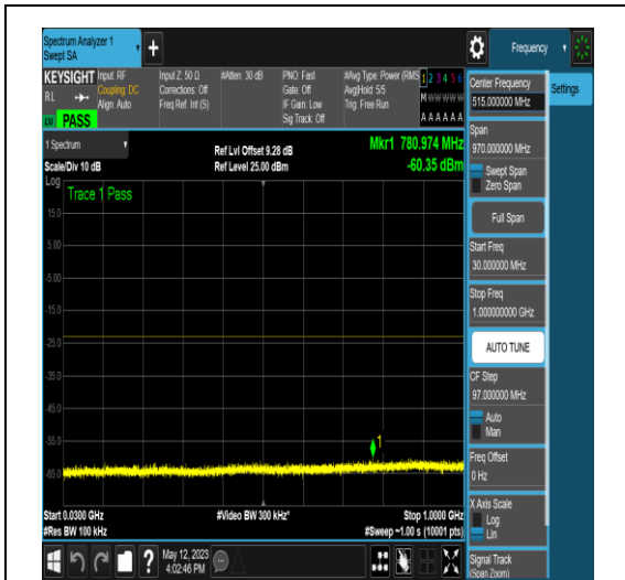
NTNV_N66_PC3_15_10_M_TID16_N/A_30_1000
