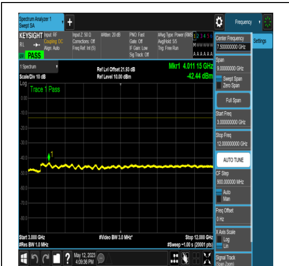
NTNV_N66_PC3_15_10_H_TID4_N/A_3000_120 00_#1
