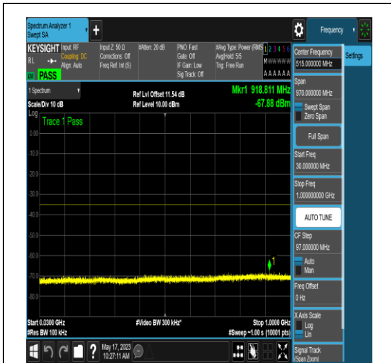
NTNV_N41_PC2_30_100_L_TID5_N/A_30_1000_#1
