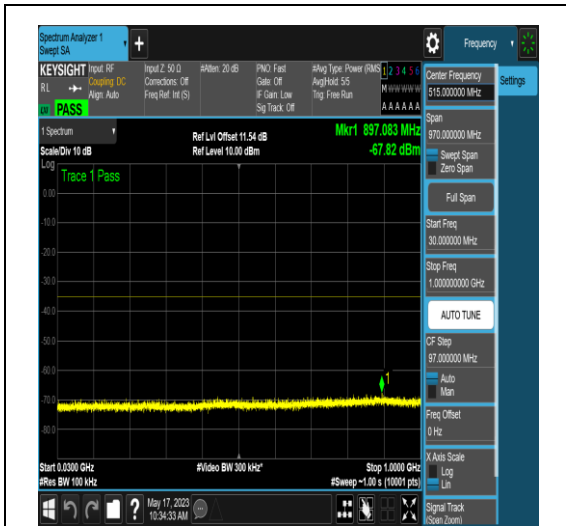
NTNV_N41_PC2_30_100_M_TID4_N/A_30_1000_#1
