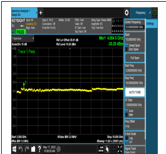
NTNV_N41_PC2_30_90_M_TID4_N/A_3000_180 00_#1
