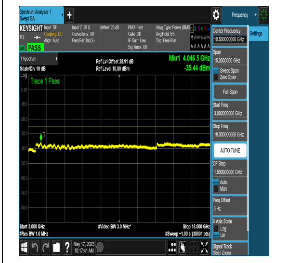
NTNV_N41_PC2_30_90_H_TID4_N/A_30_1000_#1
