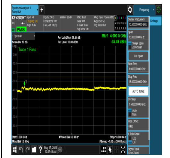
NTNV_N41_PC2_30_100_L_TID5_N/A_3000_18000_#1
