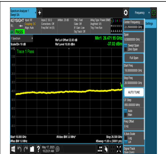
NTNV_N41_PC2_30_90_H_TID17_N/A_18000_26500_#1
