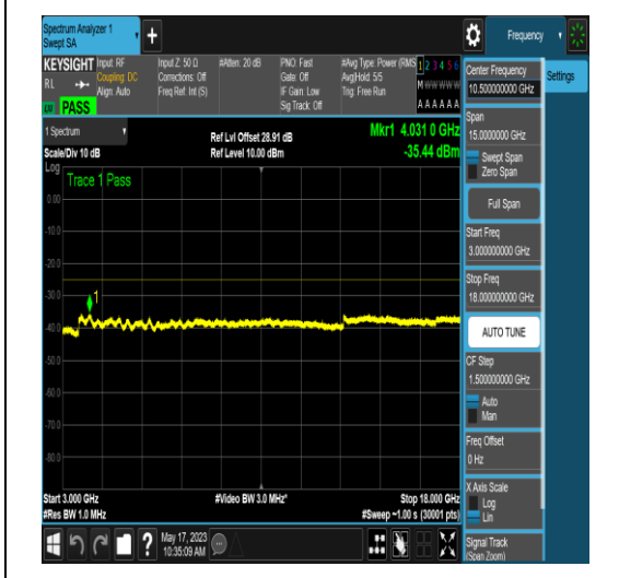
NTNV_N41_PC2_30_100_M_TID4_N/A_3000_18000_#1
