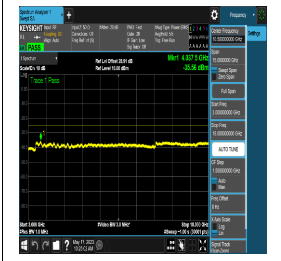
NTNV_N41_PC2_30_90_H_TID17_N/A_3000_18000_2_000_#1
