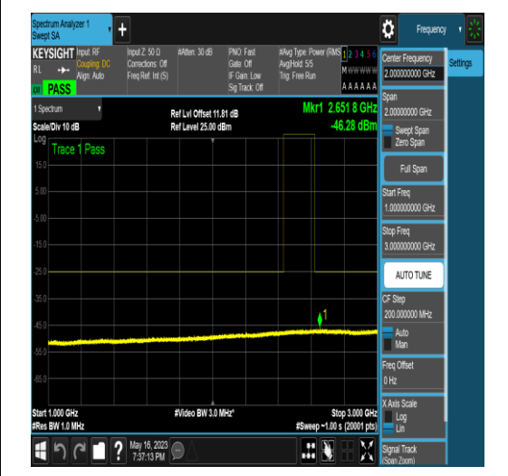
NTNV_N41_PC2_30_60_L_TID16_N/A_1000_30_00_#1
