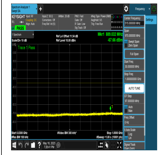
NTNV_N41_PC2_30_50_H_TID5_N/A_3000_180_00_#1
