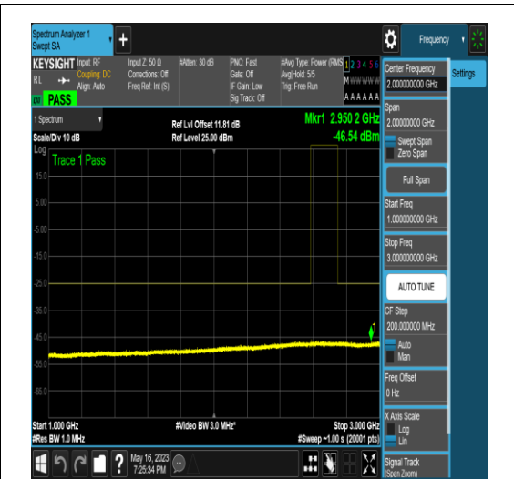
NTNV_N41_PC2_30_50_H_TID5_N/A_1000_300_0_#1
