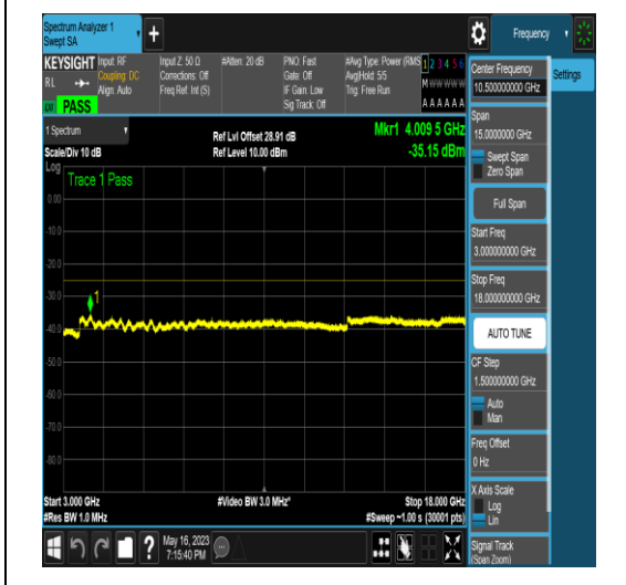
NTNV_N41_PC2_30_50_M_TID4_N/A_30_1000 #1
