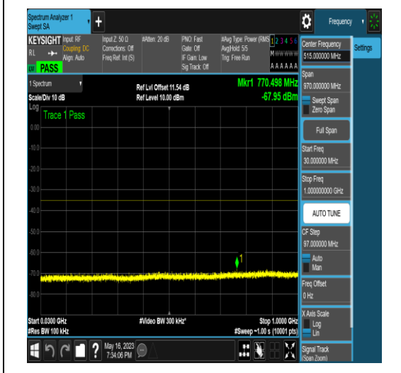
NTNV_N41_PC2_30_60_L_TID4_N/A_3000_180
