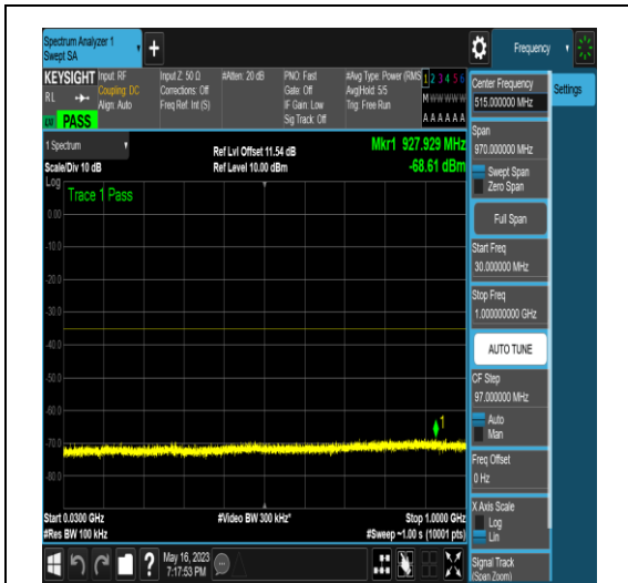
NTNV_N41_PC2_30_50_M_TID18_N/A_30_1000_#1
