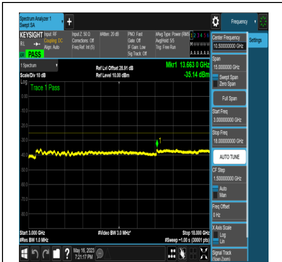
NTNV_N41_PC2_30_50_M_TID17_N/A_3000_18 000_#1
