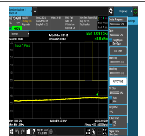
NTNV_N41_PC2_30_50_M_TID18_N/A_1000_30_00_#1
