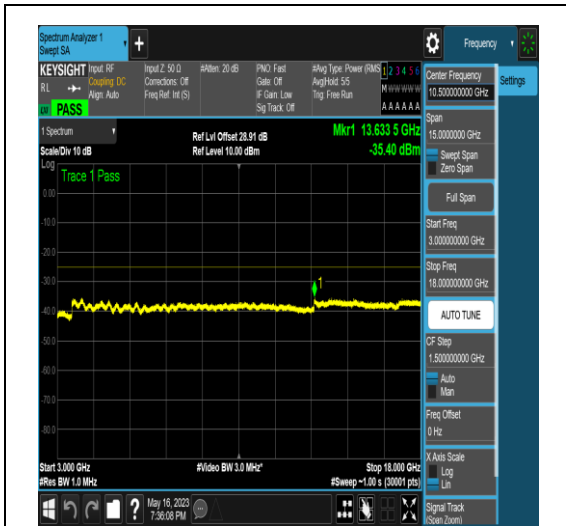
NTNV_N41_PC2_30_60_L_TID18_N/A_3000_18_000_#1
