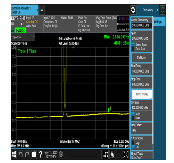
NTNV_N25_PC3_15_15_L_TID18_N/A_1000_30 00_#1
