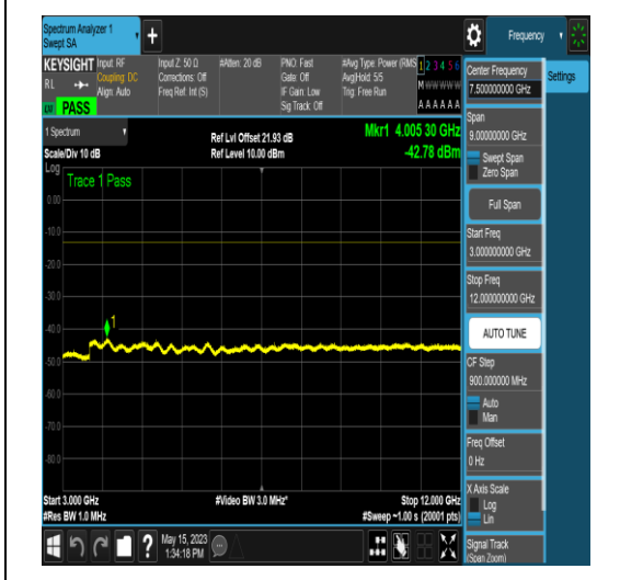
NTNV_N25_PC3_15_15_M_TID6_N/A_3000_120 00_#1
