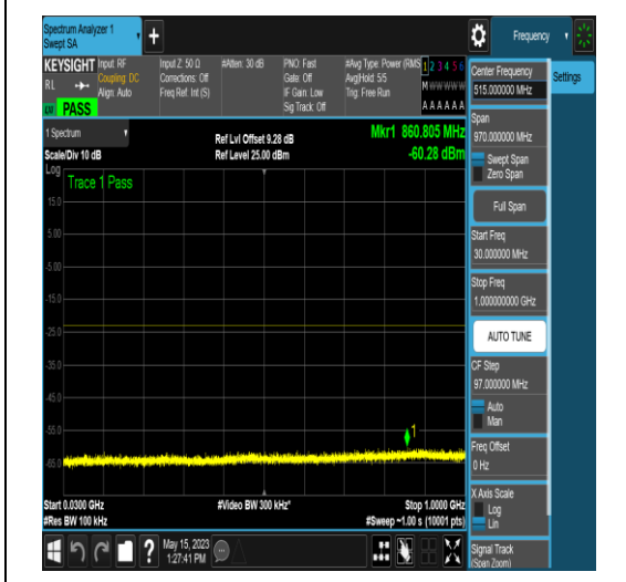
NTNV_N25_PC3_15_15_L_TID18_N/A_30_1000 _#1
