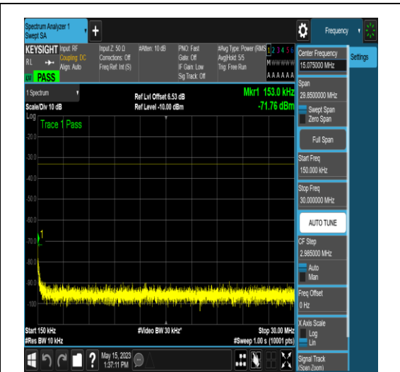
NTNV_N25_PC3_15_15_M_TID5_N/A_0.15_30
