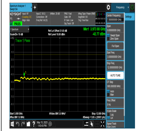
NTNV_N25_PC3_15_15_M_TID17_N/A_3000_12 000_#1
