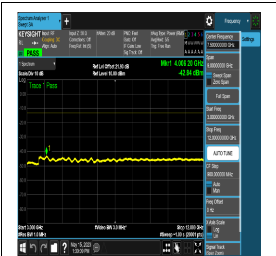
NTNV_N25_PC3_15_15_L_TID16_N/A_3000_12 000_#1
