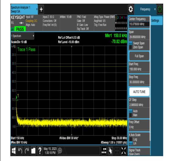
NTNV_N25_PC3_15_15_M_TID6_N/A_12000_20 000_#1
