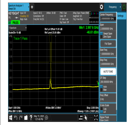
NTNV_N25_PC3_15_15_M_TID5_N/A_1000_300
