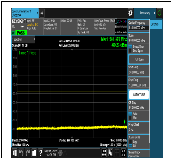
NTNV_N25_PC3_15_15_M_TID17_N/A_30_1000 _#1
