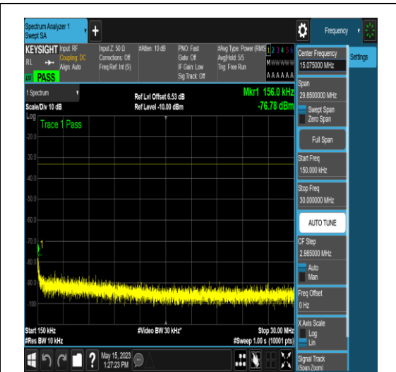
NTNV_N25_PC3_15_15_L_TID18_N/A_0.15_30 #1
