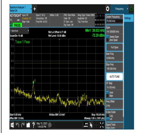
NTNV_N25_PC3_15_15_M_TID17_N/A_3000_12 000_#1
