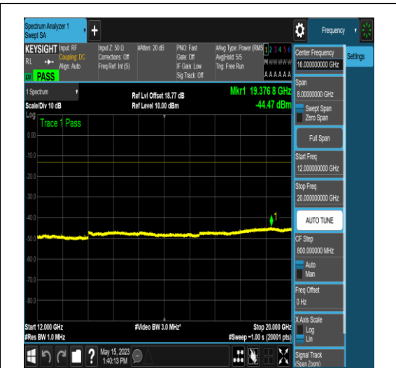
NTNV_N25_PC3_15_15_M_TID18_N/A_12000_2 0000_#1
