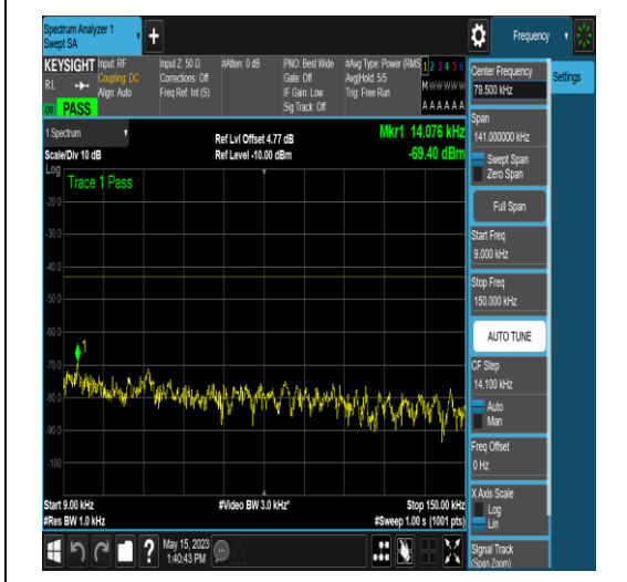
NTNV_N25_PC3_15_15_M_TID16_N/A_0.009_0. 15_#1
