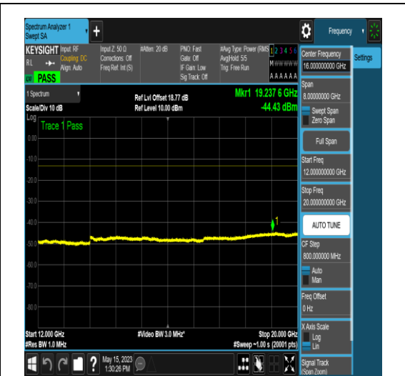
NTNV_N25_PC3_15_15_L_TID16_N/A_12000_2 0000_#1
