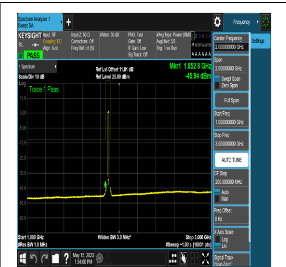
NTNV_N25_PC3_15_15_M_TID6_N/A_1000_300 0_#1
