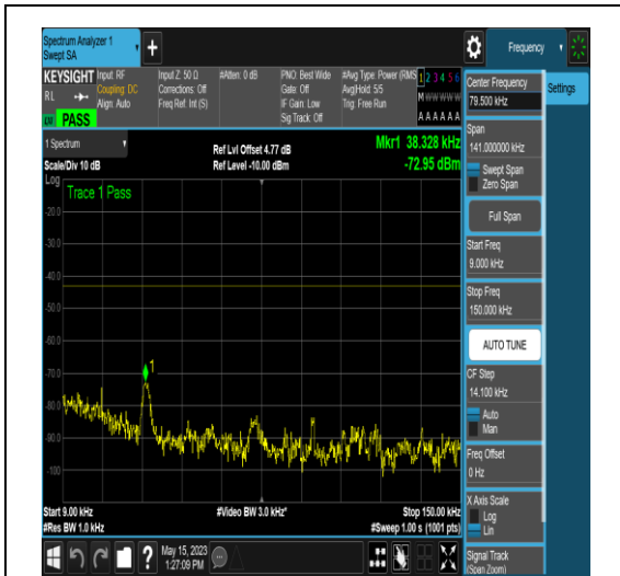
NTNV_N25_PC3_15_15_L_TID18_N/A_0.009_0. 15_#1
