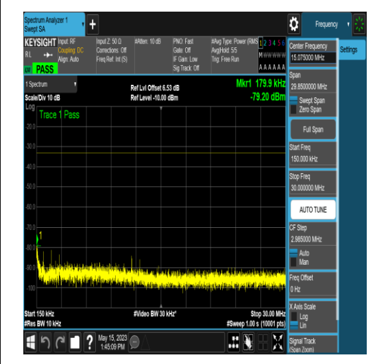
NTNV_N25_PC3_15_15_M_TID17_N/A_12000_2 0000_#1
