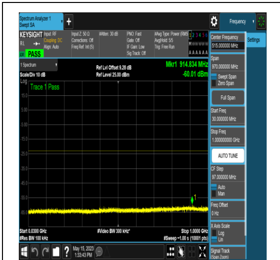
NTNV_N25_PC3_15_15_M_TID6_N/A_30_1000 #1
