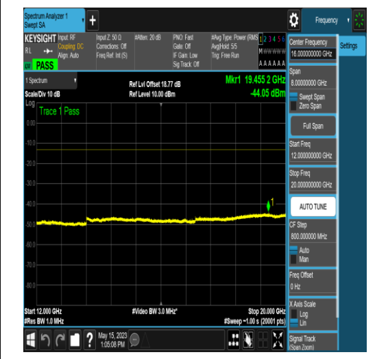
NTNV_N25_PC3_15_10_M_TID18_N/A_12000_2 0000_#1
