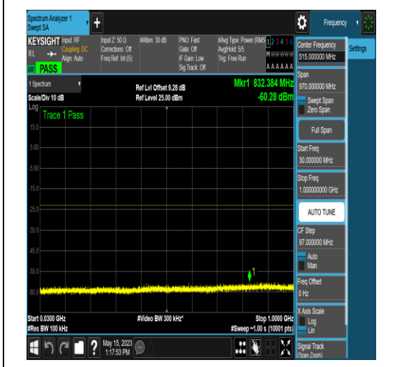
NTNV_N25_PC3_15_10_H_TID16_N/A_30_1000 _#1
