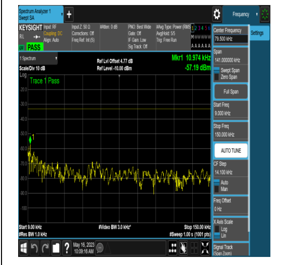
NTNV_N5_PC3_15_15_M_TID4_N/A_3000_1200
