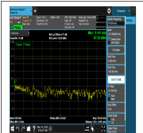
NTNV_N5_PC3_15_15_H_TID5_N/A_0.009_0.15 _#1
