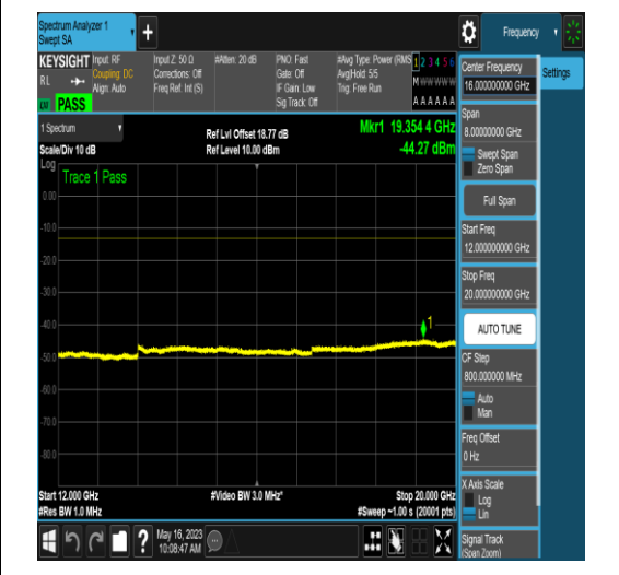
NTNV_N5_PC3_15_15_M_TID4_N/A_12000_200
