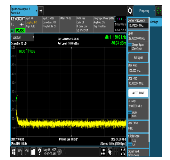
NTNV_N5_PC3_15_15_H_TID6_N/A_12000_200
