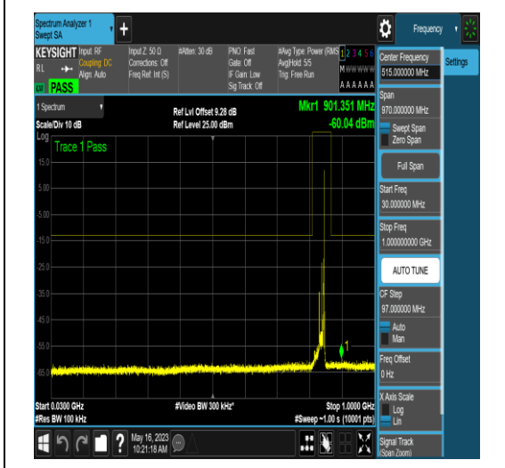
NTNV_N5_PC3_15_15_H_TID5_N/A_30_1000_# 1
