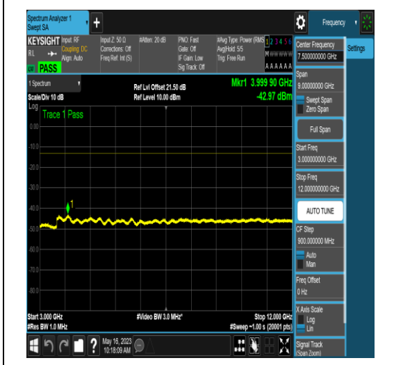
NTNV_N5_PC3_15_15_H_TID6_N/A_3000_1200
