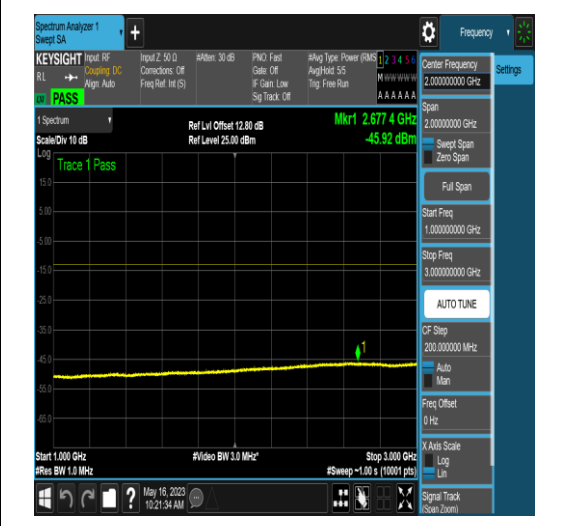
NTNV_N5_PC3_15_15_H_TID5_N/A_1000_3000 _#1
