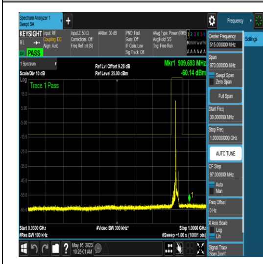
NTNV_N5_PC3_15_15_H_TID16_N/A_0.009_0.1
