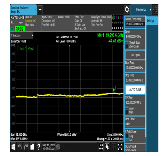
NTNV_N5_PC3_15_15_H_TID17_N/A_12000_20_000_#1
