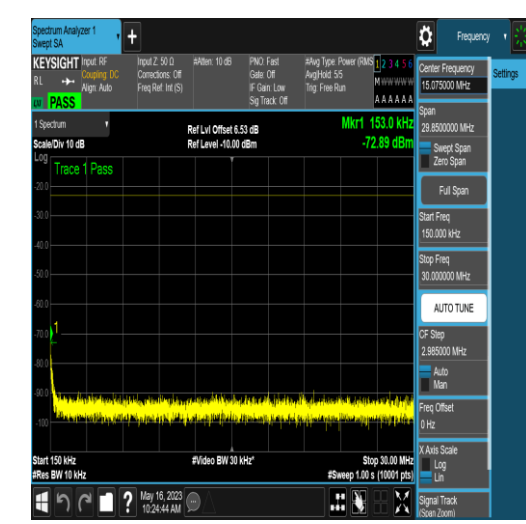
NTNV_N5_PC3_15_15_H_TID16_N/A_0.15_30_#
