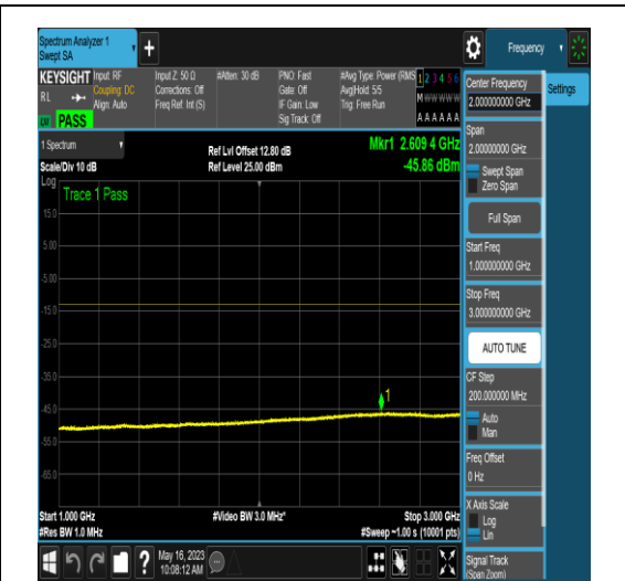
NTNV_N5_PC3_15_15_M_TID4_N/A_1000_3000
