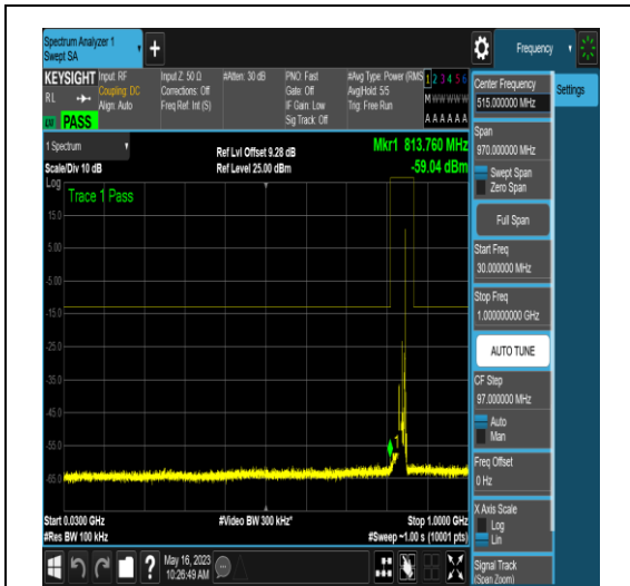
NTNV_N5_PC3_15_15_H_TID17_N/A_30_1000_#1
