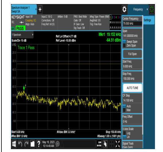
NTNV_N5_PC3_15_15_M_TID17_N/A_0.009_0.1 5_#1
