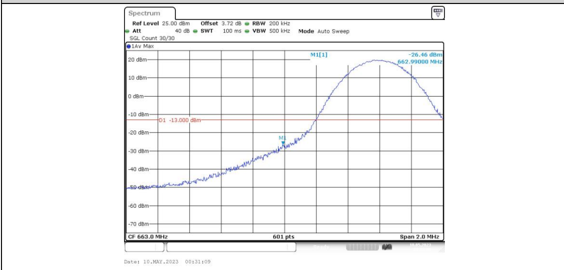
Band71-10MHz-16QAM-133172-1RB#49
