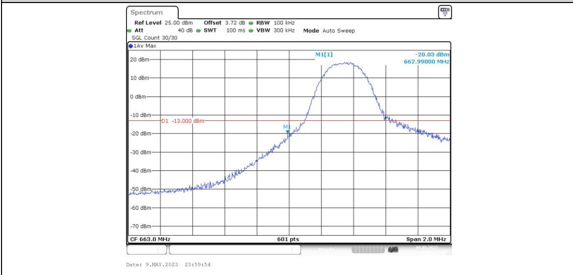
Band71-5MHz-16QAM-133147-1RB#24
