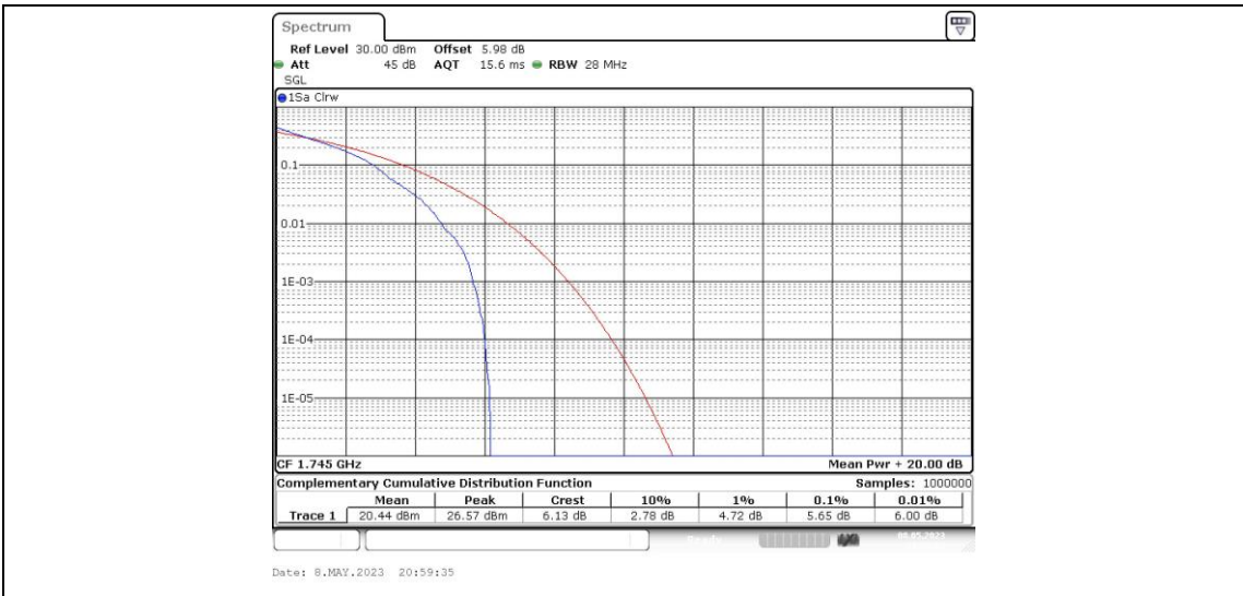
Band66-5MHz-QPSK-132322-25RB#0
