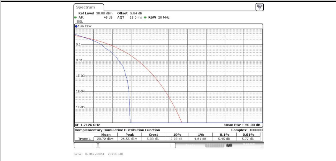
Band66-5MHz-QPSK-131997-25RB#0
