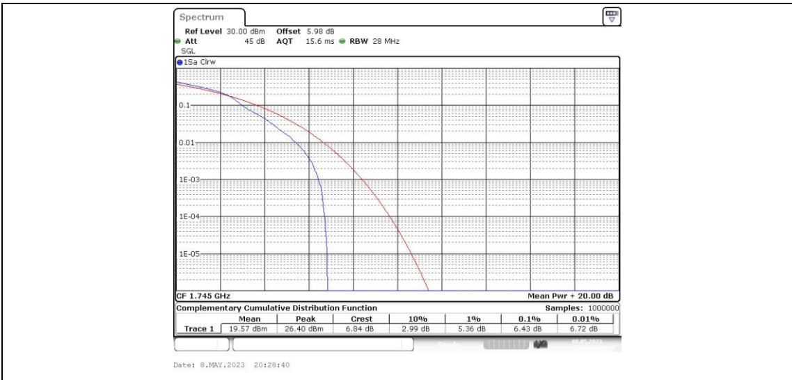
Band66-3MHz-16QAM-132322-15RB#0
