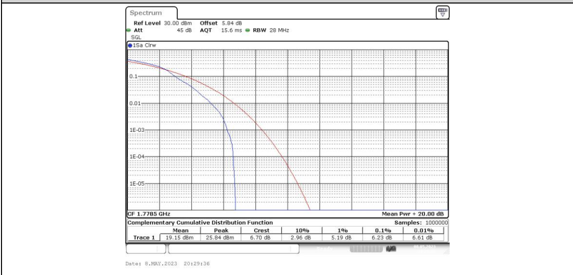
Band66-3MHz-16QAM-132657-15RB#0
