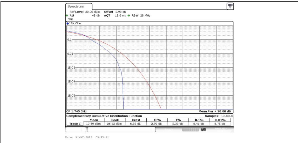
Band66-10MHz-16QAM-132322-50RB#0
