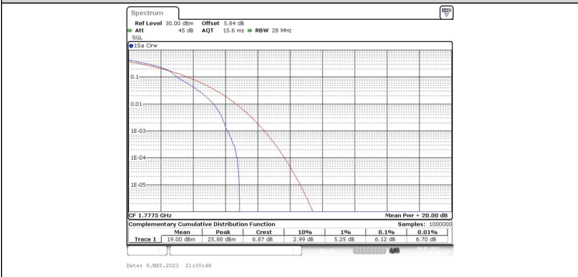
Band66-5MHz-16QAM-132647-25RB#0
