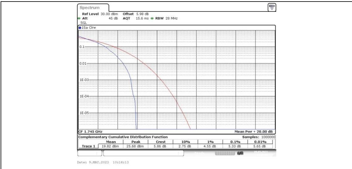
Band66-15MHz-QPSK-132322-75RB#0
