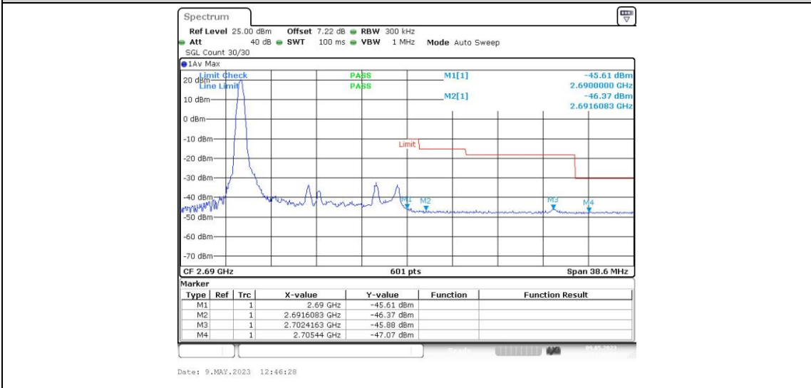
Band41-15MHz-QPSK-41515-1RB#74
