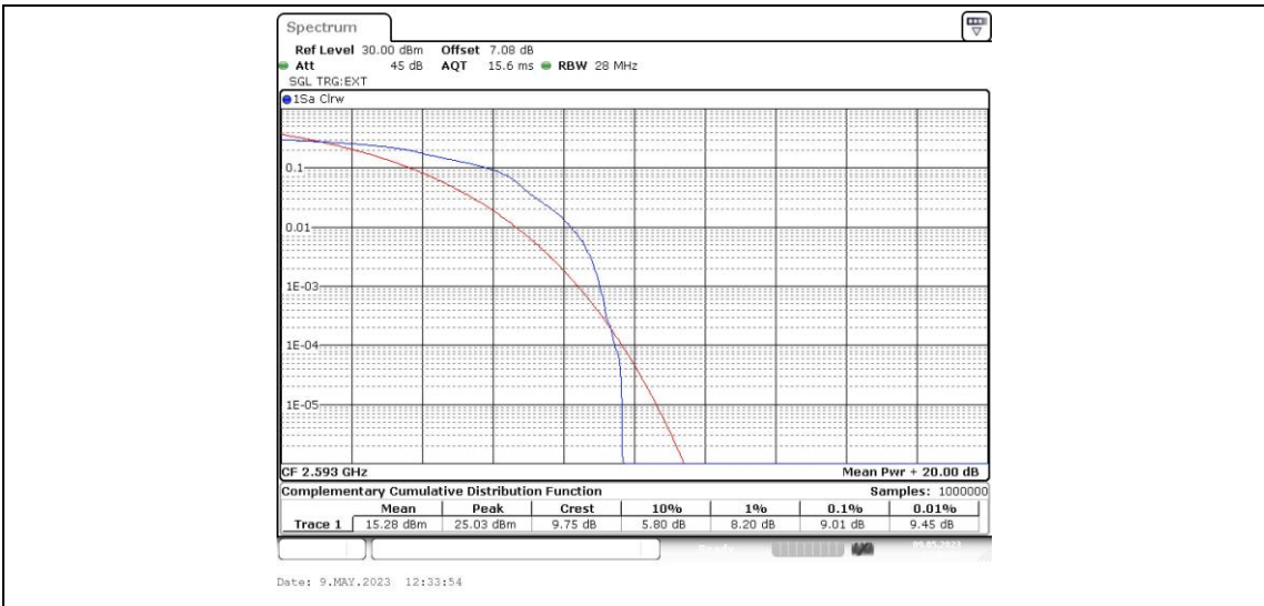
Band41-10MHz-16QAM-40620-50RB#0
