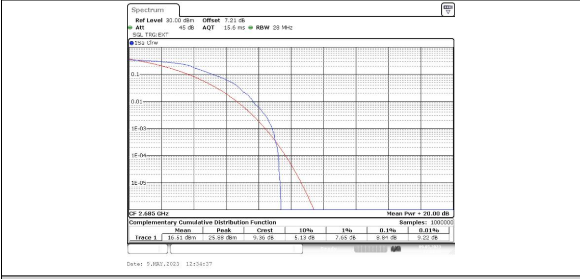
Band41-10MHz-QPSK-41540-50RB#0
