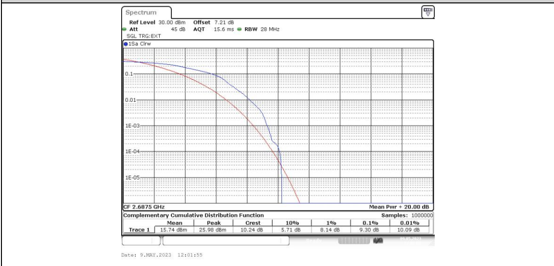
Band41-5MHz-16QAM-41565-25RB#0
