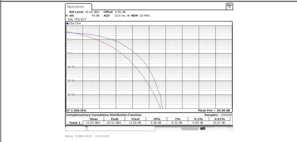
Band41-20MHz-16QAM-40620-1RB#0
