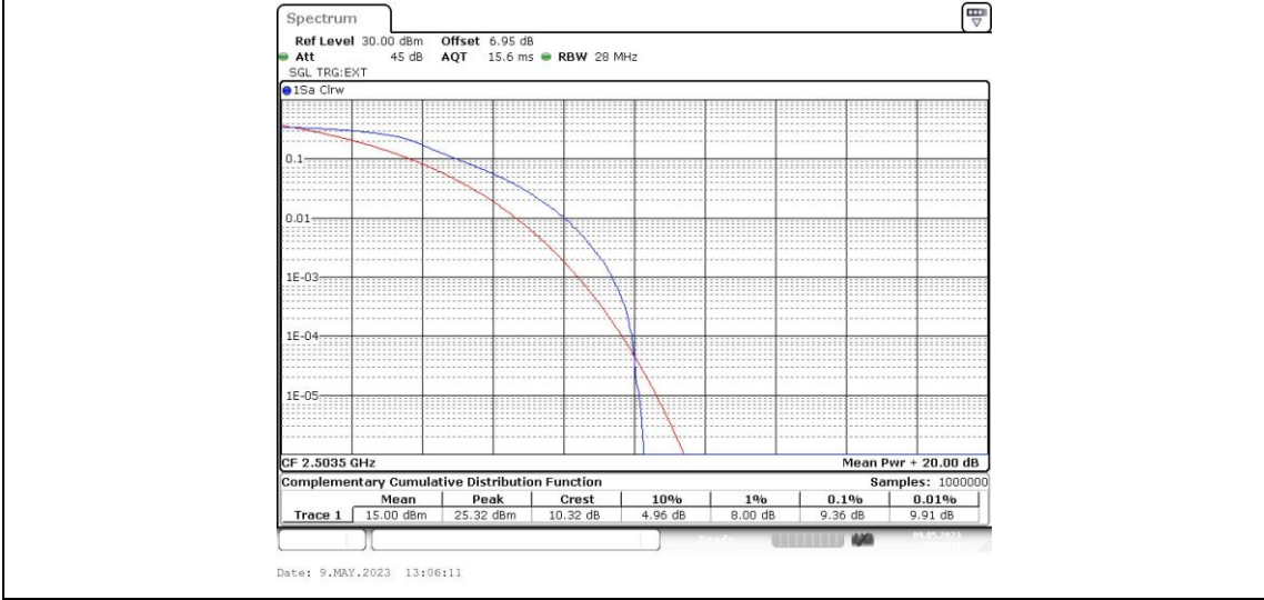
Band41-15MHz-QPSK-40620-1RB#0
