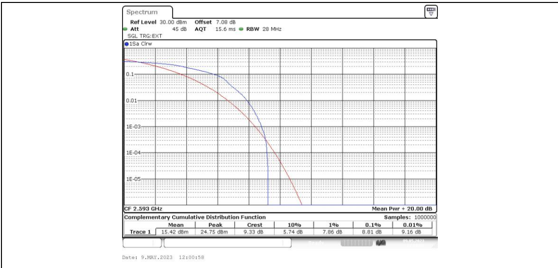
Band41-5MHz-16QAM-40620-25RB#0
