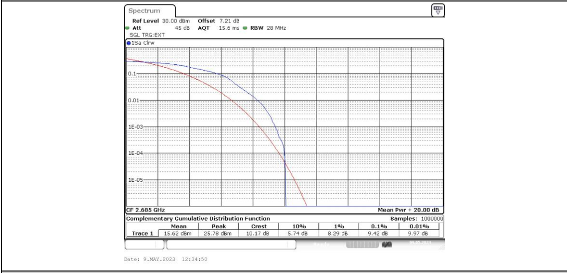
Band41-10MHz-16QAM-41540-50RB#0
