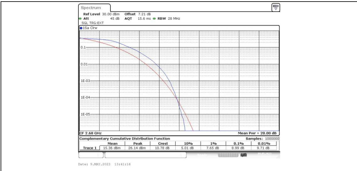
Band41-20MHz-16QAM-39750-1RB#0
