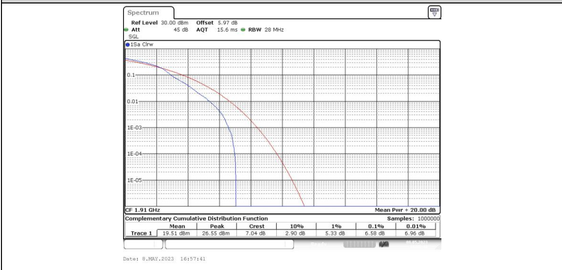
Band25-10MHz-16QAM-26640-50RB#0
