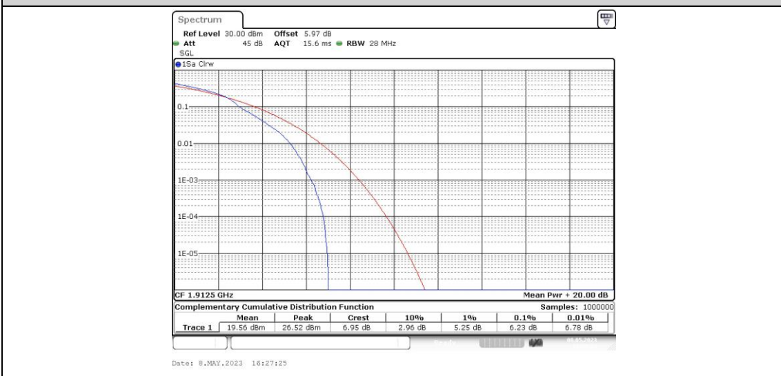
Band25-5MHz-16QAM-26665-25RB#0
