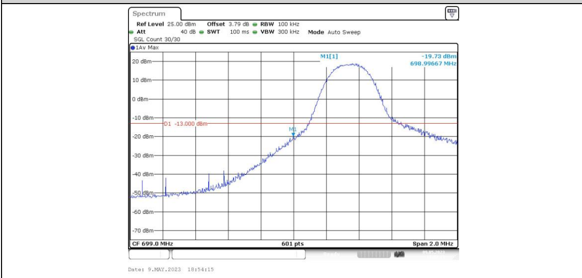
Band12-5MHz-16QAM-23035-1RB#24
