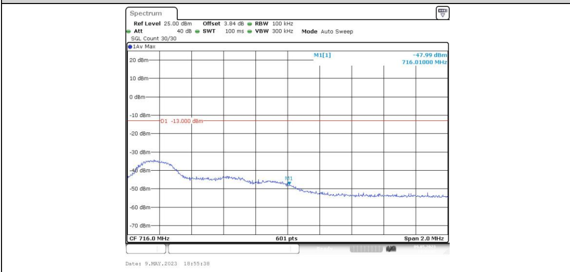
Band12-5MHz-16QAM-23155-1RB#24
