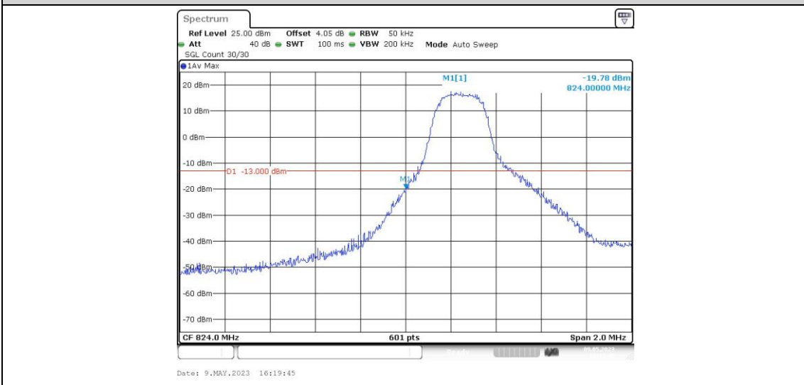
Band5-3MHz-16QAM-20415-1RB#14
