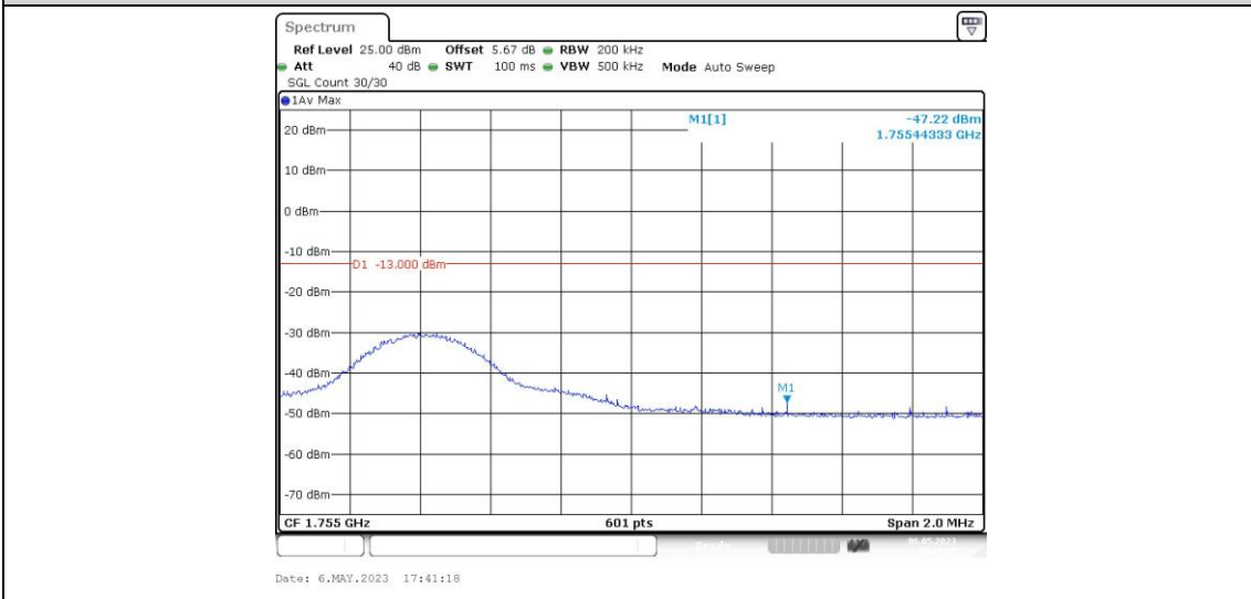
Band4-10MHz-16QAM-20350-1RB#49
