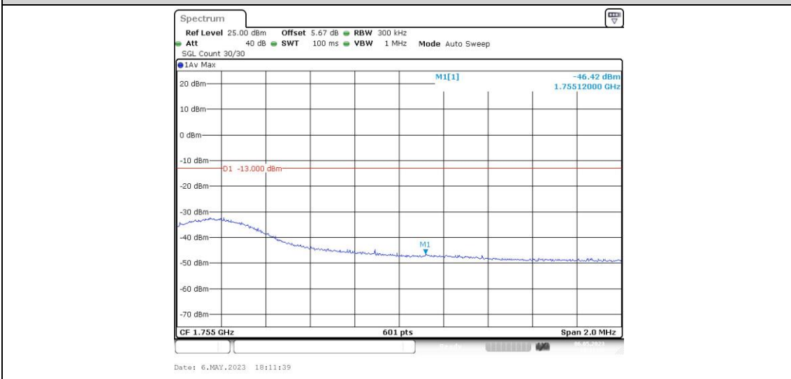
Band4-15MHz-QPSK-20325-1RB#74
