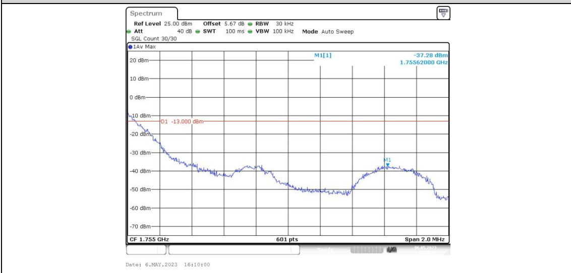
Band4-1.4MHz-QPSK-20393-1RB#5
