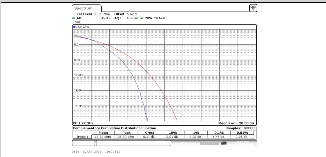
Band4-20MHz-16QAM-20175-1RB#0
