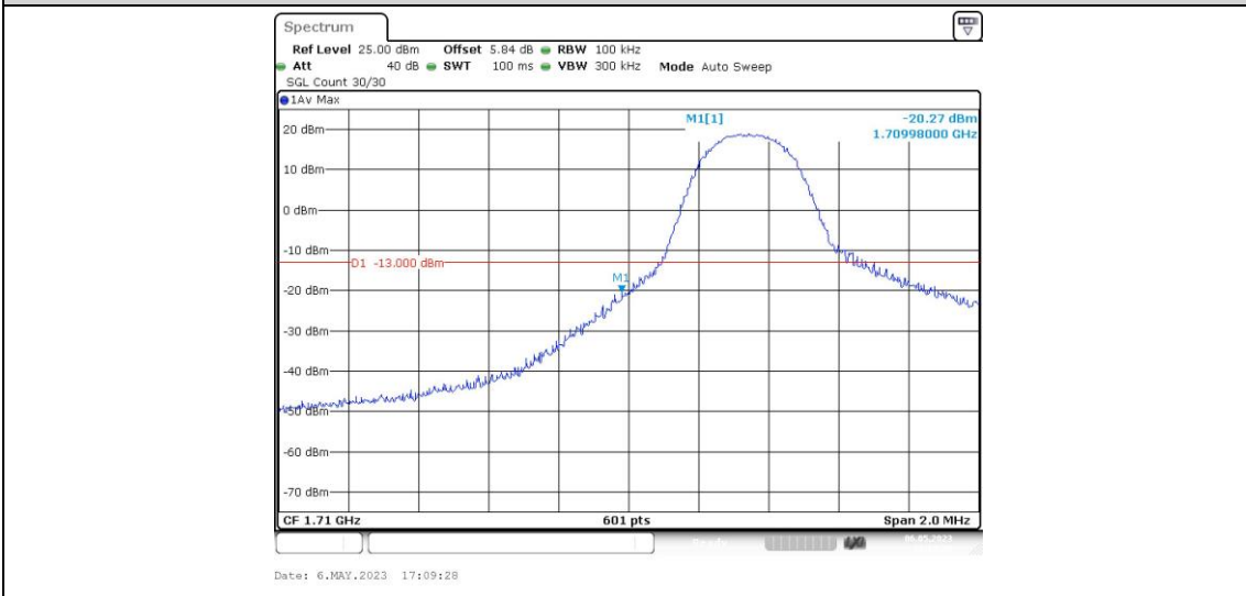
Band4-5MHz-QPSK-19975-1RB#24
