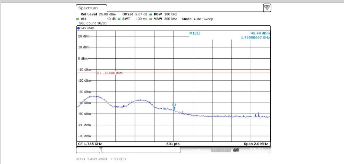
Band4-5MHz-QPSK-20375-1RB#24
