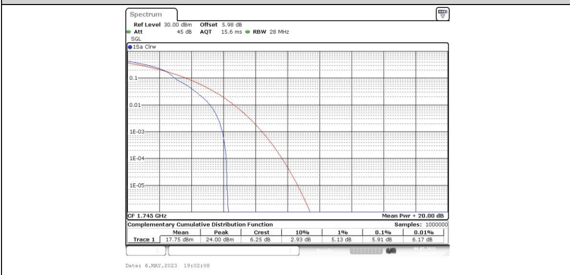
Band4-20MHz-16QAM-20300-100RB#0
