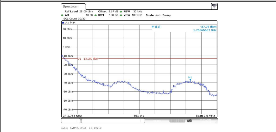
Band4-1.4MHz-16QAM-20393-1RB#5
