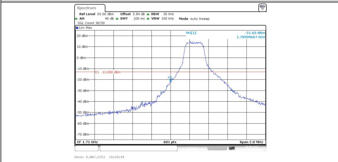
Band4-1.4MHz-16QAM-19957-1RB#5
