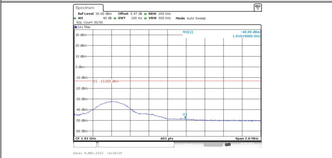
Band2-10MHz-QPSK-19150-1RB#49
