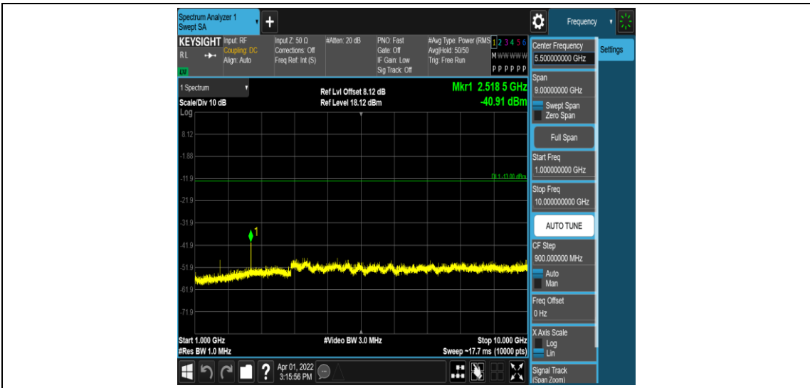
Band26-10MHz-16QAM-26990-1RB#0-Range4: 1000~10000MHz
