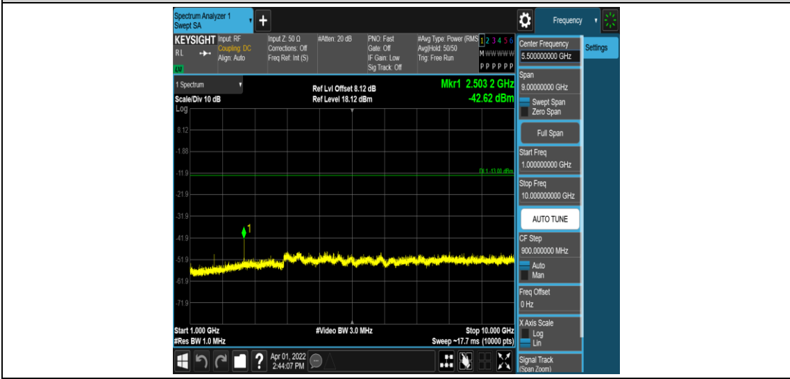
Band26-5MHz-16QAM-26915-1RB#0-Range4:1000~10000MHz
