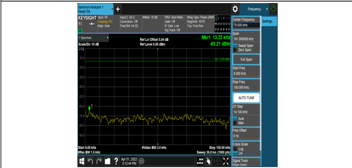
Band26-10MHz-QPSK-26915-1RB#0-Range1:0.009~0.15MHz
