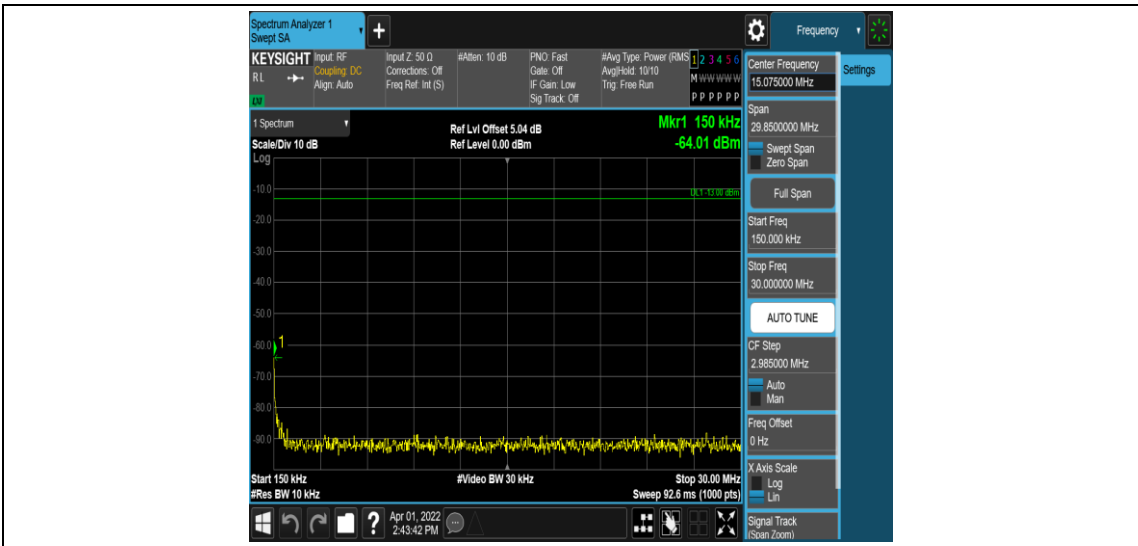
Band26-5MHz-16QAM-26915-1RB#0-Range2:0.15~30MHz
