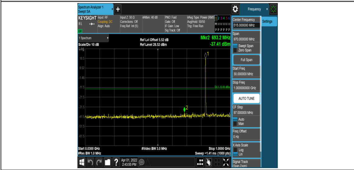
Band26-5MHz-16QAM-26915-1RB#0-Range3:30~1000MHz
