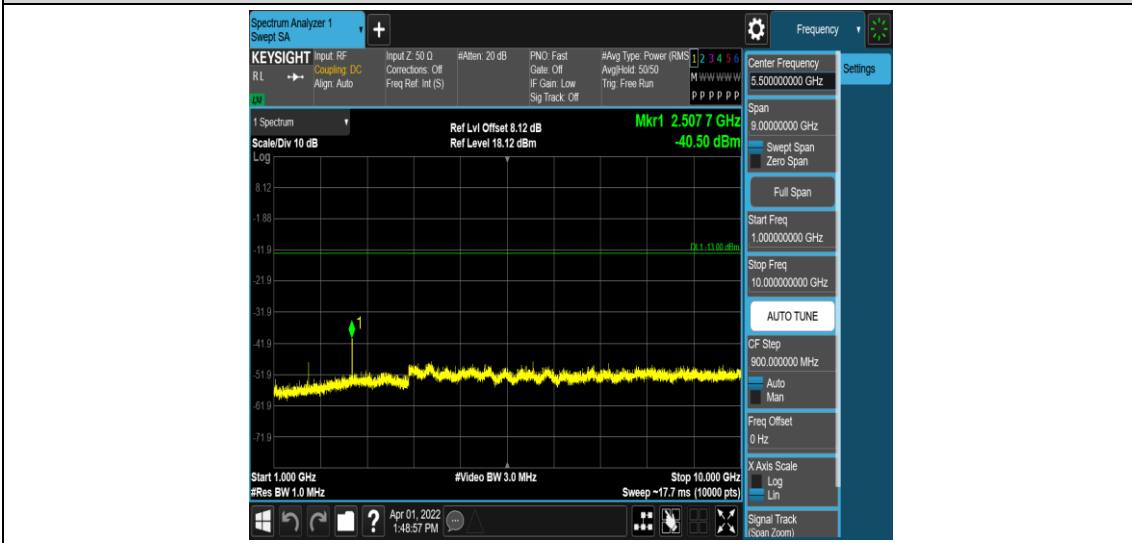
Band26-1.4MHz-QPSK-26915-1RB#0-Range4:1000~10000MHz
