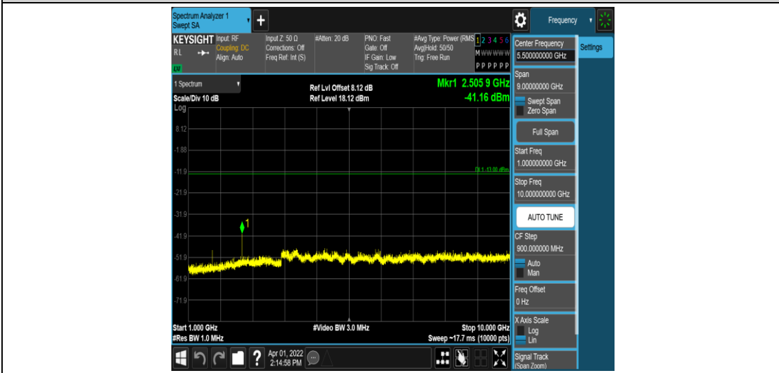
Band26-3MHz-16QAM-26915-1RB#0-Range4:1000~10000MHz
