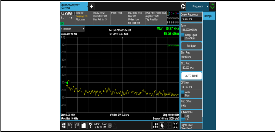
Band26-3MHz-16QAM-26805-1RB#0-Range1:0.009~0.15MHz
