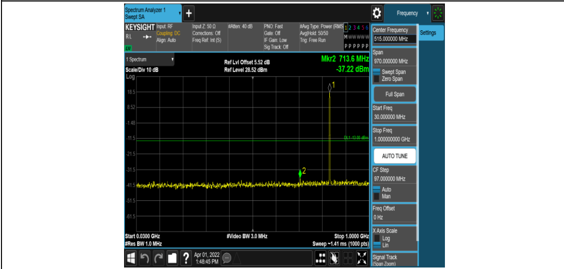
Band26-1.4MHz-QPSK-26915-1RB#0-Range3:30~1000MHz
