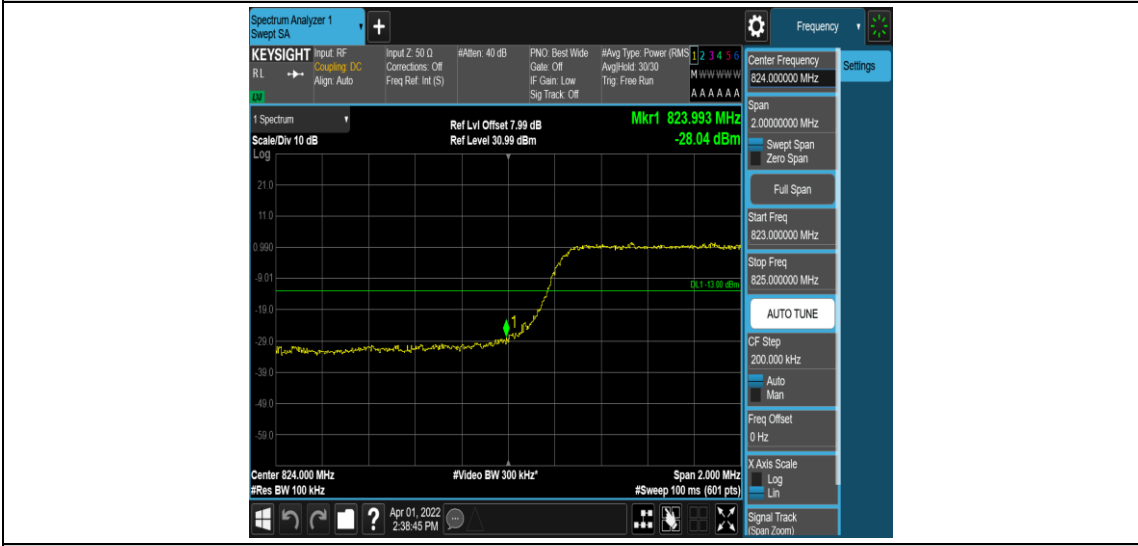
Band26-5MHz-16QAM-26815-25RB#0
