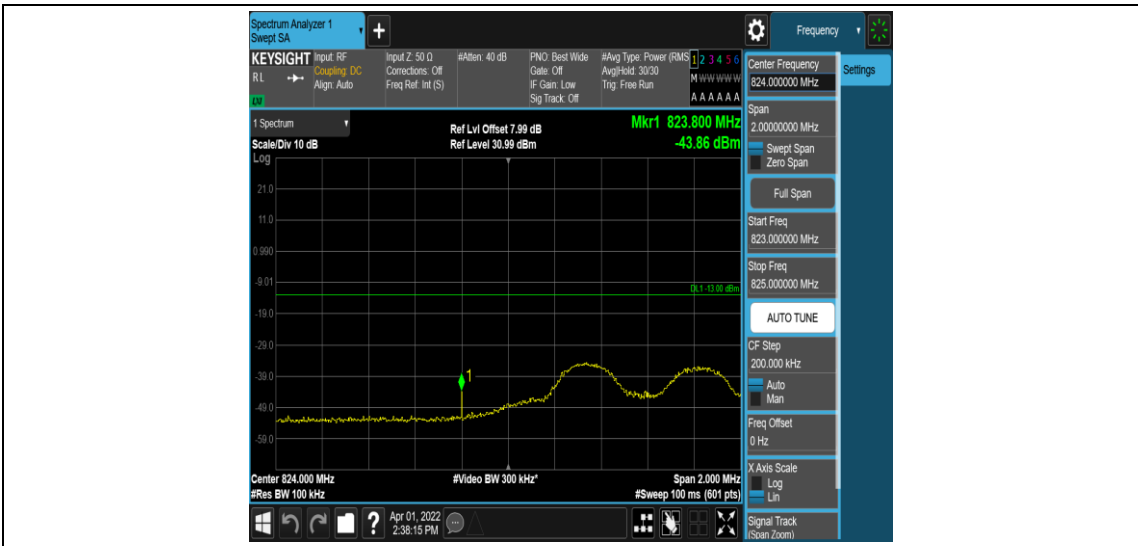
Band26-5MHz-16QAM-26815-1RB#24
