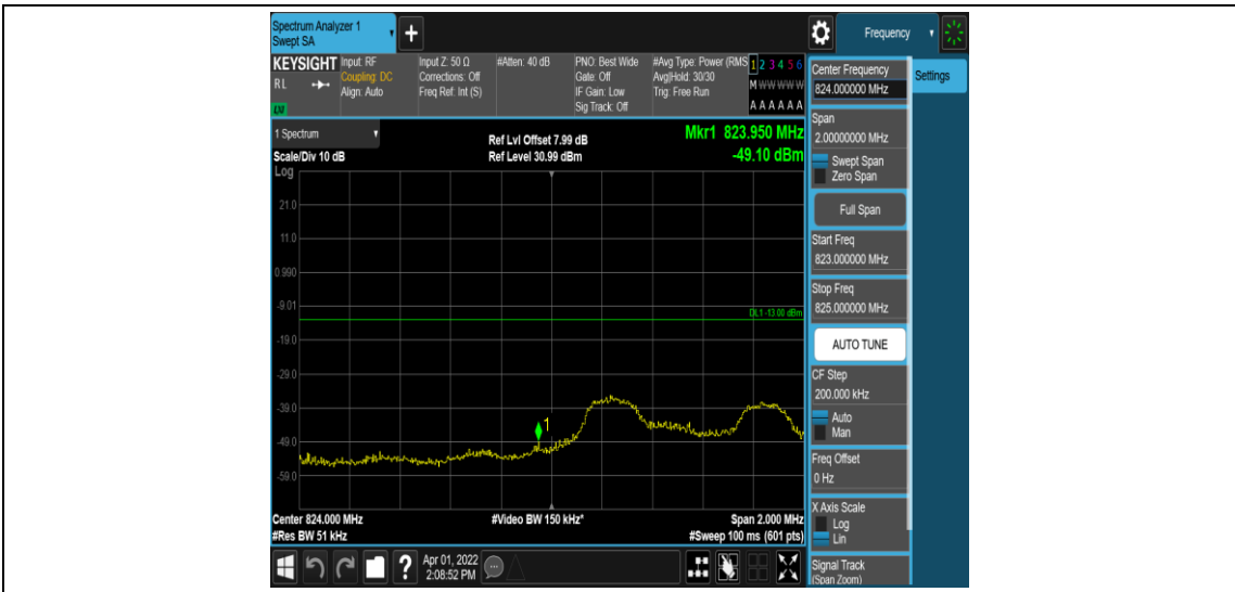
Band26-3MHz-QPSK-26805-1RB#14
