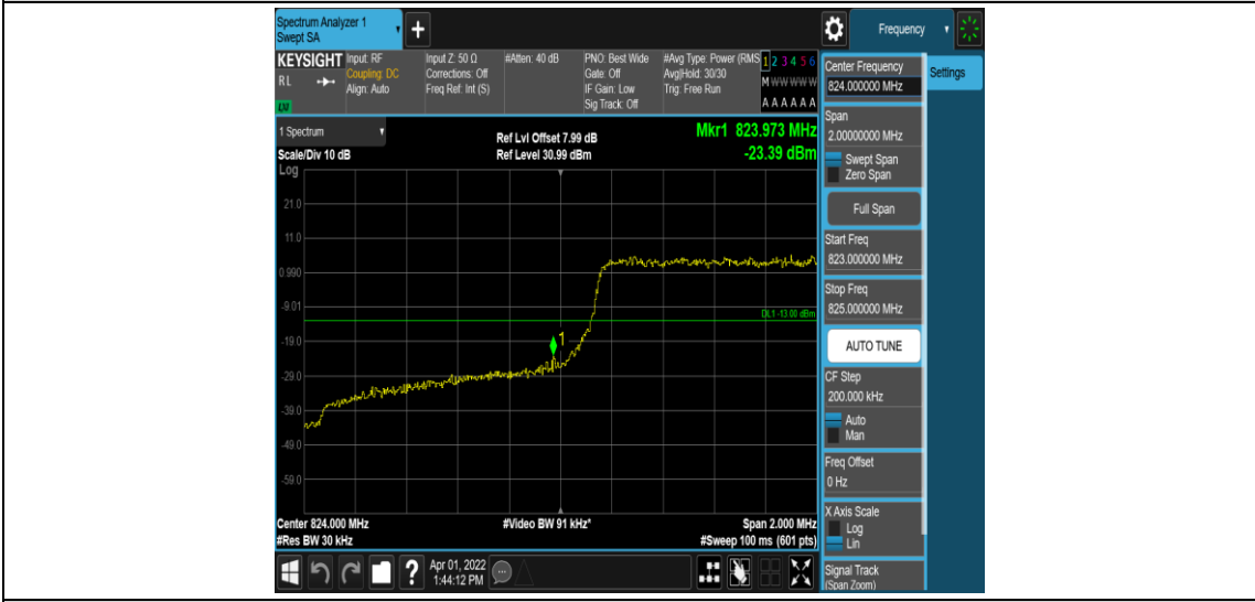
Band26-1.4MHz-QPSK-26797-6RB#0
