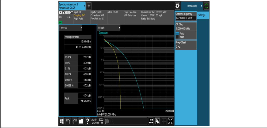
Band26-3MHz-QPSK-27025-15RB#0
