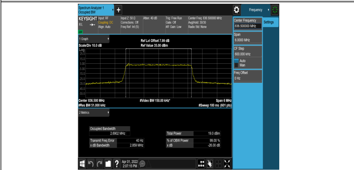
Band26-3MHz-QPSK-26915-15RB#0
