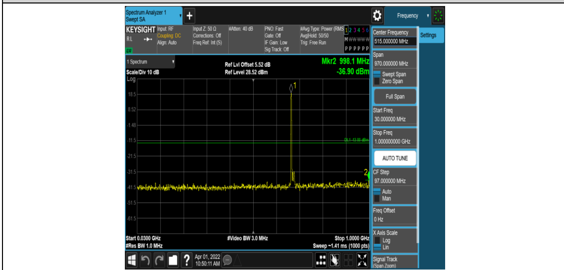
Band71-15MHz-QPSK-133297-1RB#0-Range3:30~1000MHz
