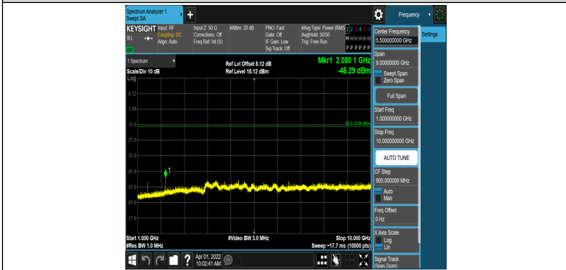
Band71-5MHz-16QAM-133447-1RB#0-Range4:1000~10000MHz
