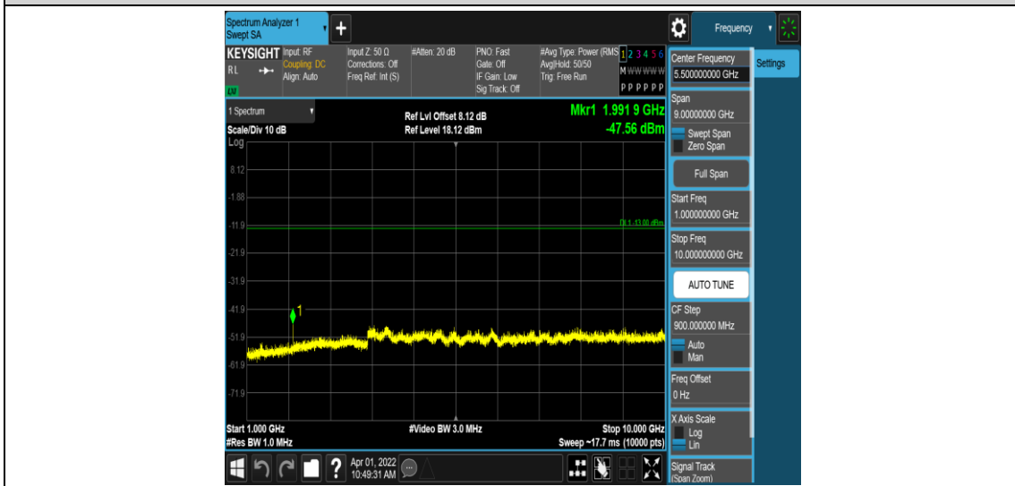
Band71-15MHz-16QAM-133197-1RB#0-Range4:1000~10000MHz
