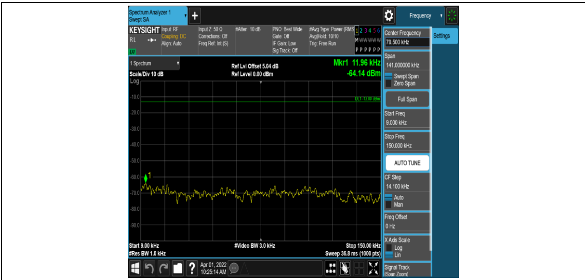
Band71-10MHz-QPSK-133297-1RB#0-Range1:0.009~0.15MHz
